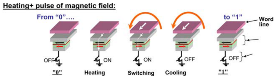
Figure 1.16: Principle of operation the TAS-MRAM where the thermal assistance (Joule heating) is combined with a pulse of magnetic field. Adapted from [74].
