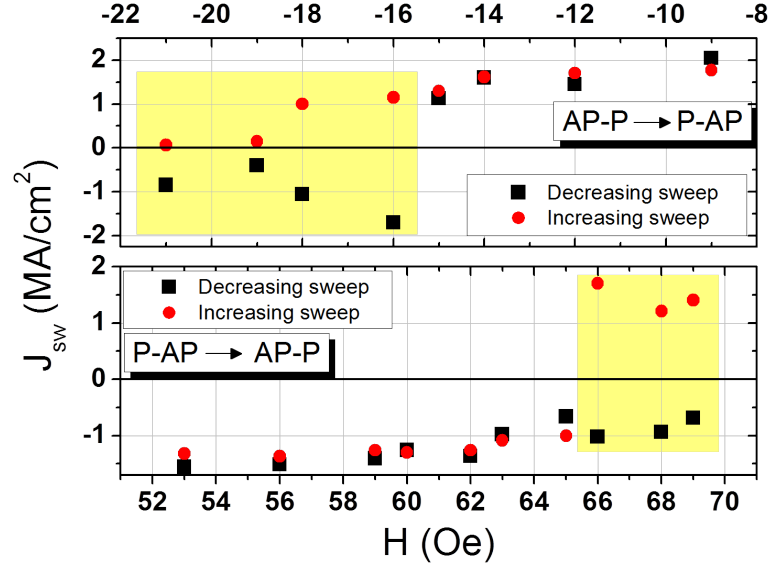
Figure 3.14: Switching current density as a function of the applied field for a junction with thin symmetric barriers and with elliptical cross section (real dimensions 140 nm × 220 nm). The respective R(H) loop is represented in figure 3.3(b). TMR_{write} = 7.1\% , H_c = 47 \text{ Oe} and H_{off} = 25 \text{ Oe} . Decreasing (black squares) and increasing (red circles) sweeps were performed for both transitions. Yellow colored region represents the area where switching happens for both current polarities due to thermal fluctuations and low energy barrier near the coercive fields.
