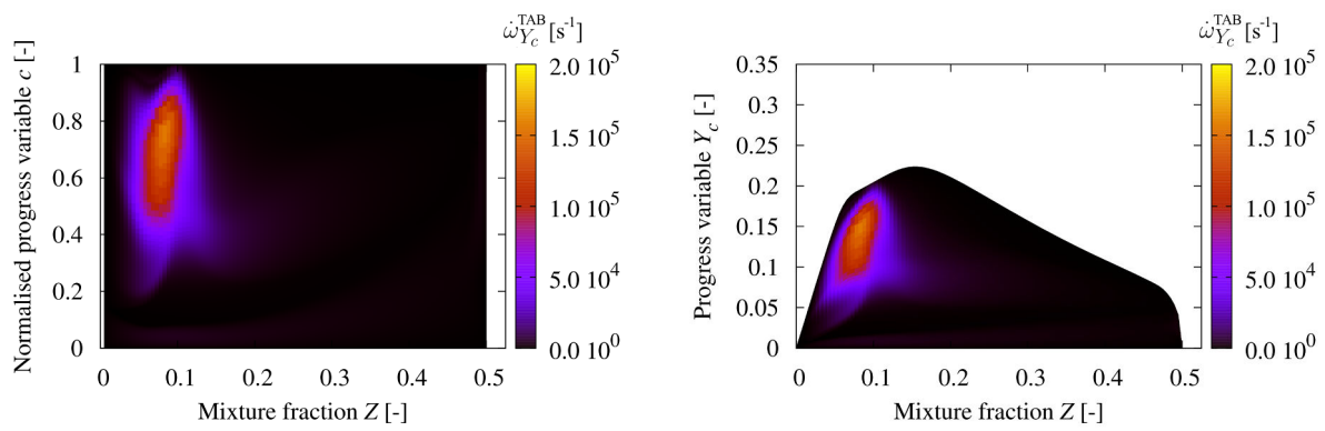
Figure 21: 1-D unsteady strained laminar diffusion flame tabulation of reaction rate of the progress variable \dot{\omega}_{Y_c}^{\text{TAB}} with mixture fraction Z and normalised progress variable c (left), and with mixture fraction Z and progress variable Y_c (right), adapted to single injection case a_0 .
