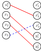
Figure 2.45: Matching \mathcal{M}_9 on \mathcal{N}_4
