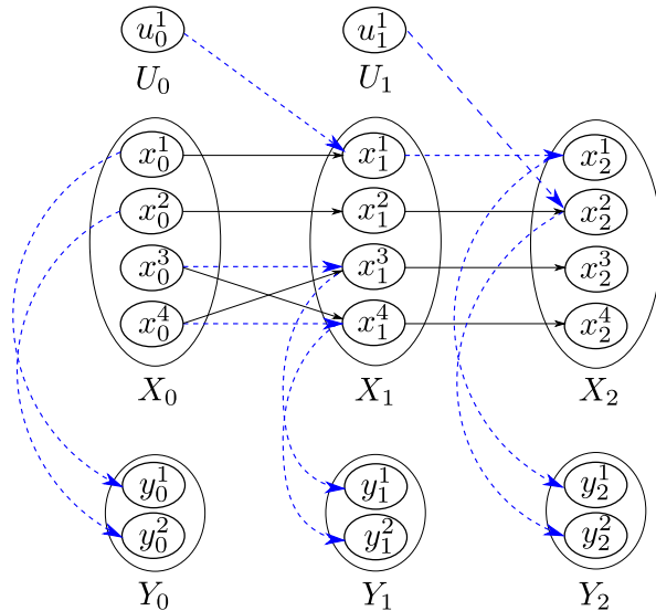
Figure 4.7: In dashed blue, a linking L_{0,2} from X_0 \cup \bar{U} to \bar{Y} on the dynamic graph associated with the example in Figure 4.3
