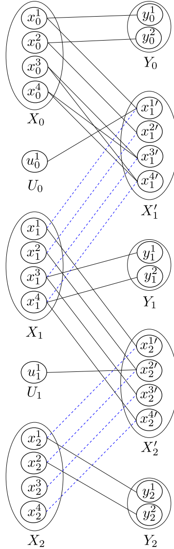
Figure 4.8: Dynamic bipartite graph \mathcal{B}(\mathcal{J}_{0,2}) . The edges in black are one-to-one correspondence with the edges in the dynamic graph in Figure 4.6, while the edges in dashed blue correspond to -I_{4 \times 4} in \mathcal{J}_{0,2}
