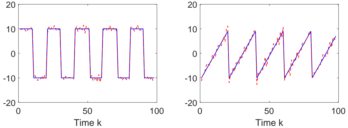
Figure 5.2: Input signals estimation: True signals (blue solid lines) vs estimated signals (red dashed lines)
