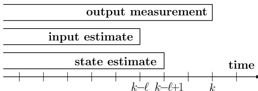
Figure 5.1: Timeline of delay- \ell estimation.
