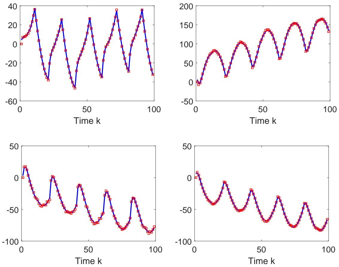
Figure 5.3: State estimation: True states (blue solid lines) vs estimated states (red square lines)
