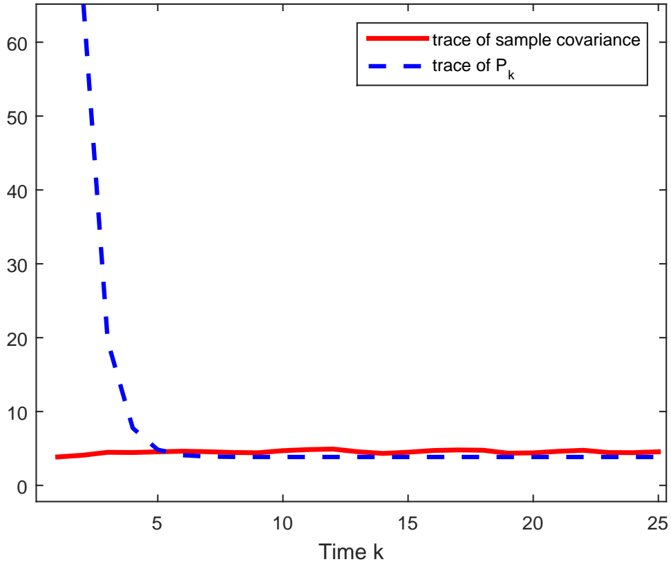
Figure 5.4: In solid red, trace of the sample covariance of the error (u_k^T - \hat{u}_k^T, x_k - \hat{x}_k^T)^T ; in dashed blue trace of the approximate covariance matrix P_k , computed by the algorithm.
