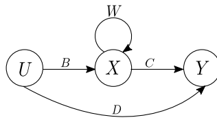
Figure 2.2: Pictorial Reminder of the Construction of \mathcal{G}
