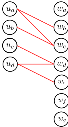
Figure 3.3: Bipartite graph \mathcal{S} associated with \tilde{\mathcal{G}}
