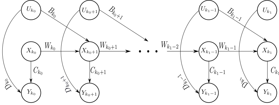
Figure 4.4: Dynamic graph \mathcal{S}_{k_0, k_1}
