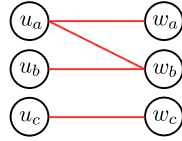
Figure 1.7: Bipartite graph \mathcal{B}
