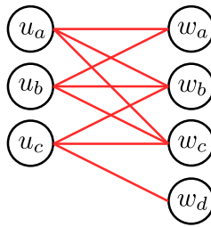
Figure 3.9: Bipartite graph \mathcal{S}_1 associated with \tilde{\mathcal{G}}_1
