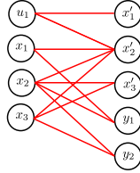
Figure 2.18: Bipartite graph \mathcal{H}_2 associated with \mathcal{G}_2
