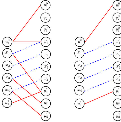
Figure 2.55: Bipartite graph \mathcal{N}_5 Figure 2.56: Matching \mathcal{S} on \mathcal{N}_5
