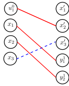
Figure 2.45: Matching \mathcal{M}_9 on \mathcal{N}_4
