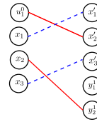
Figure 2.44: Matching \mathcal{M}_8 on \mathcal{N}_4
