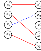
Figure 2.40: Matching \mathcal{M}_4 on \mathcal{N}_4
