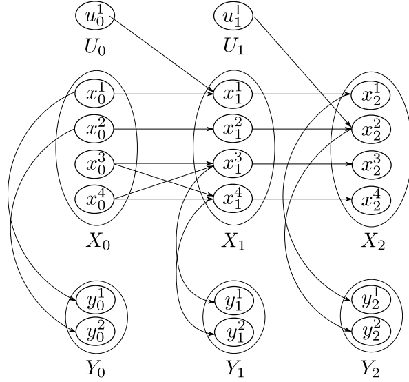
Figure 4.6: Dynamic graph \mathcal{S}_{0,2} associated with the example in Figure 4.3
