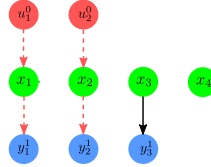
Figure 2.10: Directed graph \mathcal{K}_1 : highlighted in dashed red a linking from U to Y
