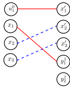
Figure 2.38: Matching \mathcal{M}_2 on \mathcal{N}_4
