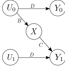
Figure 2.5: Directed graph \mathcal{K}
