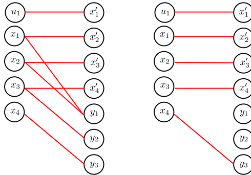
Figure 2.49: Bipartite graph \mathcal{H}_5
