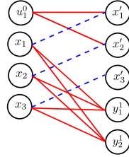
Figure 2.36: \mathcal{N}_4 : the edges in red are in one-to-one correspondence with the edges in \mathcal{G}_4 , while the edges in dashed blue are the newly added ones.
