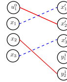
Figure 2.44: Matching \mathcal{M}_8 on \mathcal{N}_4
