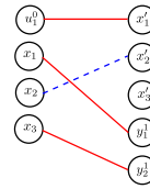
Figure 2.40: Matching \mathcal{M}_4 on \mathcal{N}_4
