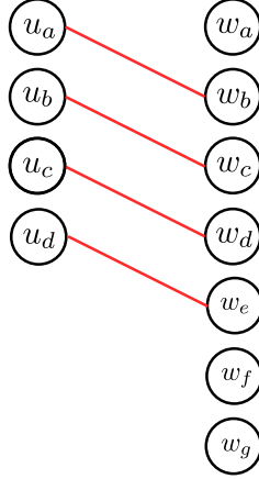
Figure 3.4: A Matching \mathcal{M} in \mathcal{S}
