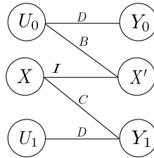
Figure 2.12: Bipartite graph \mathcal{N}
