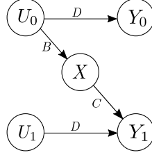
Figure 2.5: Directed graph \mathcal{K}
