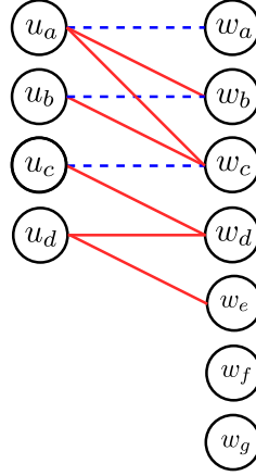
Figure 3.5: Bipartite graph \mathcal{S}_{\times} , in solid red: \mathcal{S}_{\times} \cap \mathcal{S} , in dashed blue: \mathcal{E}_{\text{new}} = \{(u_a, w_a), (u_b, w_b), (u_c, w_c)\} while \mathcal{E}_{\text{loop}} = \{(u_d, w_d)\}
