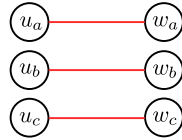
Figure 1.8: A uniquely restricted matching \mathcal{M} on \mathcal{B}
