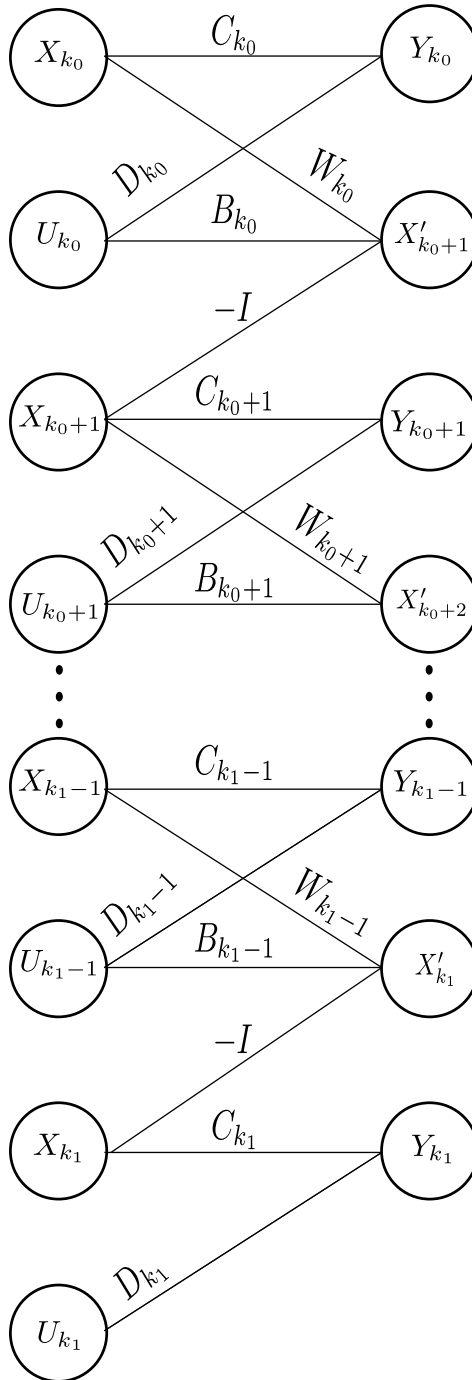
Figure 4.5: Dynamic bipartite graph \mathcal{B}(\mathcal{J}_{k_0, k_1})
