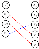
Figure 2.41: Matching \mathcal{M}_5 on \mathcal{N}_4
