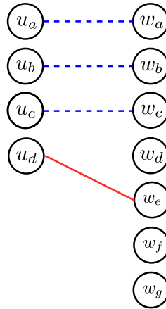
Figure 3.6: A matching \mathcal{M}_{\times} in \mathcal{S}_{\times}
