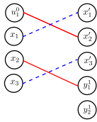
Figure 2.37: Matching \mathcal{M}_1 on \mathcal{N}_4
