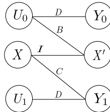
Figure 2.12: Bipartite graph \mathcal{N}
