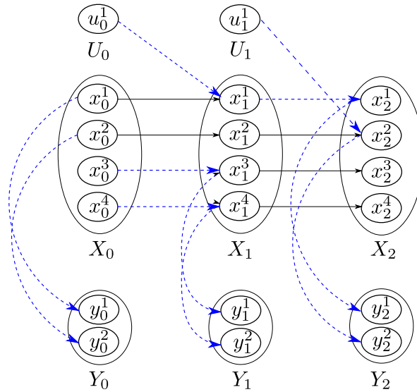
Figure 4.16: In dashed blue, a linking L_{0,2}^1 from X_0 \cup \bar{U} to \bar{Y} on the dynamic graph associated with the example in Figure 4.14
