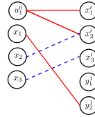
Figure 2.39: Matching \mathcal{M}_3 on \mathcal{N}_4
