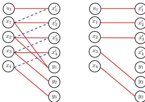
Figure 2.52: Bipartite graph \mathcal{H}_{\times 5}
