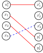
Figure 2.41: Matching \mathcal{M}_5 on \mathcal{N}_4
