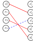
Figure 2.46: Matching \mathcal{M}_{10} on \mathcal{N}_4
