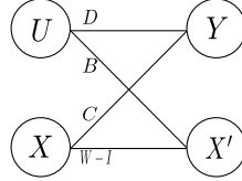
Figure 2.11: Bipartite graph \mathcal{H}_\times
