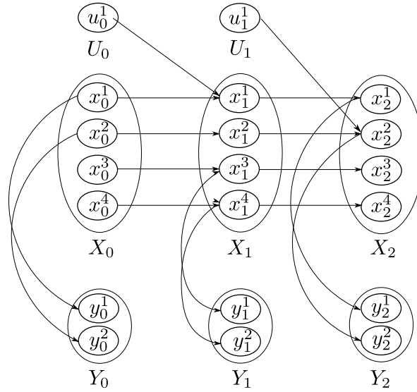
Figure 4.15: Dynamic graph \mathcal{S}_{0,2}^1 associated with the example in Figure 4.14
