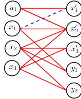
Figure 2.19: Bipartite graph \mathcal{H}_{x_2} ; in dashed blue the newly added self-loop, while the remaining edges are in one-to-one correspondence with those of \mathcal{G}_2
