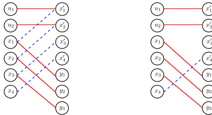
Figure 2.14: Bipartite graph \mathcal{N}_1 Figure 2.15: Matching \mathcal{M}^{\mathcal{N}} , of size 6, on \mathcal{N}_1
