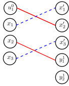
Figure 2.37: Matching \mathcal{M}_1 on \mathcal{N}_4
