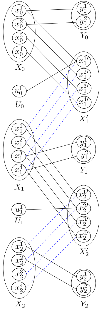
Figure 4.17: Dynamic bipartite graph \mathcal{B}^1(\mathcal{J}_{0,2}^1) . The edges in black are one-to-one correspondence with the edges in the dynamic graph in Figure 4.6, while the edges in dashed blue correspond to -I_{4 \times 4} in \mathcal{J}_{0,2}^1 .
