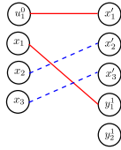
Figure 2.38: Matching \mathcal{M}_2 on \mathcal{N}_4
