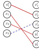
Figure 2.46: Matching \mathcal{M}_{10} on \mathcal{N}_4
