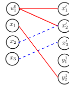
Figure 2.39: Matching \mathcal{M}_3 on \mathcal{N}_4
