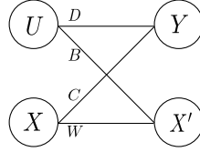
Figure 2.3: Bipartite graph \mathcal{H} associated with a structured system
