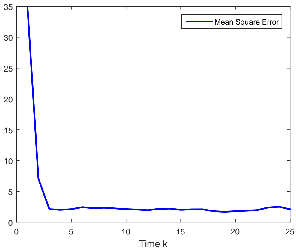
Figure 5.6: Plot of mean square error in the estimation.
