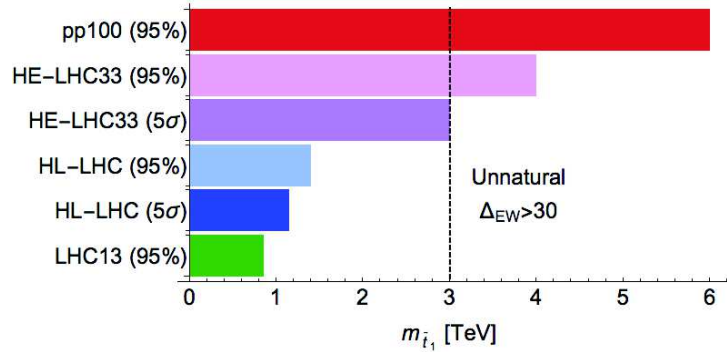
Figure 5.19: Potential of discovery ( 5\sigma ) and exclusion (95%) of the stop \tilde{t}_1 mass for the past LHC searches with an integrated luminosity \int \mathcal{L} \sim 13 \text{ fb}^{-1} and a center-of-mass energy \sqrt{s} of 13 TeV, HL-LHC with \sqrt{s} = 13 \text{ TeV} and \int \mathcal{L} = 3000 \text{ fb}^{-1} , HE-LHC with \sqrt{s} = 33 \text{ TeV} and \int \mathcal{L} = 3000 \text{ fb}^{-1} , and a pp collider (FCC) with \sqrt{s} = 100 \text{ TeV} and \int \mathcal{L} = 3000 \text{ fb}^{-1} [116].
