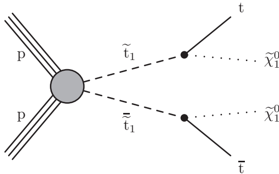
Figure 4.6: An example of diagram of direct stop pair production. In this diagram both stops decay to a top quark and a neutralino.
