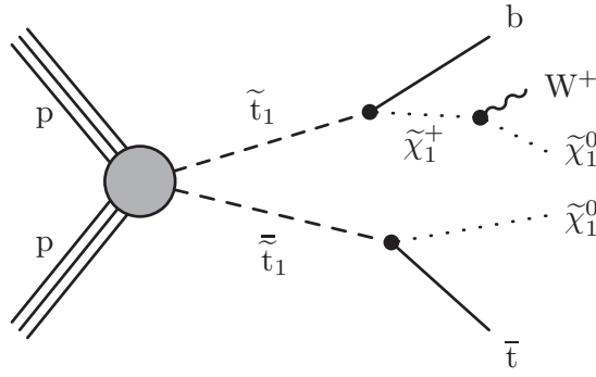
Figure 5.3: The SMS diagram for the direct stop pair production considering the mixed decay of the stop pair \tilde{t}_1\tilde{t}_1^0 b\tilde{\chi}_1^+ \tilde{\chi}_1^0 [134].
