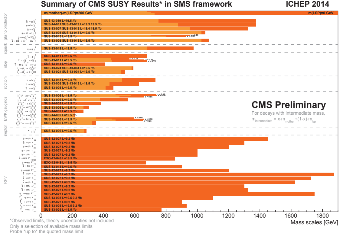
Figure 4.10: Summary of the masses of SUSY particles excluded by the CMS collaboration [123]. The limits in darker shades are given for a massless LSP, while lighter shades limits are for m(\text{mother})-m(\text{LSP})=200 GeV. More details can be seen in the documentation of the analyses.
