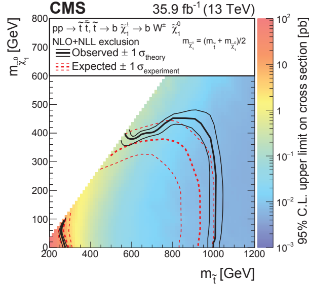
Figure 5.17: The exclusion limits at 95% CL on the T2bW model corresponding to an integrated luminosity of 35.9 \text{ fb}^{-1} [128]. The interpretation is provided in the context of the SMS, in the plane of the stop mass vs LSP mass. The color code shows the 95% CL upper limit on the cross section. The red and black contours represent the expected and observed exclusion limits, respectively. The area below the black thick curve indicates the excluded region of the signal points.
