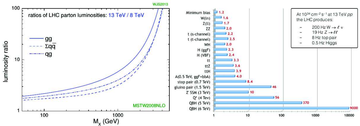
Figure 4.11: (left) The ratios of 13 TeV to 8 TeV LHC parton luminosities as a function of a produced particle mass M_X . (right) The value of this ratio for several SM and beyond SM processes [127].
