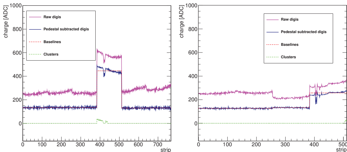
Figure 2.33: Examples of data from one tracker module undergoing zero suppression and clustering. The raw digis are shown in pink. From the raw digis, the pedestals are subtracted and the resulting digis are shown in blue. The baselines shown in red are computed and subtracted from pedestal subtracted digis. The final clusters are shown in green. (left) The fourth APV has a \sigma_{raw} of 14 ADC and a baseline value of 446 ADC. (right) The fourth APV has a \sigma_{raw} of 21 ADC and a baseline value of 257 ADC.
