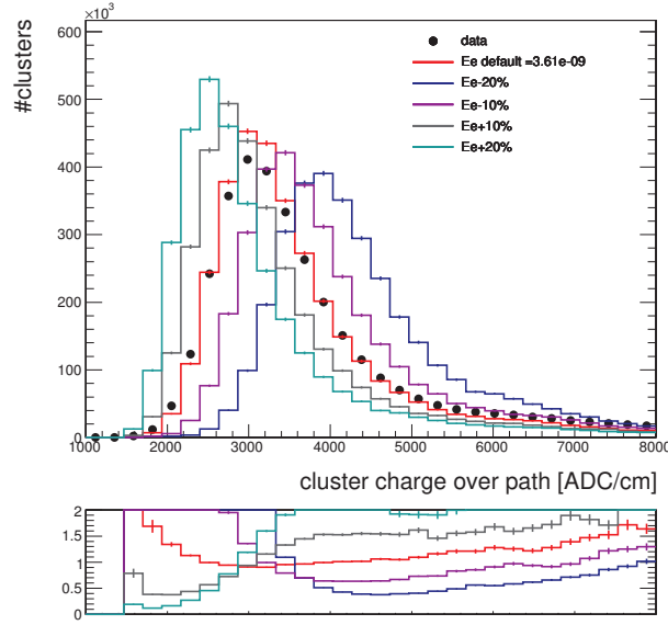
Figure 3.24: Data and simulation comparison of the on-track cluster charge divided by the track length for the OB2 geometry and different values of the energy to electrons conversion factor E_e . The simulated distributions are rescaled to the number of clusters in data. The bottom plot represents the data to simulation ratios.
