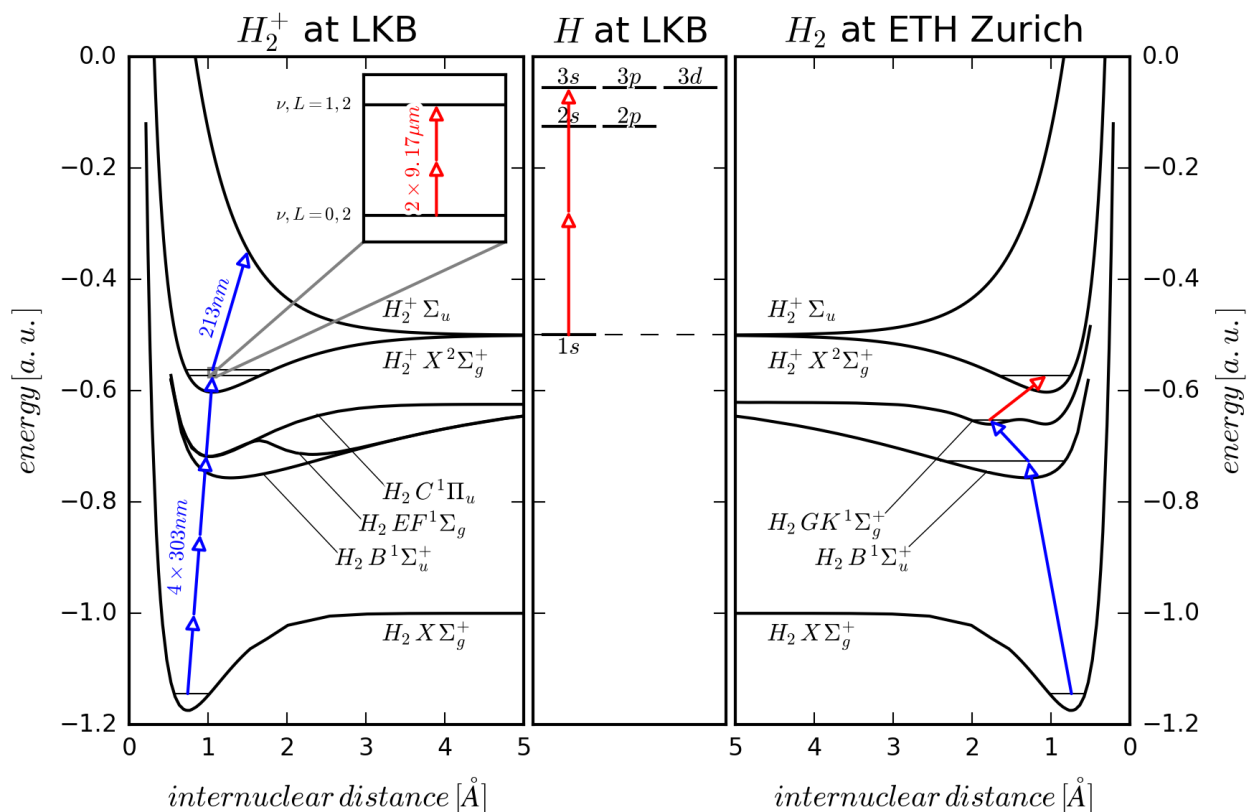
Figure 1.1: Left: Electronic states in the Born-Oppenheimer approximation for \text{H}_2 and \text{H}_2^+ and transitions as planned at LKB. The arrows show the vibrational ground state preparation of \text{H}_2^+ using a 3 + 1 REMPI scheme at 303 nm, and after that the 2 + 1 REMPLD spectroscopy. The inset shows the two-photon transition at 9.17 \mu\text{m} between two ro-vibrational levels. Center: The energy structure of the \text{H} atom and the transition currently probed at one of the groups at LKB. Right: Rydberg state spectroscopy of \text{H}_2 as performed at the ETH Zürich.
