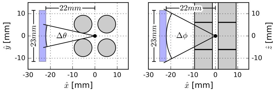
Figure 2.30: Sketch of the position of the lens (indicated on the left side) relatively to the trap. The electrode diameter limits the angle \theta .
