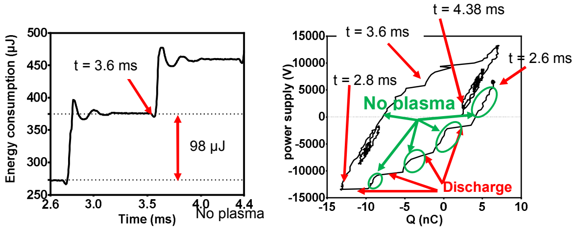
Fig 119 Left: Detail of the integral of the power as a function of time. The decrease in the energy consumed just after 2.7 ms, as well as the overshoot between 2.8 and 2.9 ms is due to the transient capacitive currents (this is energy stored in capacitive form and then released). Right: XY representations of signals between t=2.6 ms and t=4.38 ms.
