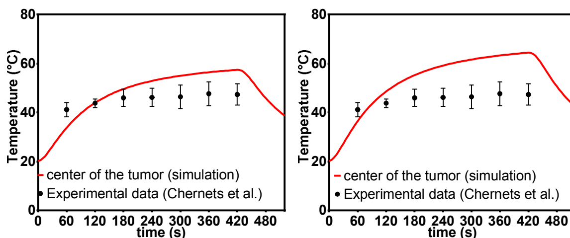
Fig 279 Temperature in the center of the tumor as a function of time for q_{plasma} = 5000 \text{ W/m}^2 (left) and q_{plasma} = 6000 \text{ W/m}^2 with \lambda_{tumor} = 0.2 \text{ W} \cdot \text{m}^{-1} \cdot \text{K}^{-1} .
