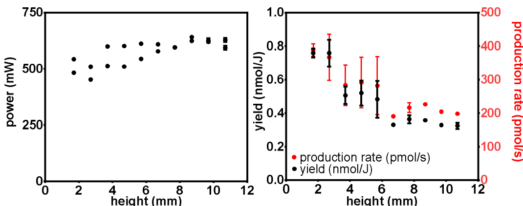
Fig 93 Left: power (mW) as a function of height. Right: yield (nmol/J) and production rate (pmol/s) of \text{HO}^\circ as a function of height. Treatment time = 3 min, frequency of power supply = 500 Hz, peak to peak voltage = 28.1 kV, \Phi_{He} = 500 \text{ sscm} , height = 1.5-10.5 mm, power supply = “500 Hz generator n°3” (II.2.1, Power supply). Each well of the 24-well plate (flat bottom) contains 1400 \mu\text{L} of the TPA +KOH solution. Duplicate.
