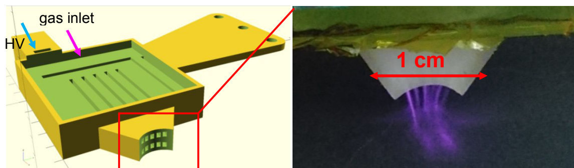
Fig 19 Left , view of a multi-channel plasma jet. The gas circulates in five rectangular channels ( 1.5 \times 3 \text{ mm} ). The high voltage electrode is placed 1.4 mm above these channels. The polymerized resin 1060ES7 made the dielectric layer and gas sealing. At the position of the nozzle each, channel is divided in two. The ten channels are distributed over a length of about 1 cm. Right , view of the nozzle facing a black paper stuck on the electrical ground.
