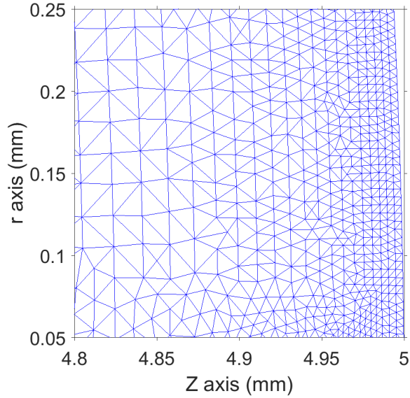
Fig 166 Triangulations applied to the outermost layers of mouse skin. For epidermis and dermis, the size of each triangle is below the size of the cell itself (order of magnitude d \sim 10 \mu\text{m} ). The mesh enables to describe temperature and damage field in a precise manner. At this spatial resolution, it is not the resolution of the simulation that is lacking, but the physical model which ceases to be valid. It doesn't make sense to perform calculations of the field of temperature at the subcellular or cellular scale because the medium is far from being isotropic and homogeneous.
