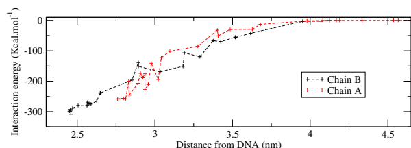
Figure 5.41: MgFur + Fur box simulation
