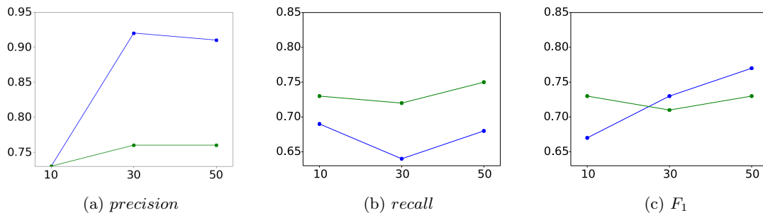
Figure 4.10: Freiburg N_{CY} Results . Scores in function of N_{CY} . Blue indicates the single-scale system, green indicates the multi-scale. The accuracy scores fell between 0.81 and 0.87.
