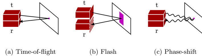
Figure 2.1: Lidar Methods . The methods are illustrated in a schematic way. t indicates the transmitter, r the receiver. The different laser patterns are shown through the violet forms on the target surface. 2.1b shows the array of detectors of the receiver. 2.1c emphasizes how the signal is processed based on the laser wave phase.
