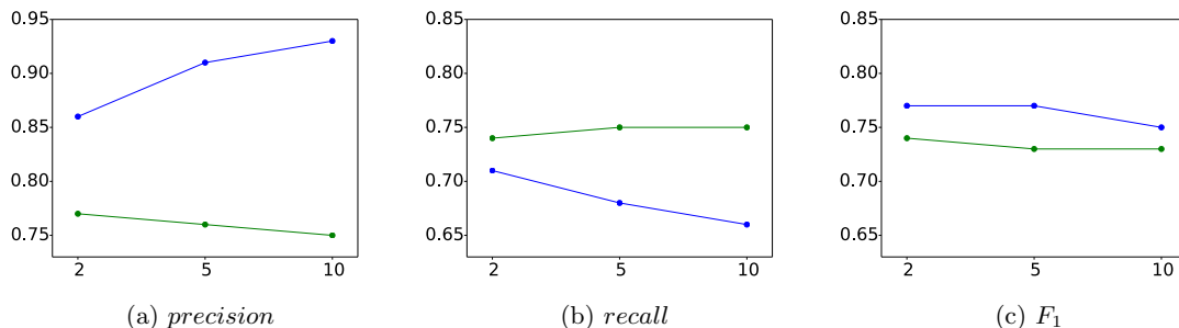
Figure 4.6: Freiburg Learning Curves . The plots show the scores in function of the number of scans in the training set. The scores are the total precision, recall and F_1 . The total F_1 is the average of the classwise F_1 scores, so the precision and recall shown are not directly used in the computation, but rather indicators of the global trend across the classes. Blue indicates the single-scale results, green indicates the multi-scale results. The accuracy scores fell between 0.83 and 0.87.
