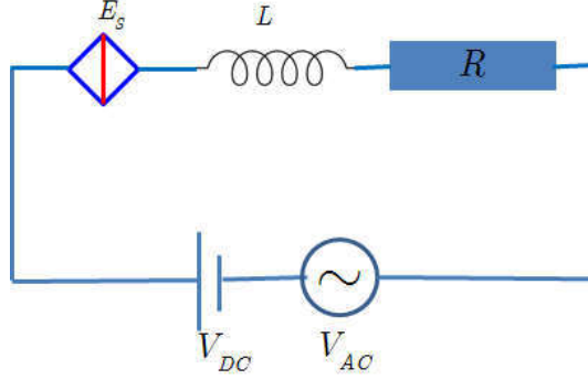
Figure 1.10: Voltage-biased phase-slip junction.
