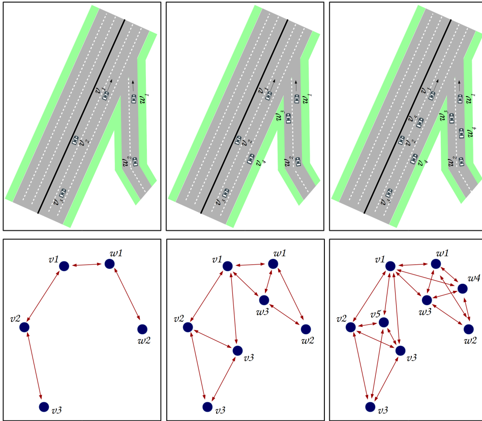
Figure 4.6 – A highway junction and related communication graphs
