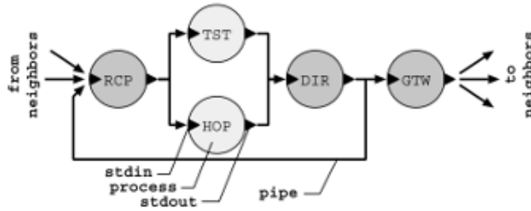
Figure B.2 – Communicating architecture of EMU
