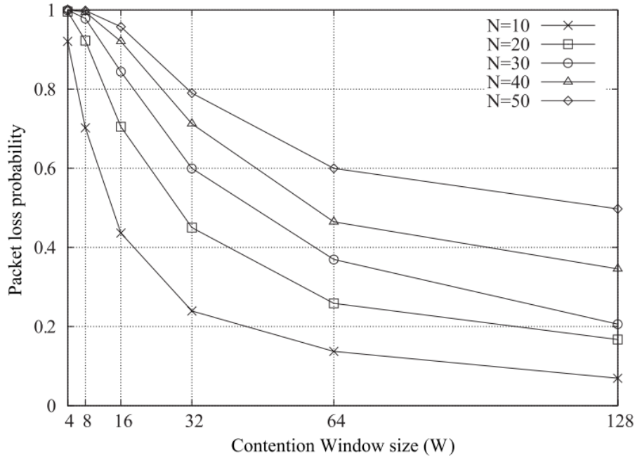
Figure 3.1 – Packet loss probability from [Campolo and Vinel, 2011]
