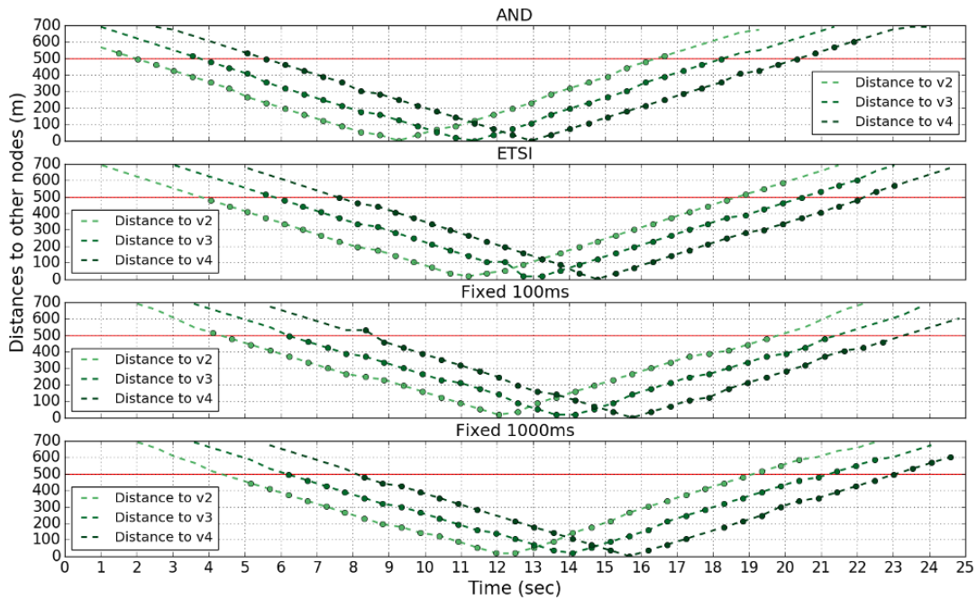
Figure 3.6 – Distances of discovery obtained by each considered algorithm and a variable packet loss rate. v_1 is the ego-node.
