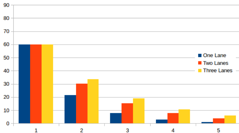
Figure 4.5 – Trust computed on Node a for nodes at 1 to 5 hops. Using \beta = 0.8
