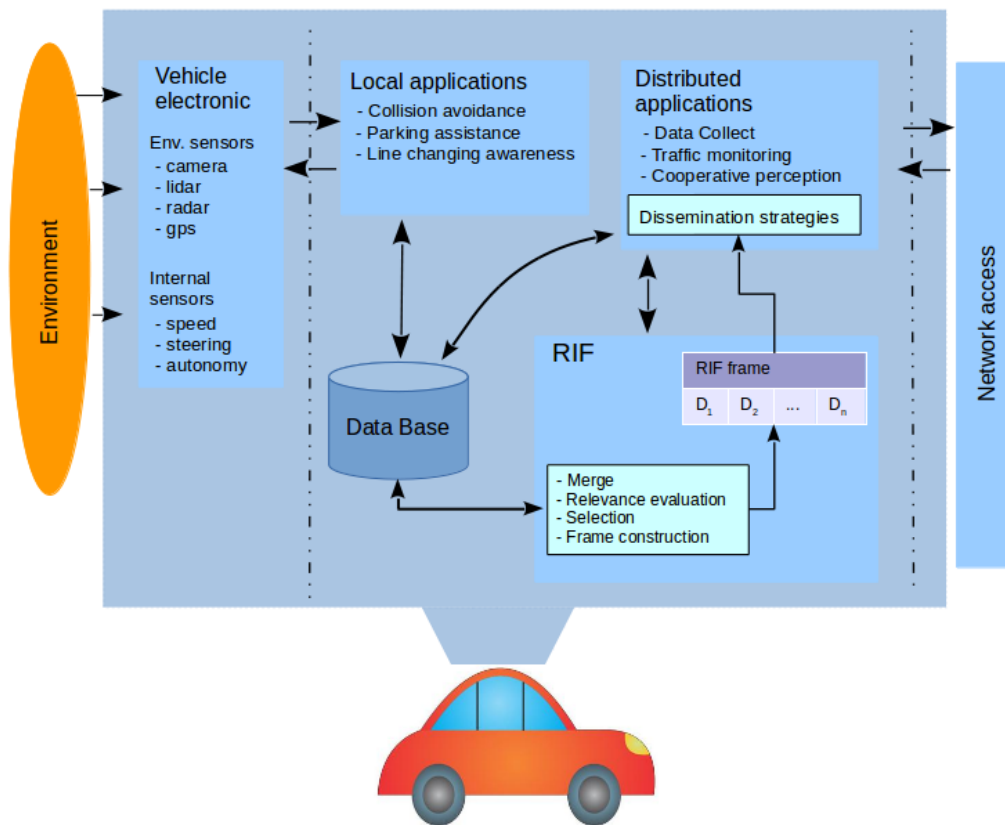
Figure 5.1 – High level view of RIF architecture for a VANET node
