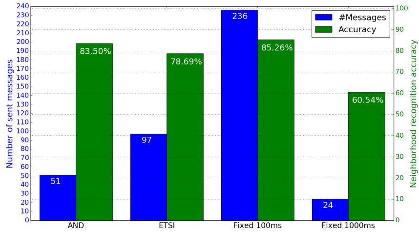
Figure 3.9 – Overall experiment results obtained by each considered algorithm in a network with 70% of loss rate
