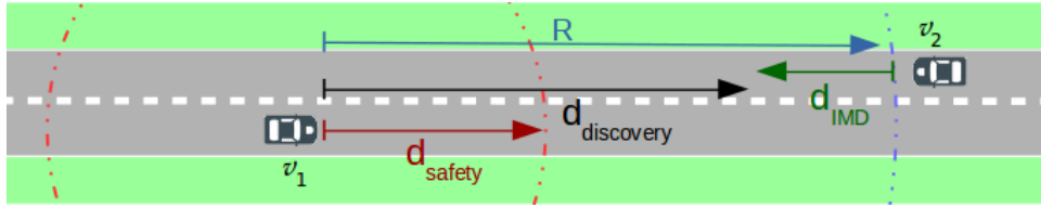
Figure 3.3 – Scenario considered for the analytical study of vehicles identification - Vehicles moving towards one another.
