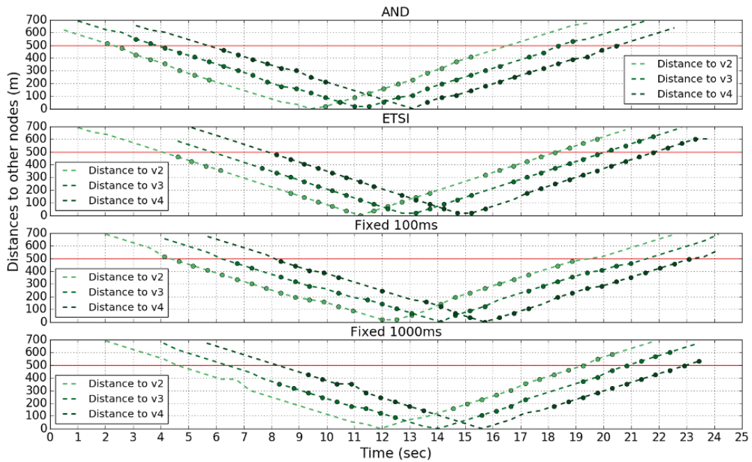
Figure 3.5 – Distances of discovery obtained by each considered algorithm and a packet loss rate of 70%. v1 is the ego-node.
