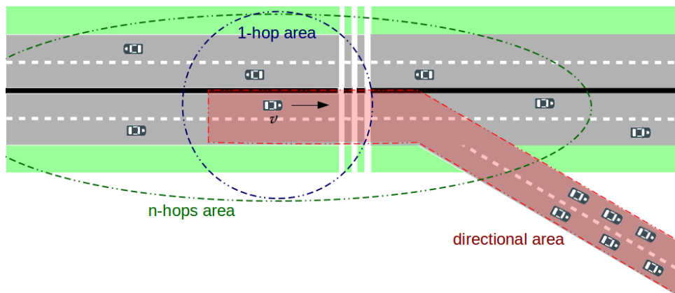
Figure 2.2 – Areas of interest for an ego-vehicle v
