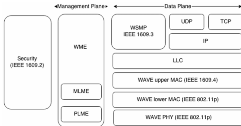
Figure 1.1 – WAVE architecture [Vivek et al., 2017]
