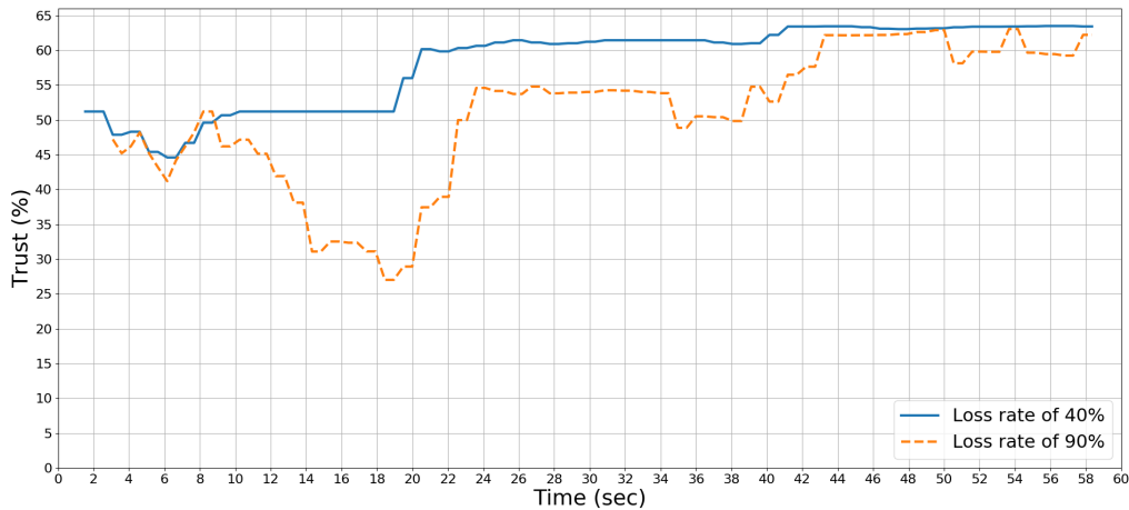
Figure 4.9 – Trust variation of Node w_2 in other nodes when applying the smoothing mechanism
