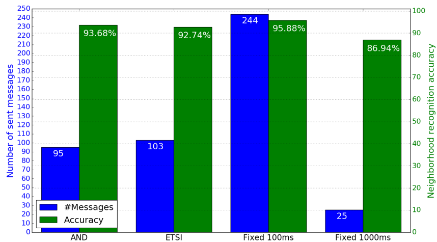
Figure 3.10 – Overall experiment results obtained by each considered algorithm in a network with a variable loss rate
