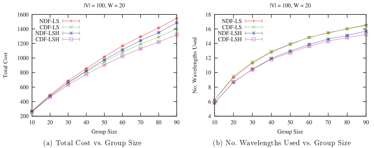
Figure 5.24 – Performances of algorithms on 100-node random graphs with W = 20
