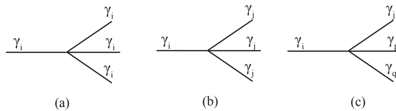
Figure 1.11 – Three MC-OXC models in a WDM multicast network: (a) MSW. (b) MSDW. (c) MAW. [8]
