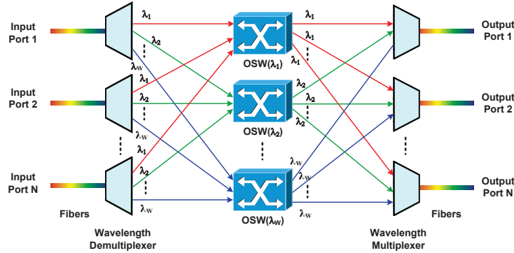
Figure 1.3 – A general optical cross-connect architecture [2]
