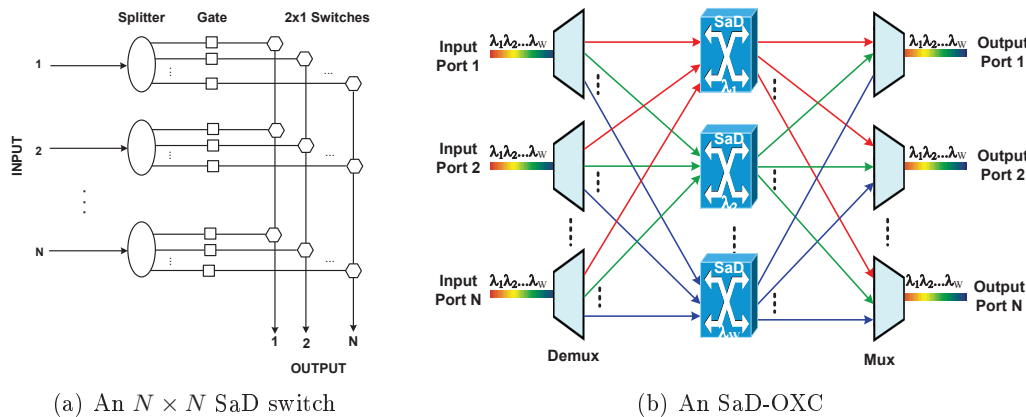
Figure 1.4 – An N \times N SaD-OXC architecture [3]
