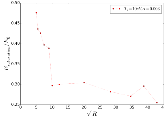
Figure 2.10 – The saturation energy of the bulk electrons at t = 1250 in units of the total energy for \alpha = 0.003 and for the temperature T_b = 10\text{eV} for the electron beam. The temperature of the bulk electrons is T_e = 0.1\text{eV}
