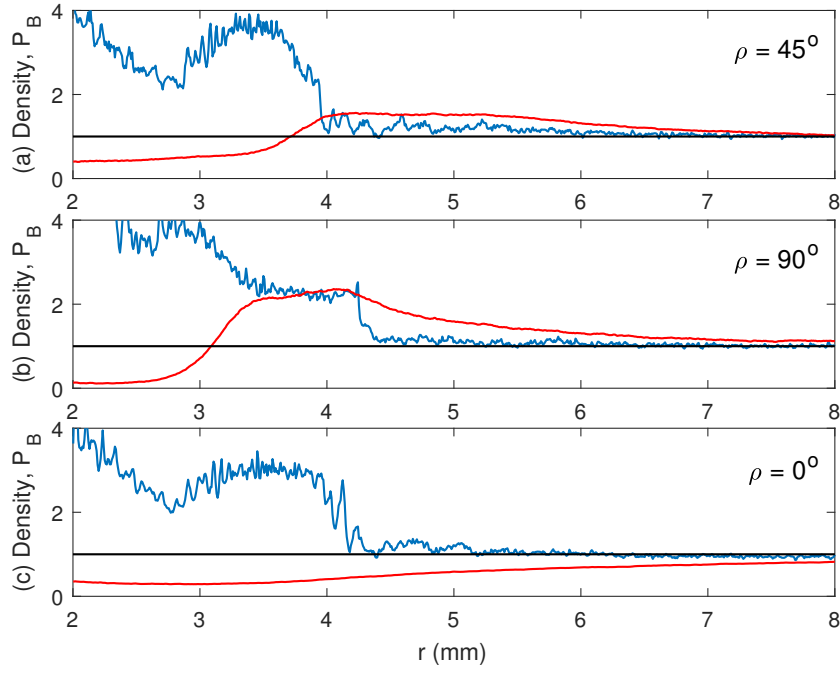
Figure 4.20 – Radial profiles of the ion density (blue) and the magnetic pressure P_B (red): (a) along the direction 45^\circ , (b) along the direction 90^\circ and (c) along \rho = 0 . Both distributions have been averaged over an angular interval with the width 0.5^\circ . The time is t_{sim} = 3.57 ns.
