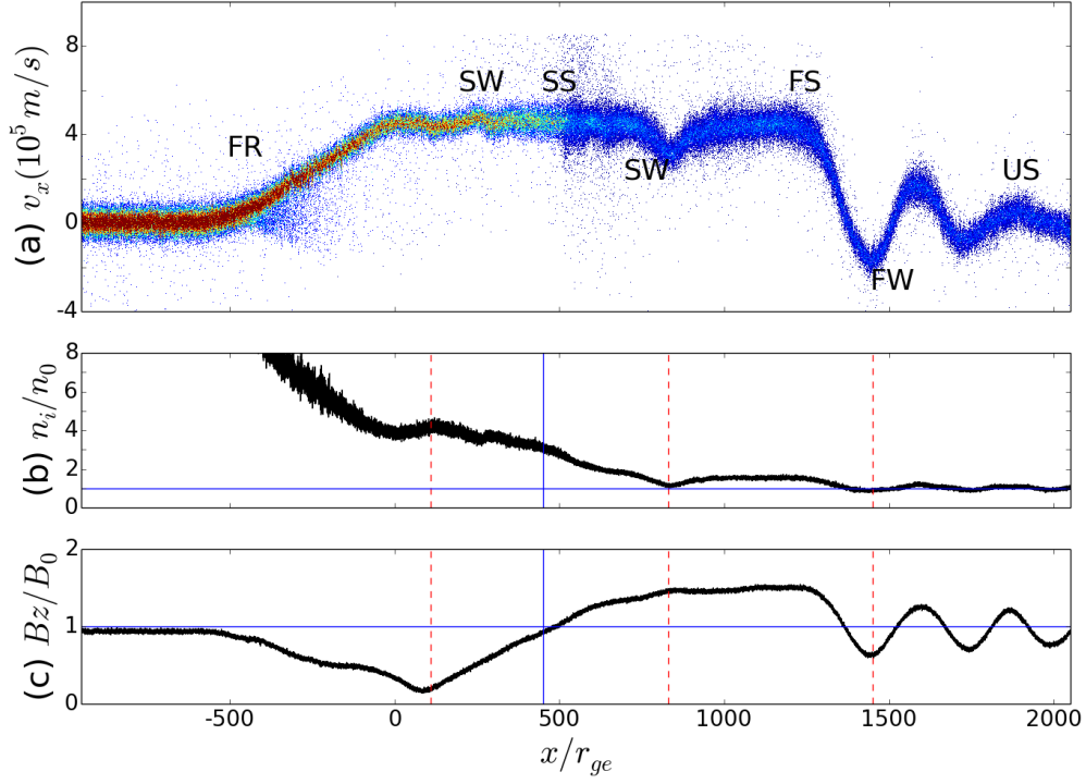
Figure 4.13 – The plasma state at the time t\omega_{ce} = 2 \times 10^4 : panel (a) shows the phase space density distribution of the ions normalized to the maximum upstream value and clamped at 2.9 for visualization reasons. We recognize the fast rarefaction wave (FR), the slow shock (SS), the fast shock (FS), the fast wave (FW) precursor and the upstream (US) ions. We observe a slow wave (SW) precursor close to the slow shock. Panel (b) shows the ion density n_i/n_0 . The blue lines denote n_i = n_0 and x/r_{ge} = 450 . The magnetic B_z component is plotted in (c). The blue line denotes B_z = B_0 and x/r_{ge} = 450 . The dashed red lines in (b,c) emphasize the phase relation between n_i and B_z and, thus, the wave mode. The obliquity is \theta = 70^\circ .
