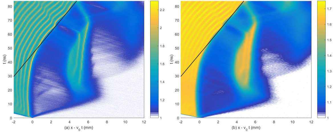
Figure 4.30 – The proton density distribution n_i(\hat{x}, t)/n_0 is shown as a function of space and time in panel (a) and that of the magnetic B_z(\hat{x}, t)/B_0 component in panel (b). Both distributions are sampled in the reference frame \hat{x} = x - v_0 t with v_0 = 1.25 \times 10^6 m/s. The overplotted line has the slope v_0/10 .
