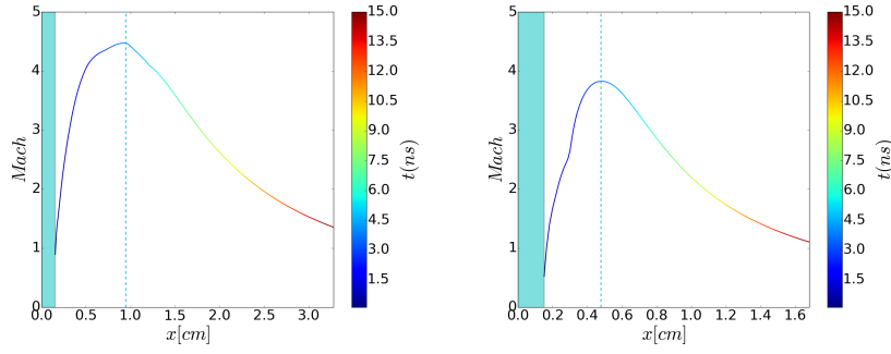
Figure 6.8 – Evolution of the magnetosonic Mach number M_{ms} of the edge of the plasma plume versus time (color) and space (x axis) in the LMJ (left) and LULI2000 (right) case.
