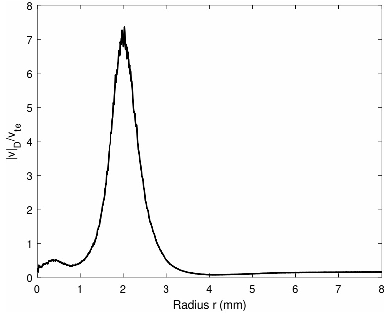
Figure 4.24 – The magnitude of the azimuthally averaged drift speed |v_D|/v_{Te} at the time t_{sim} = 3.57 ns.
