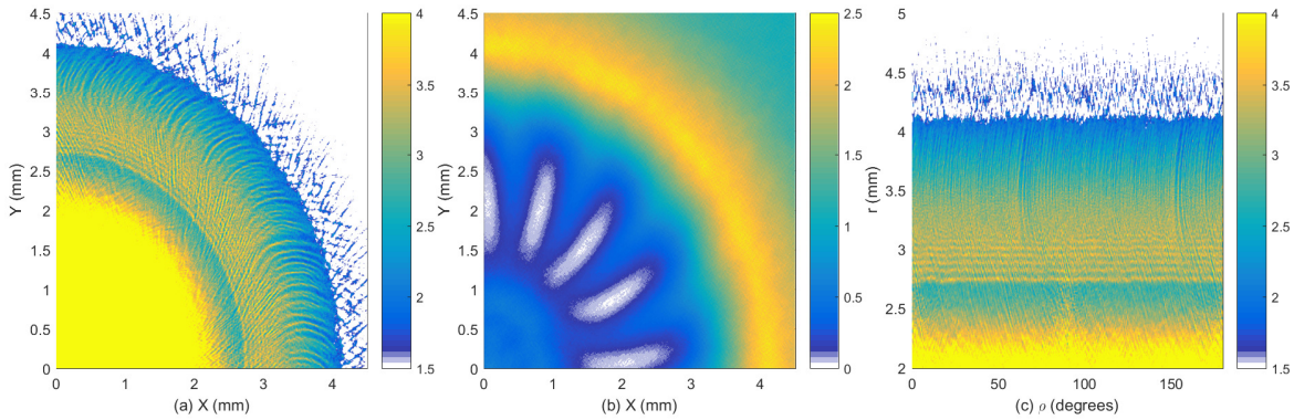
Figure 4.21 – The distribution of the ion density n_i and of the normalized magnetic pressure P_B = (B_x^2 + B_y^2 + B_z^2)/B_0^2 . The ion density is shown in cartesian coordinates in (a). Panel (b) shows the magnetic pressure in cartesian coordinates. The ion density distribution in polar coordinates is shown in panel (c). The linear color scale is clamped to the value 1.5 in (a, c) in order to emphasize the location of the shock. The time is t_{sim} = 3.57 ns.
