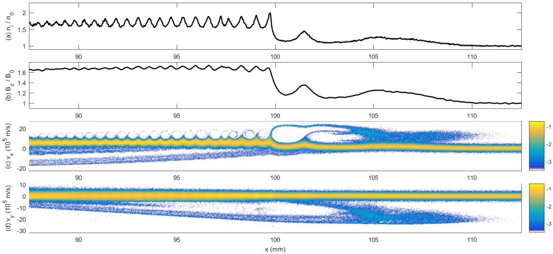
Figure 4.34 – The plasma state at 76 ns: panel (a) shows the proton density n_i/n_0 . The magnetic B_z/B_0 component is plotted in panel (b). Panels (c, d) show the phase space density distributions (x, v_x) and (x, v_y) of the protons. The latter are normalized to their maximum values and displayed on a 10-logarithmic scale.
