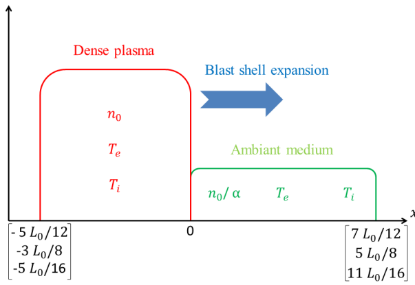
Figure 3.2 – Sketch of the plasma density distribution in the simulation box. The localisation of the boundaries of the simulation box change regarding to \alpha .
