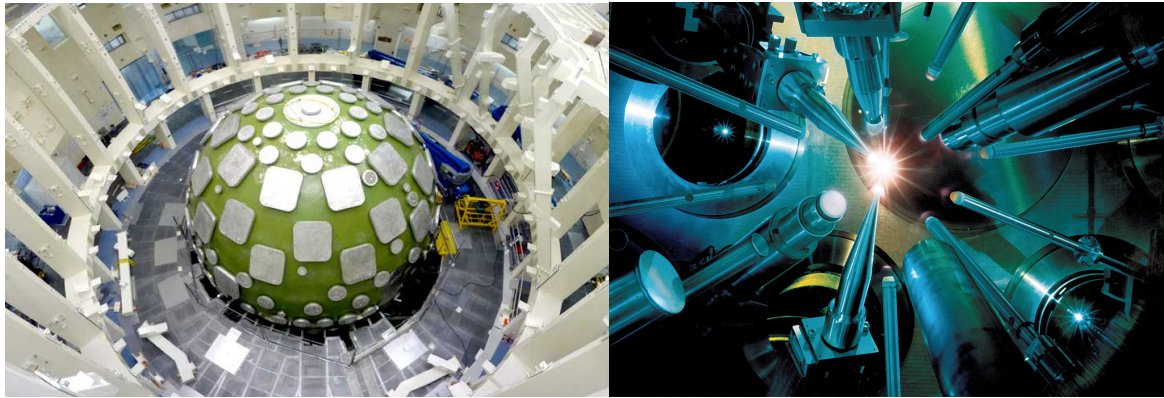
Figure 5 – Experimental sphere of the LMJ facility (left), and artist representation of laboratory astrophysics experiments (right). By mimicking fundamental physics aspects in the lab, researchers hope to better understand violent cosmic phenomena.
