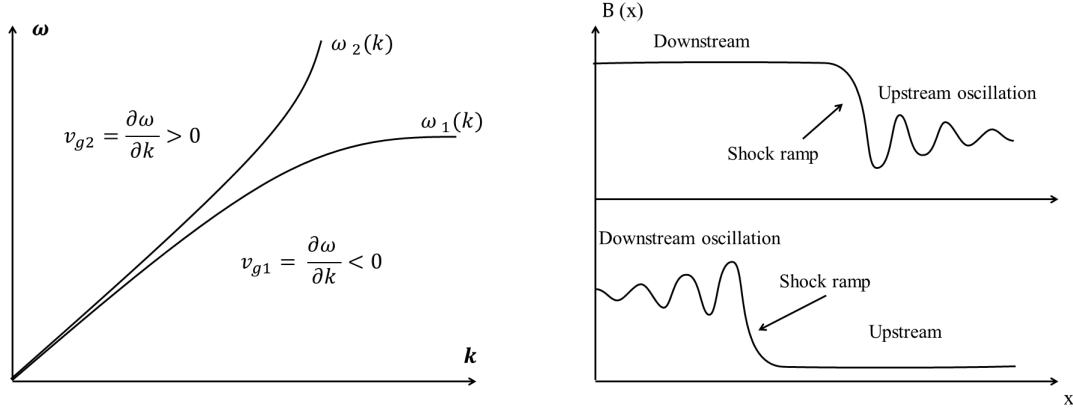
Figure 4.2 – Two different types of dispersions in the (\omega_r, \mathbf{k}) -plane. (left) The short waves with concave dispersion relation, \omega_1 , have a smaller group velocity than long waves and form a trail on the long wave. For a convex dispersion relation, \omega_2 , the short waves move faster than long waves. The effect of this difference in sideband wave velocity on a laminar subcritical shock wave are shown in the right panel. The waves, spatially damped, moving-away from the shock ramp into the downstream region, are produced by a concave dispersion relation (down right). These waves occur in the upstream region for a convex dispersion relation (up right).
