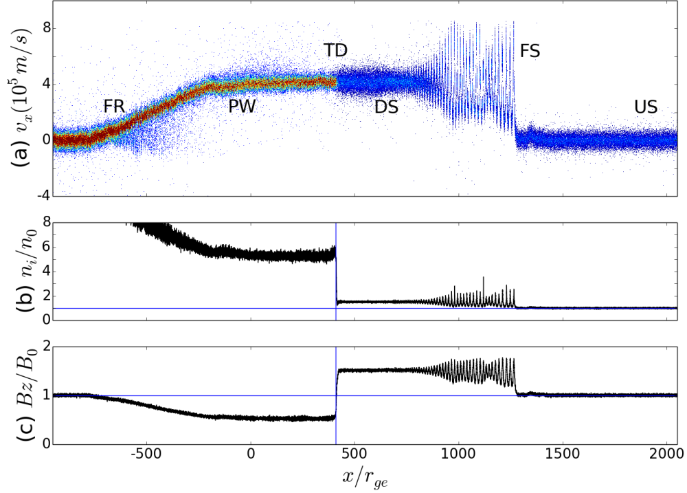
Figure 4.5 – The plasma state at the time t\omega_{ce} = 2 \times 10^4 : panel (a) shows the phase space density distribution of the ions normalized to the maximum upstream value and clamped at 2.9 for visualization reasons. We recognize the fast rarefaction wave (FR), the precursor wave (PW), the tangential discontinuity (TD), the fast shock (FS), and the upstream/downstream (US/DS) ions. Panel (b) shows the ion density n_i/n_0 . The blue lines denote n_i = n_0 and x/r_{ge} = 410 . The magnetic B_z component is plotted in (c). The blue line denotes B_z = B_0 and x/r_{ge} = 450 . The obliquity is \theta = 90^\circ .
