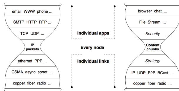
Figure 1.5: Communication layer: similarities and differences between IP and NDN. Picture from [JSB + 09].
