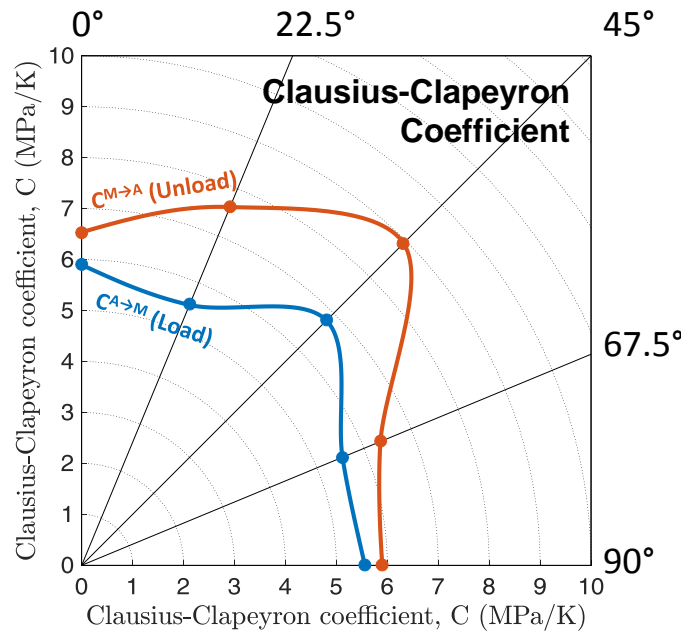
Figure 3.11: Clausius-Clapeyron coefficients for forward ( C^{A \rightarrow M} ) and reverse ( C^{M \rightarrow A} ) transformations at f_m = 0.5 .
