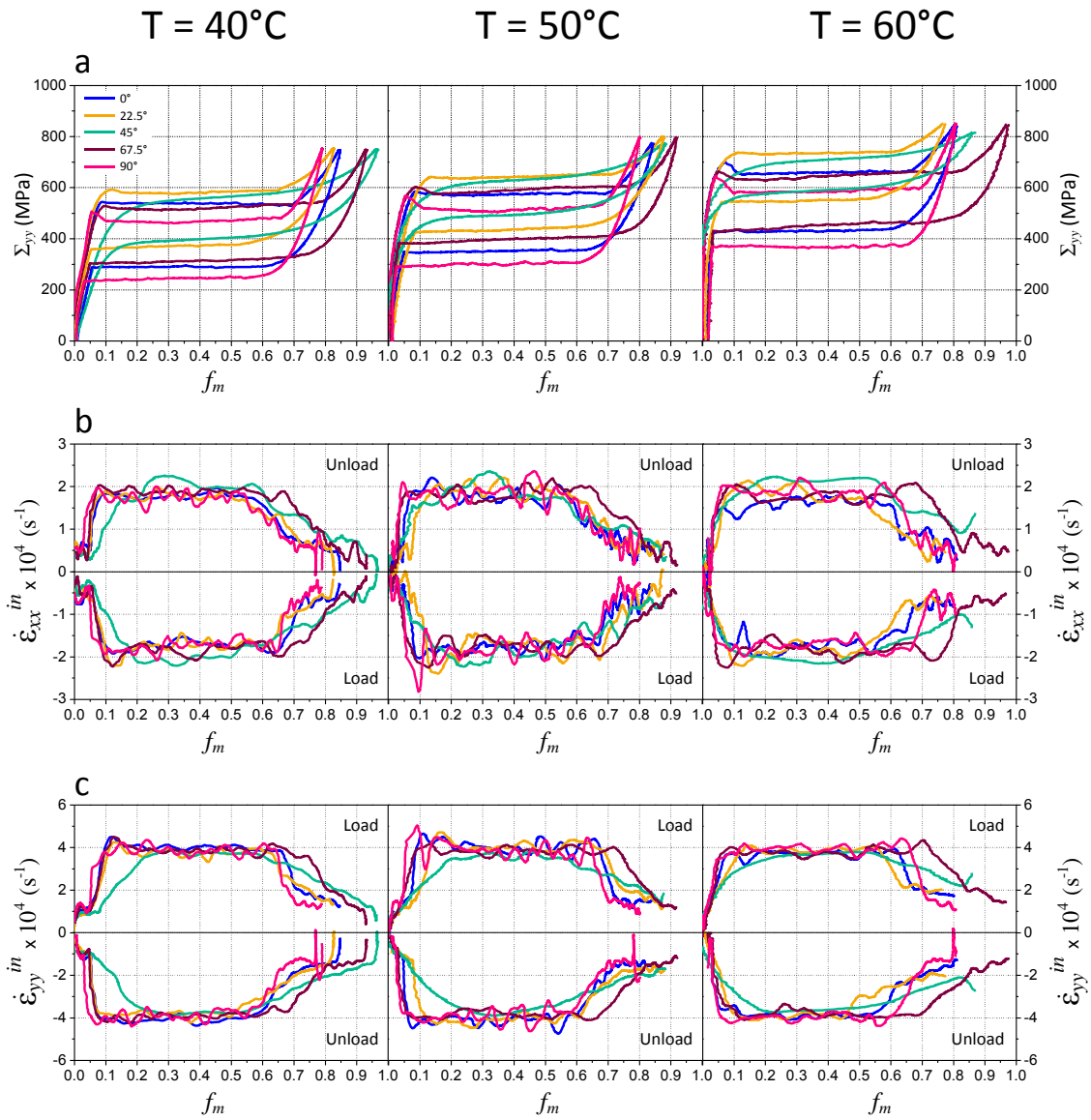
Figure 4.14: Evolution of averaged strain rates in the transverse and longitudinal directions of samples with martensite fraction.
