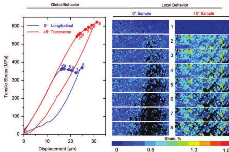
Figure 1.19: Evolution of grain local elastic strain of 0° and 45° NiTi digbone samples. The black zones are transformed grains (martensite phase). The samples' gauge length is 800μm which means loading was carried out until 3-4% tensile strain (From Barney et al., 2011).
