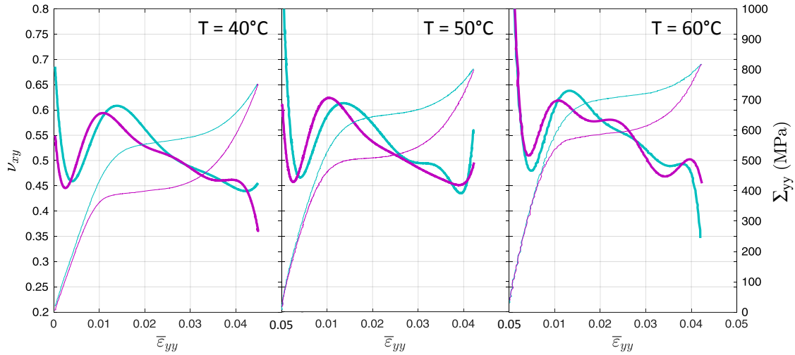
Figure 4.10: Evolution of \nu_{xy} at \theta = 45^\circ for tensile tests at 40°C, 50°C and 60°C.
