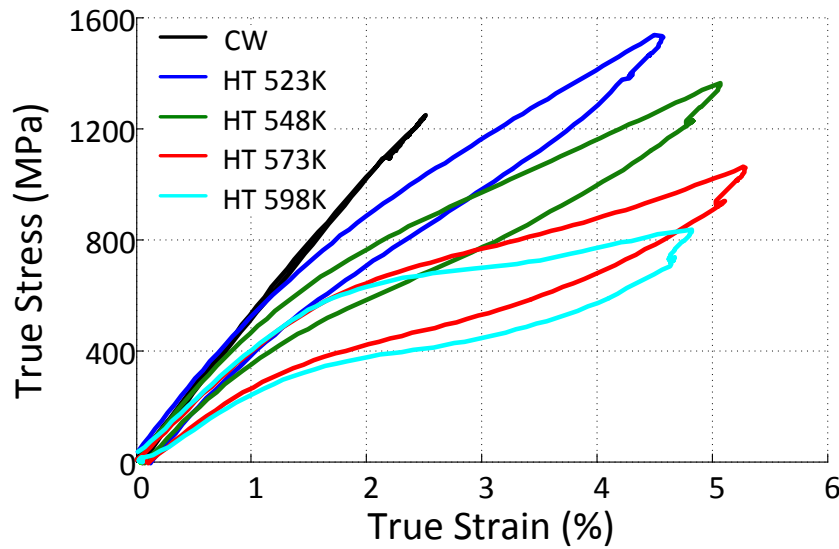
Figure 2.3: Superelastic tensile behavior of the Ti-50.9\text{ at\% Ni} wire CW and submitted to different heat treatments.
