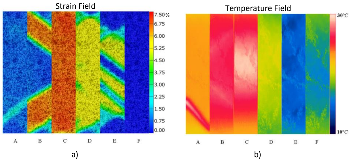
Figure 1.16: a) Strain field obtained trough DIC and b) temperature field obtained trough IR camera of a dog-bone shaped NiTi specimen showing localization pattern. (Adapted from Xie et al., 2016)
