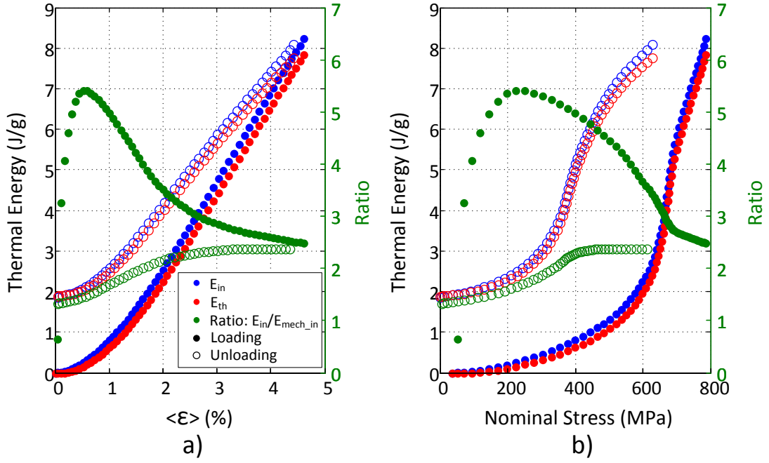
Figure 3.13: a) Thermal energy ( E_{th} ) and the inelastic thermal energy ( E_{in} ) on left ordinate axis and Energy ratio ( E_{in}/E_{mech\_in} ) on the right ordinate axis in function of true strain. b) Same values in function of nominal stress.
