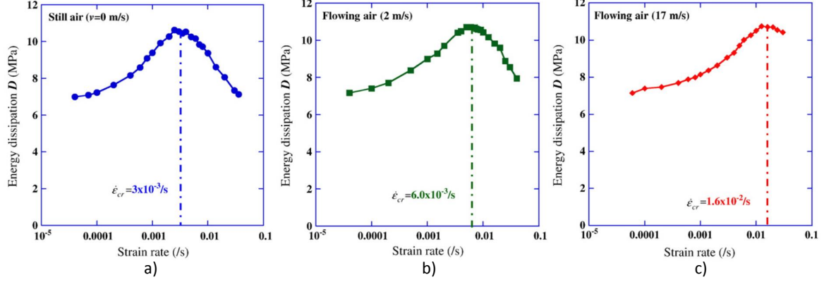
Figure 1.10: Energy dissipation (hysteresis area) in function of strain rate at three different ambient conditions (a) still air, (b) airflow at v = 2 m/s and (c) airflow at v = 17 m/s (dapted from He et al., 2010).
