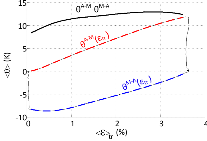
Figure 3.18: Average temperature variation \langle \theta \rangle in function of the average transformation strain \langle \epsilon_{tr} \rangle . The dashed red line stands for the temperature variation during loading ( \theta^{A-M}(\epsilon_{tr}) ) and the blue dashed line during unloading ( \theta^{M-A}(\epsilon_{tr}) ). The black curve stands for the difference between temperature variation during loading and unloading ( \theta^{A-M} - \theta^{M-A} ).
