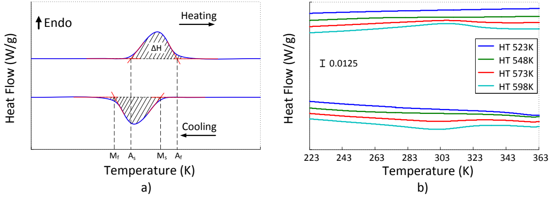
Figure 2.4: a) Graphical representation of a classic DSC curve and methodology to determine the specific latent heat and the critical temperatures. b) Actual DSC results of heat treated NiTi wires.
