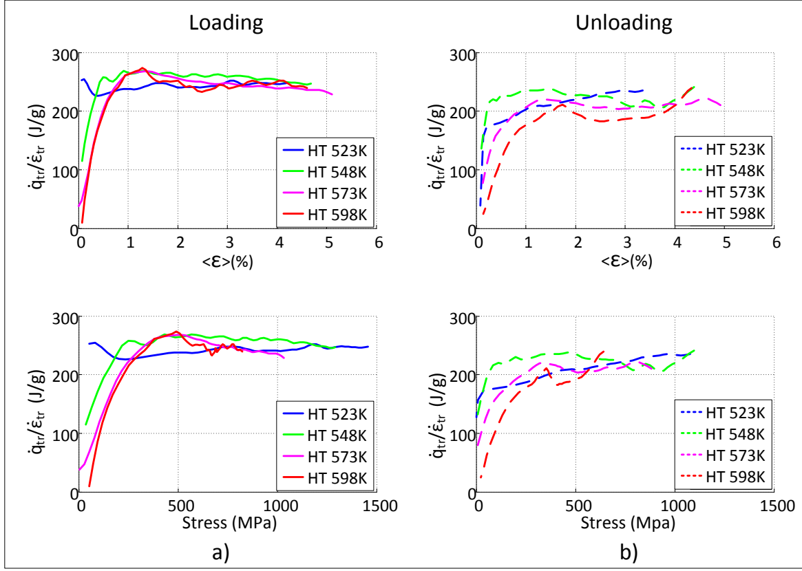
Figure 4.9: Ratio \dot{q}_{tr}/\dot{\varepsilon}_{tr} , computed with experimental data and Eq. 4.4, as a function of strain and stress during a) loading and b) unloading for all heat treated wires.
