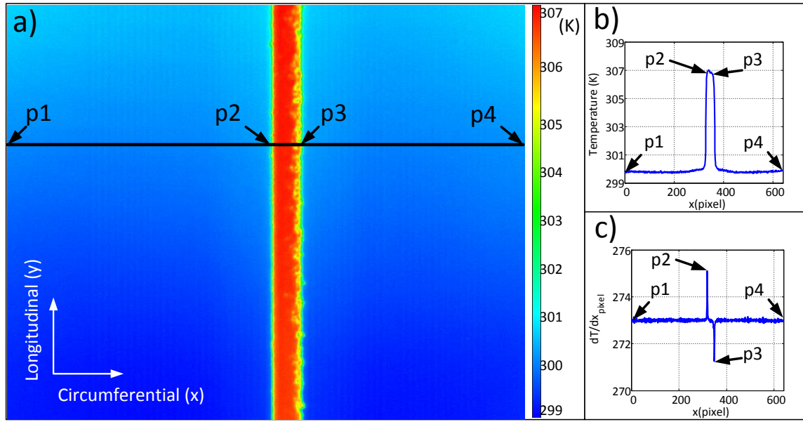
Figure 2.17: a) Example of thermal image of a tested wire. b) Temperature profile of the blue line shown in a). c) Spatial (x direction) temperature derivate curve used to determine the wire's position on thermal image.
