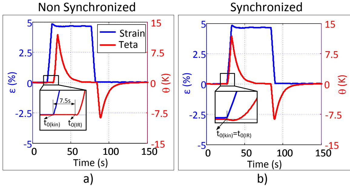
Figure 2.24: a) Example of experimental data with both axial strain ( \epsilon ) and temperature variation ( \theta ) before synchronization. b) and after synchronization.
