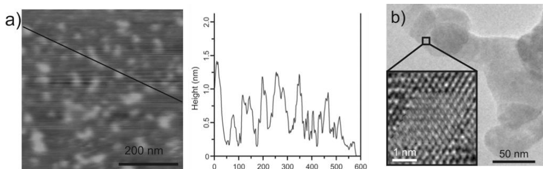
Fig. 2.25. (a) AFM image of [CoO 2 ] - nanosheets dropcasted from the exfoliated suspension onto mica substrate with the correspondent height profile revealing the presence of individual sheets with 0.35 nm thickness and (b) a bright-field HRTEM image of the cobalt oxide nanosheets revealing hexagonal closed-packed arrangement of cobalt atoms. Reprinted with permission of [162].
