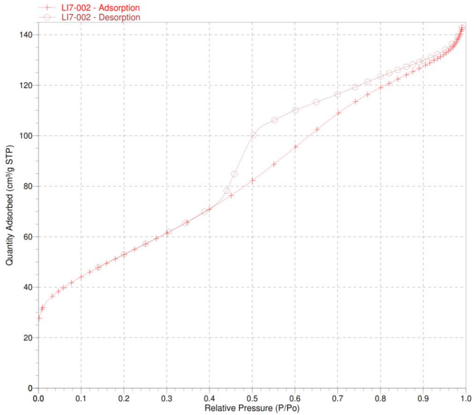
Fig. 3.5.18. BET adsorption-desorption isotherm results for NCO x -H.
