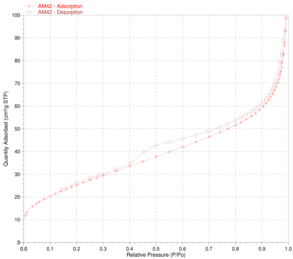
Fig. 3.5.19. BET adsorption-desorption isotherm results for NCO x -TBA.
