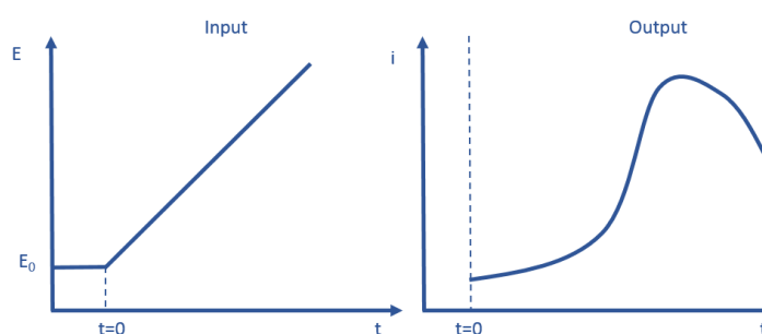
Fig. 2.12. Linear potential sweep voltammetry comparison for the input and output responses. Reprinted with copyright permission of [6].
