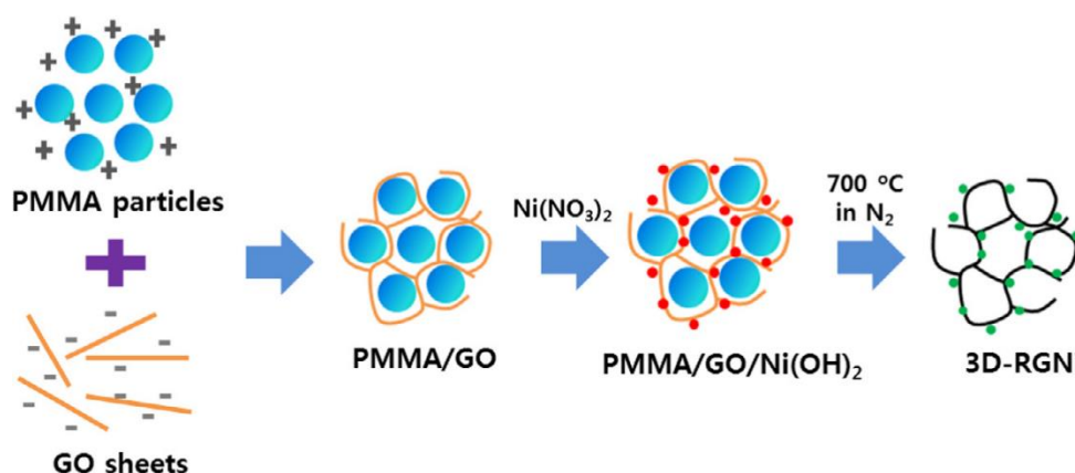
Fig. 1.16. Illustration of a synthesis process of reduced graphene oxide with nickel oxide nanoparticles developed by Trung et al. Reprinted with copyright permission of [199].
