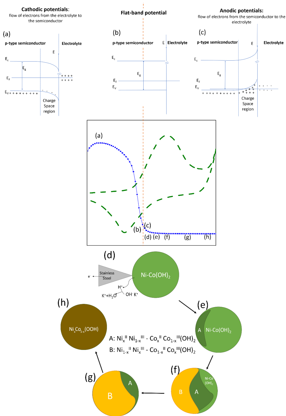
Fig. 3.2.5. Electronic and Phase model of the Charging process of Nickel-Cobalt hydroxide based on the current density (cyclic voltammetry) and charge-space capacitance (Mott-Schottky) as a function of the applied potential. (a) Illustration of the band bend occurring when the Fermi level of the semiconductor is placed higher than that of the electrolyte for a p-type semiconductor. (b) Illustration of the equilibrium state of bands when the Fermi level of the semiconductor is the same of the electrolyte. (c) Illustration of the band bend happening when the Fermi level of the semiconductor is placed lower than that of the electrolyte for a p-type semiconductor. (d-e) Modification of the phase transformations occurring during the charging process for the Ni-Co double hydroxide materials first presented by Barnard, Randell and Tye [43].
