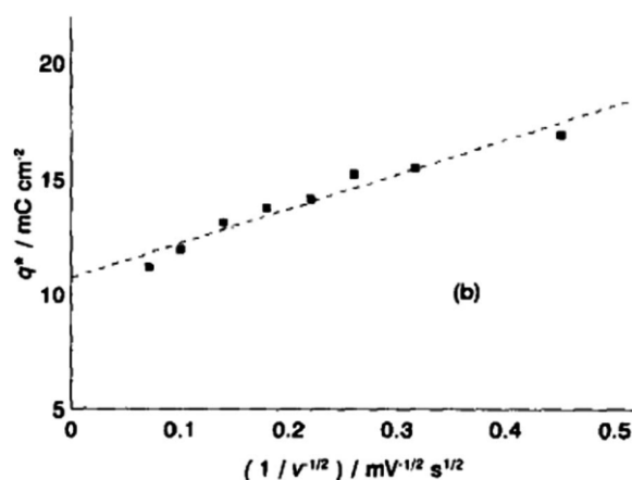
Fig. 1.13. Kinetic analysis of capacity contribution from outer surface response proposed by Trasatti et al. The y-intercept would correspond to the infinite sweep rate capacity. Reprinted with copyright permission from [170].
