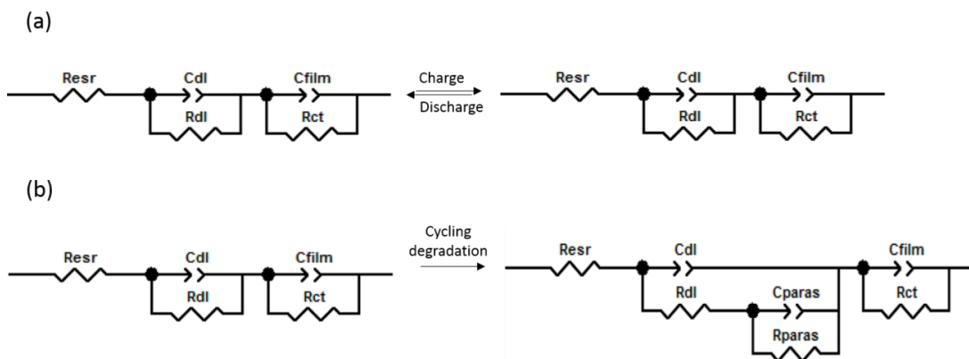
Fig. 3.4.17. (a) General equivalent circuit model used in the fitting of the impedance spectra acquired for NCO x and NCO x /Er-GO for the results obtained at -0.2V (discharged) and 0.45V (charged) and (b) Equivalent circuit model used in the fitting of impedance spectra acquired for NCO x /Er-GO at -0.2V with cycling after 750, 1500 and 5000 cycles.
