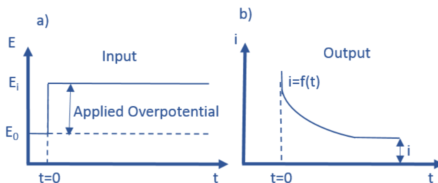
Fig.2.10. Variation of current with time for potentiostatic electrodeposition. Reprinted with copyright permission of [6].
