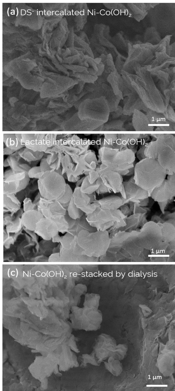
Fig. 3.5.4 Scanning Electron Microscopy images of (a) DS-NCOH, (b) Lac-NCOH and (c) restacked nickel-cobalt hydroxide nanoslabs by dialysis after exfoliation in distilled water (NCOH-DIAL).
