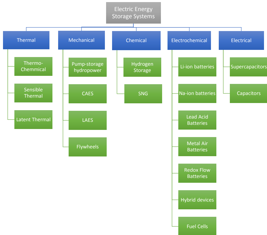
Fig. 1.2. Scientific categorization of Electrical Energy storage systems. CAES stands for Compressed Air Energy Storage; LAES for Liquid Air Energy Storage; SNG for Synthetic Natural Gas. Note that this list is representative of the major electrical energy storage systems and may not include all of them. Diagram extracted and modified with copyright permission of the E-Storage report on World Energy Resources by the World Energy Council [10].
