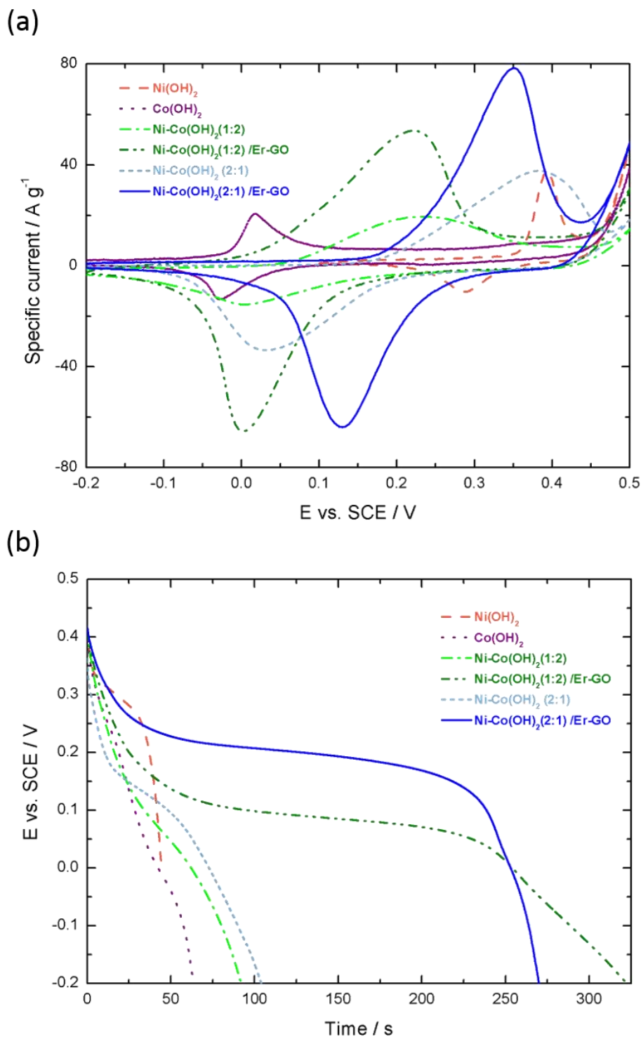
Fig. 3.1.9. (a) Cyclic Voltammetry comparison at 50 mV/s and (b) Galvanostatic Charge Discharge comparison at 1A/g.
