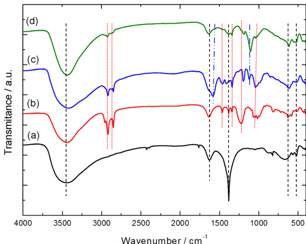
Fig. 3.5.7. Fourier-transform infrared spectroscopy results for (a) NCOH taken as reference material, (b) SDS-NCOH, (c) Lac-NCOH and (d) NCOH-DIAL after exfoliation in H 2 O and re-stacking by dialysis.
