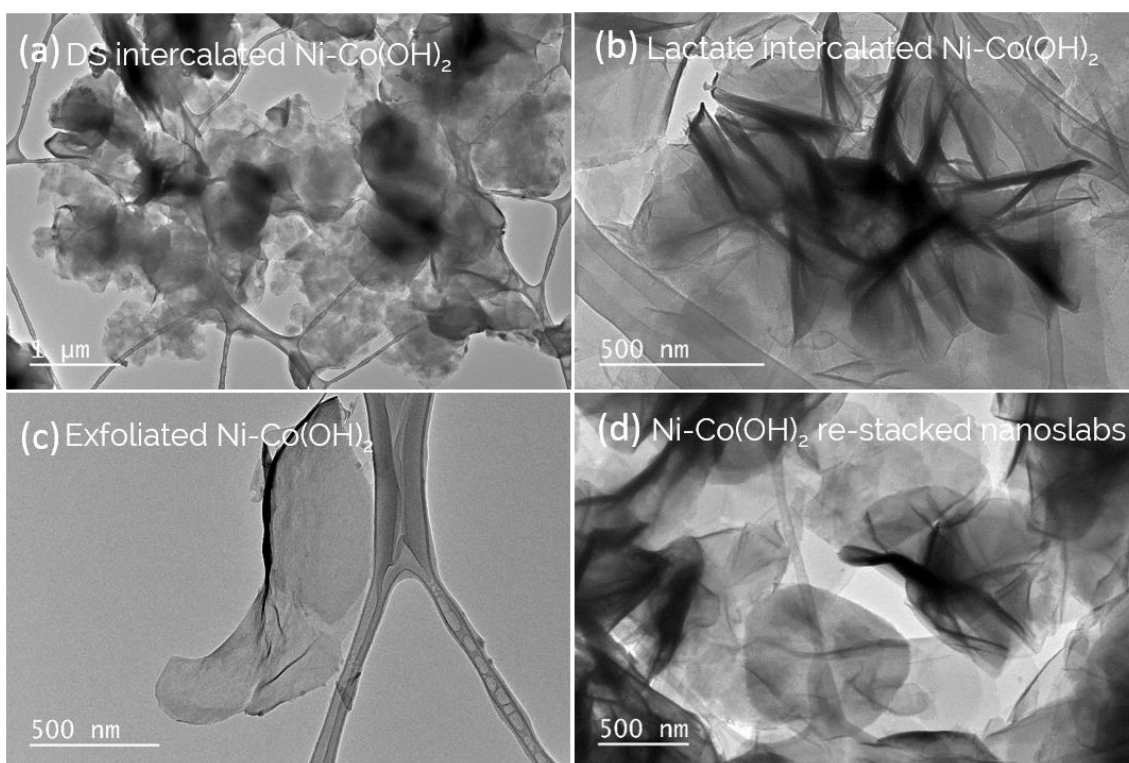
Fig. 3.5.5 Transmission Electron Microscopy images of (a) DS-NCOH, (b) Lac-NCOH, (c) delaminated nanoslabs of lactate intercalated \text{Ni-Co(OH)}_2 in distilled water and (d) restacked nanoslabs of delaminated \text{Ni-Co(OH)}_2 slabs obtained by dialysis (NCOH-DIAL).
