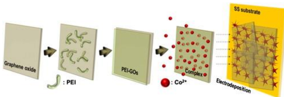
Fig. 1.17. Schematic representation of the co-electrodeposition of cobalt oxide/graphene composite material. Reprinted with copyright permission of [230].
