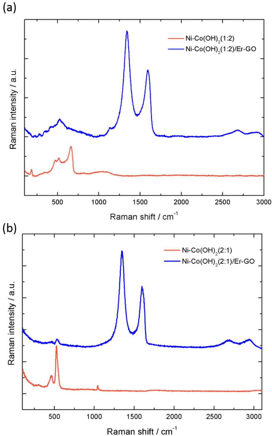
Fig. 3.1.7. Raman Spectra for (a) Ni-Co(OH) 2 (1:2) and Ni-Co(OH) 2 (1:2)/Er-GO and (b) Ni-Co(OH) 2 (2:1) and Ni-Co(OH) 2 (2:1)/Er-GO Electrodeposited on Stainless Steel.
