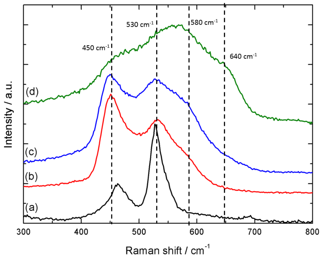
Fig. 3.5.17. Raman results for (a) NCOH, (b) NCO x -HNK, (c) NCO x -H and (d) restacked NCO x -TBA.
