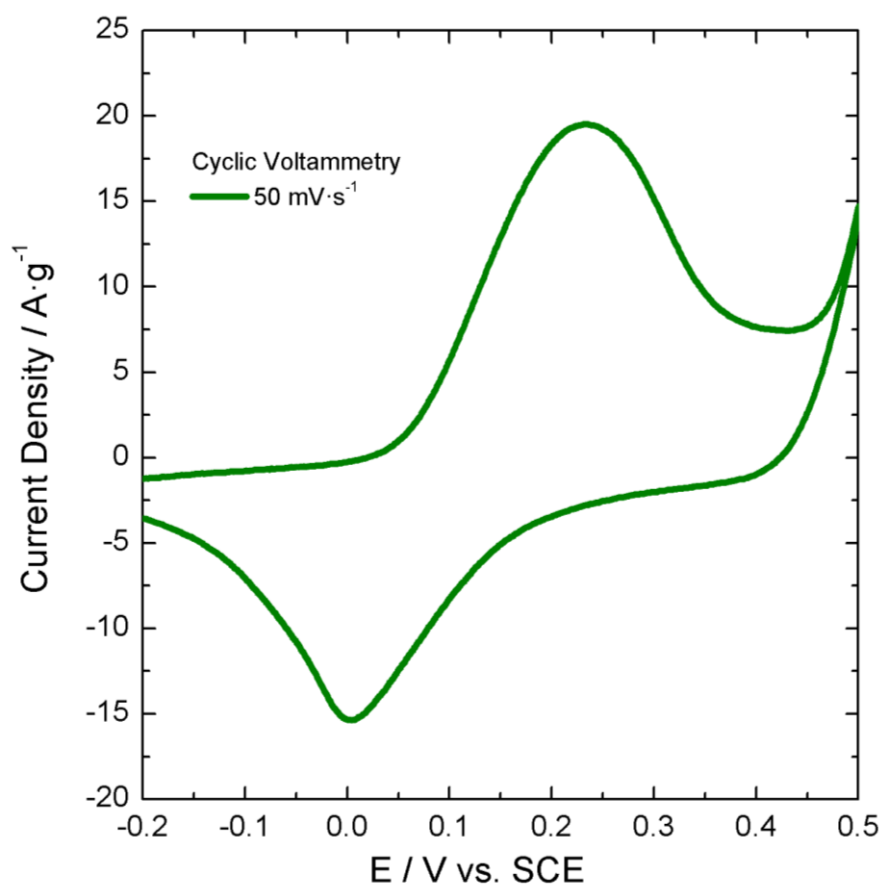
Fig. 3.2.2. Cyclic Voltammetry at 50 \text{ mV}\cdot\text{s}^{-1} plot for Ni-Co(OH) 2 (1:2) [30].
