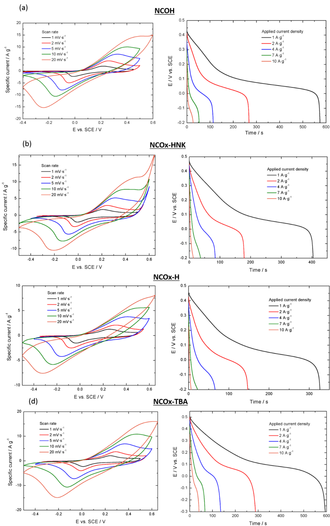
Fig. 3.5.30. Cyclic voltammeties at different scan rates and galvanostatic discharge curves at different applied current densities for the materials obtained during the delamination of nickel-cobalt oxyhydroxide by tetrabutylammonium intercalation evaluated in 1M LiOH.
