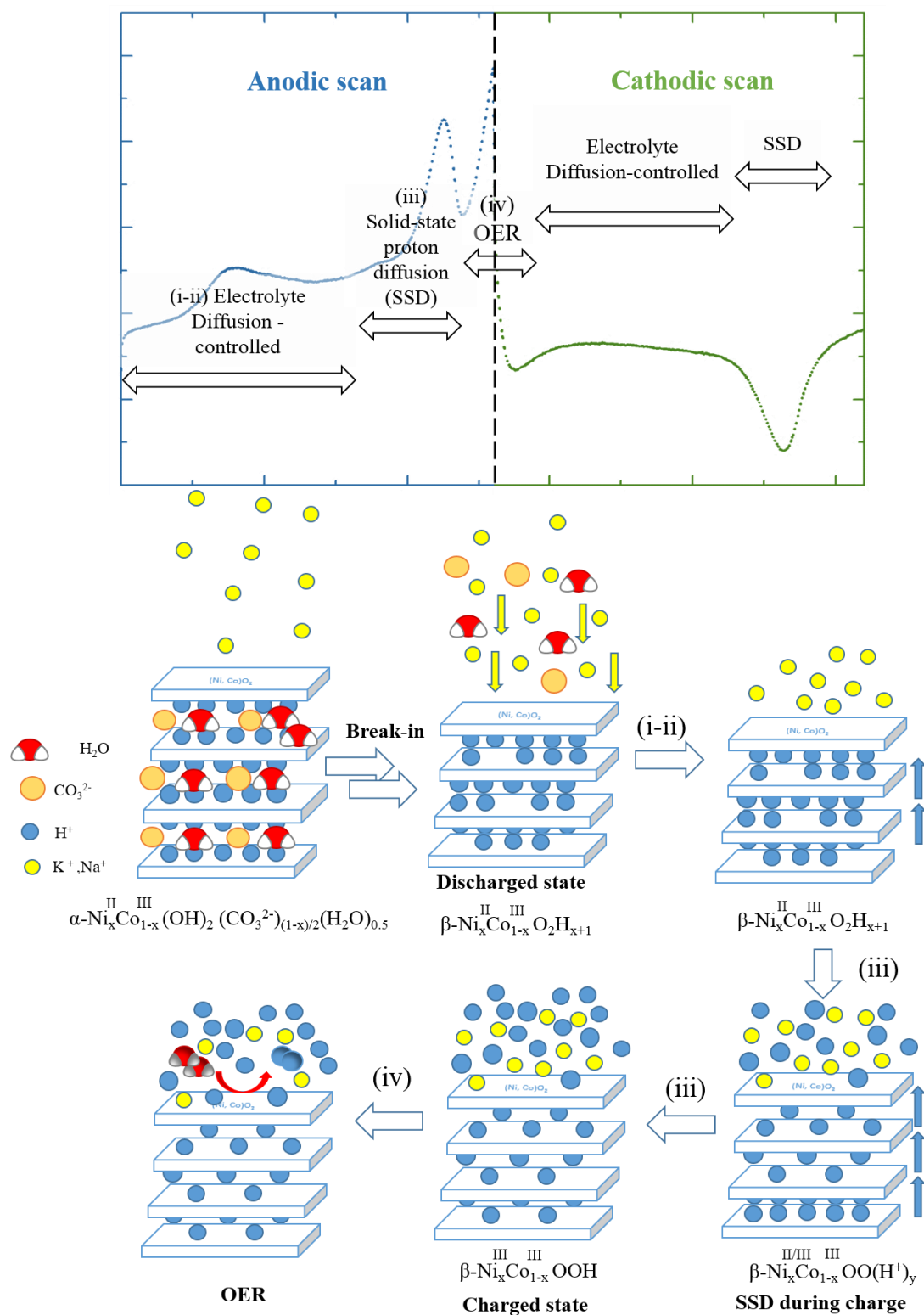
Fig. 3.3.5. Schematic representation of the processes occurring during oxidation-reduction of Ni_xCo_{1-x}(OH)_2 in K_2SO_4/Na_2SO_4 0.05M.
