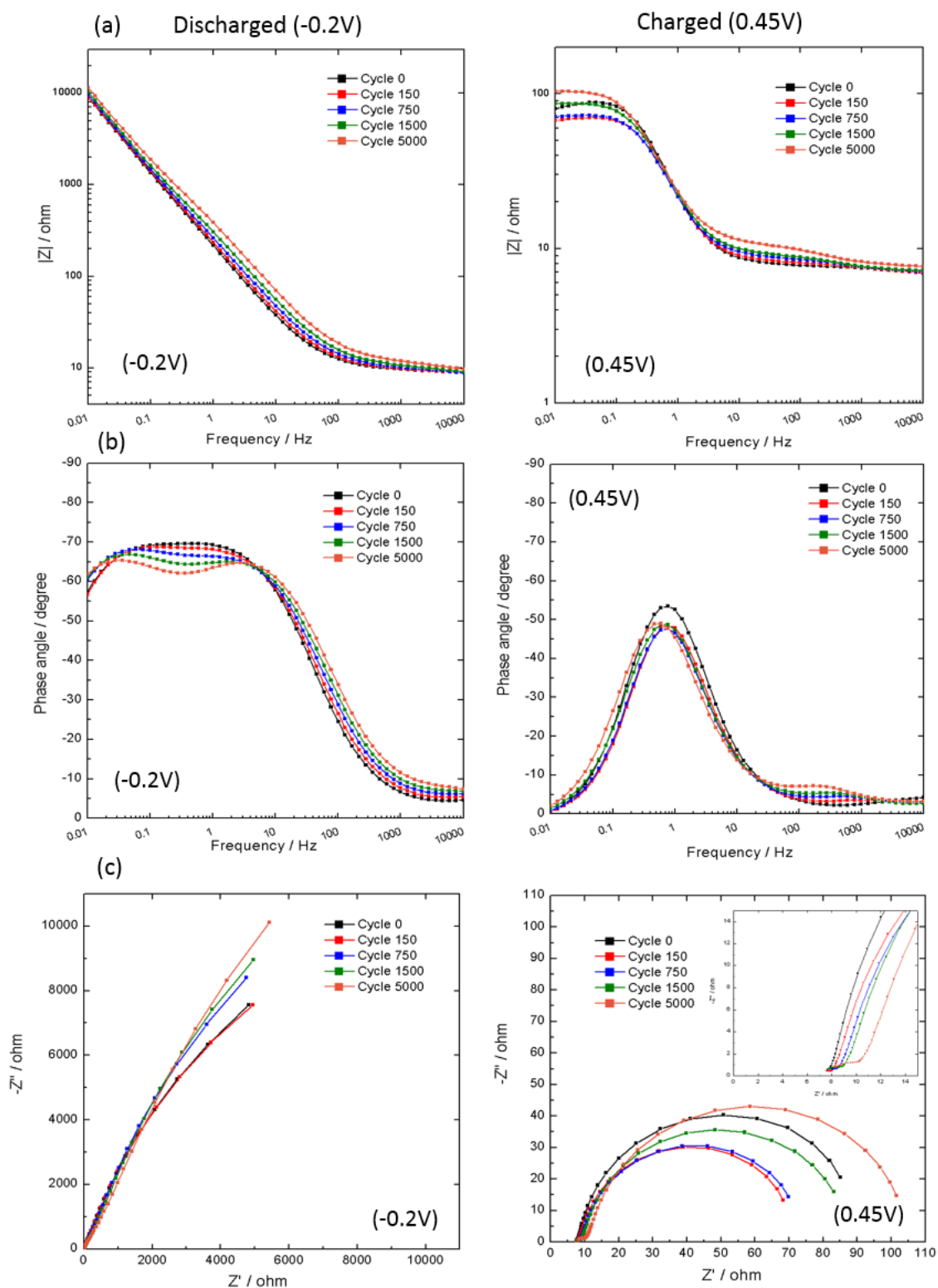
Fig. 3.4.16. (a) and (b) Bode and (c) Nyquist Electrochemical Impedance Spectra for NCO x /Er-GO composite material after 0, 150, 750, 1500 and 5000 cycles of Galvanostatic Charge Discharge at 8 A/g for both discharged (-0.2V, left) and charged (0.45V, right) potentials.
