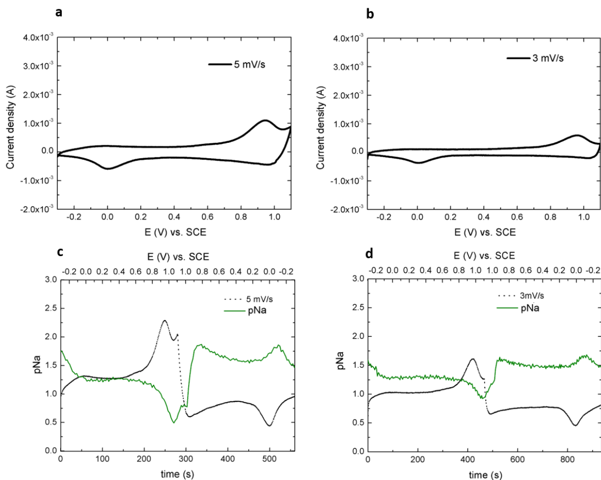
Fig. 3.3.4. Cyclic voltammetry at: a) 5 \text{ mV}\cdot\text{s}^{-1} and b) 3 \text{ mV}\cdot\text{s}^{-1} and their expanded version in time c) and d) with the corresponding in-situ measurements of pNa within a potential ranging from -0.3 \text{ V} to 1.1 \text{ V} in \text{Na}_2\text{SO}_4 0.05 \text{ M} .
