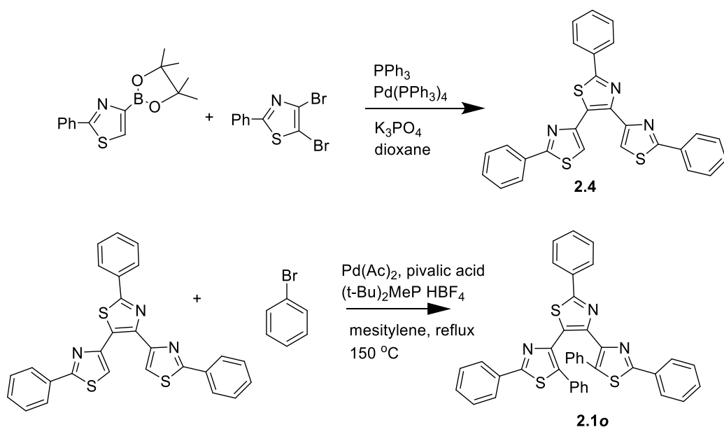
Scheme 2.4. Synthesis route for 2.1o . See Section 7.1.2 for details.
