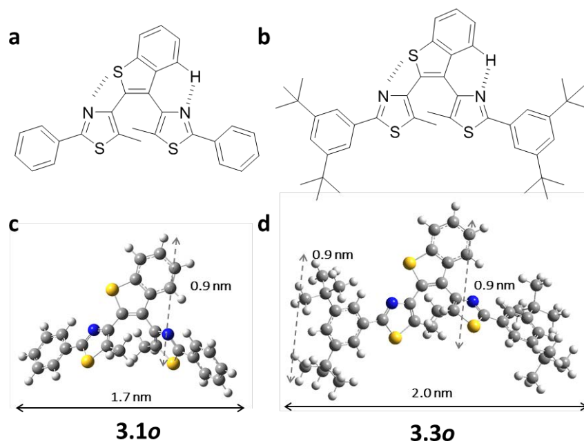
Figure 5.1. Structures of (a) 3.1o and (b) 3.3o showing the intramolecular forces that keep them in their reactive conformation and their DFT-optimized structures shown in (c) and (d) respectively.
