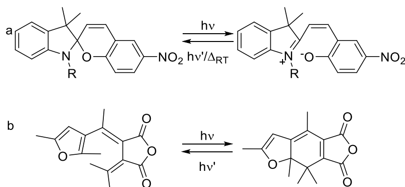
Scheme 1.2. Structure and photochromism of (a) spiropyrans and (b) fulgides.
