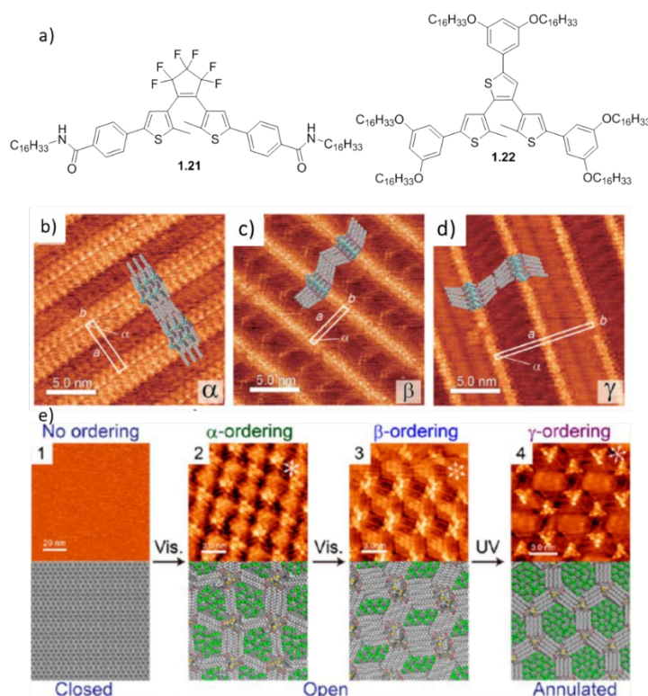
Figure1.5. a) Structures of 1.21 and 1.22 . b-d) assemblies of the o , c , and annulated form of 1.21 . Packing parameters for b) a = 5.71 nm, b = 0.89 nm, \alpha = 88^\circ ; c) a = 4.82 nm, b = 0.56 nm, \alpha = 85^\circ ; d) a = 10.2 nm, b = 0.48 nm, \alpha = 87^\circ ; data from ref. 77. e) Four state switching of compound 1.22 from the c form, two concentration-dependent orderings of the o forms, and that of the annulated form. From ref. 81.
