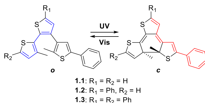
Scheme 1.4. Switching of \pi electron pathways in two isomers due to the incorporation of aromatic rings on the bridge. [24]
