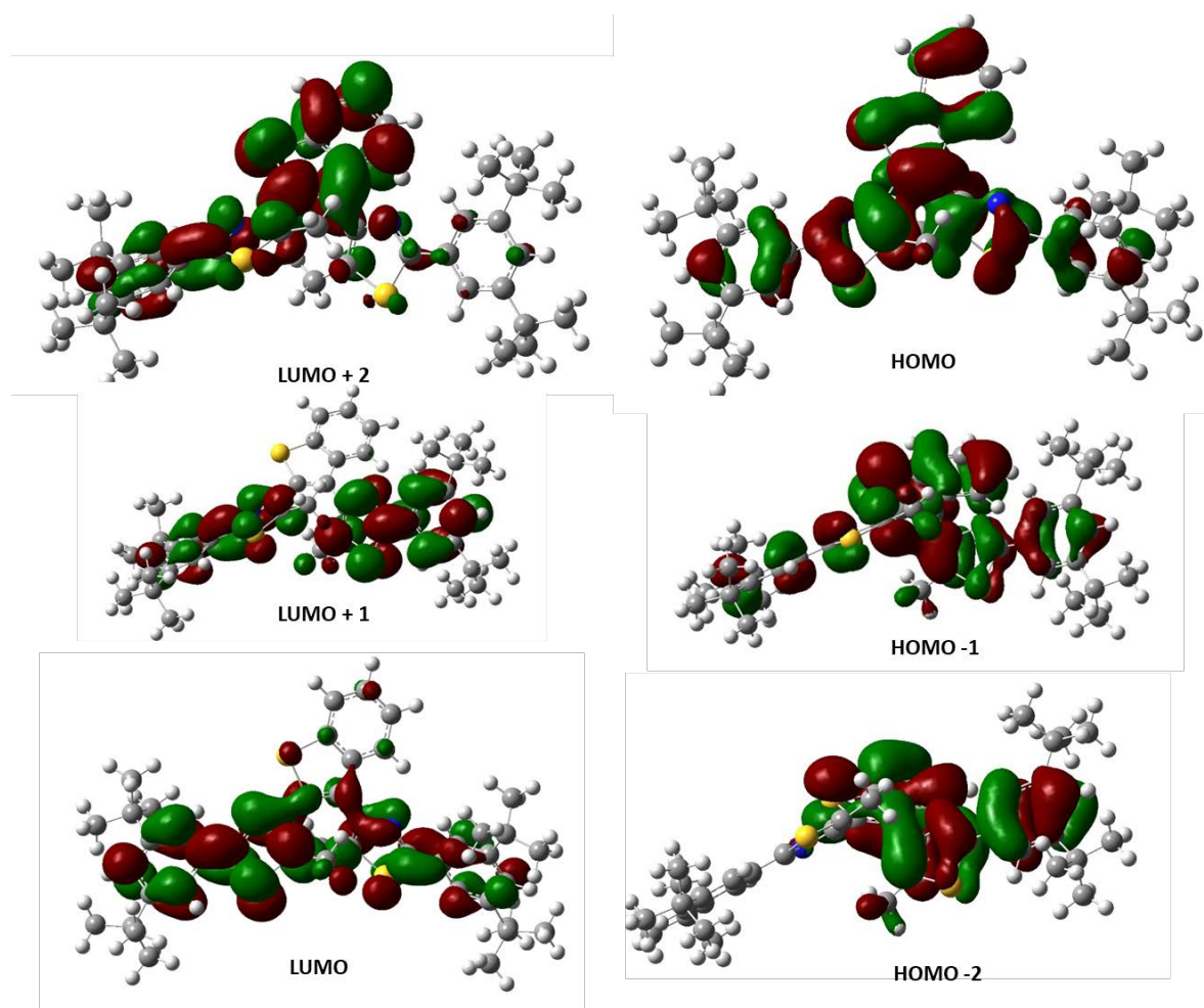
Figure 5.4. Maps of HOMO-2 to LUMO+2 of 3.3o showing that the tert -butyl groups do not contribute to these orbitals.
