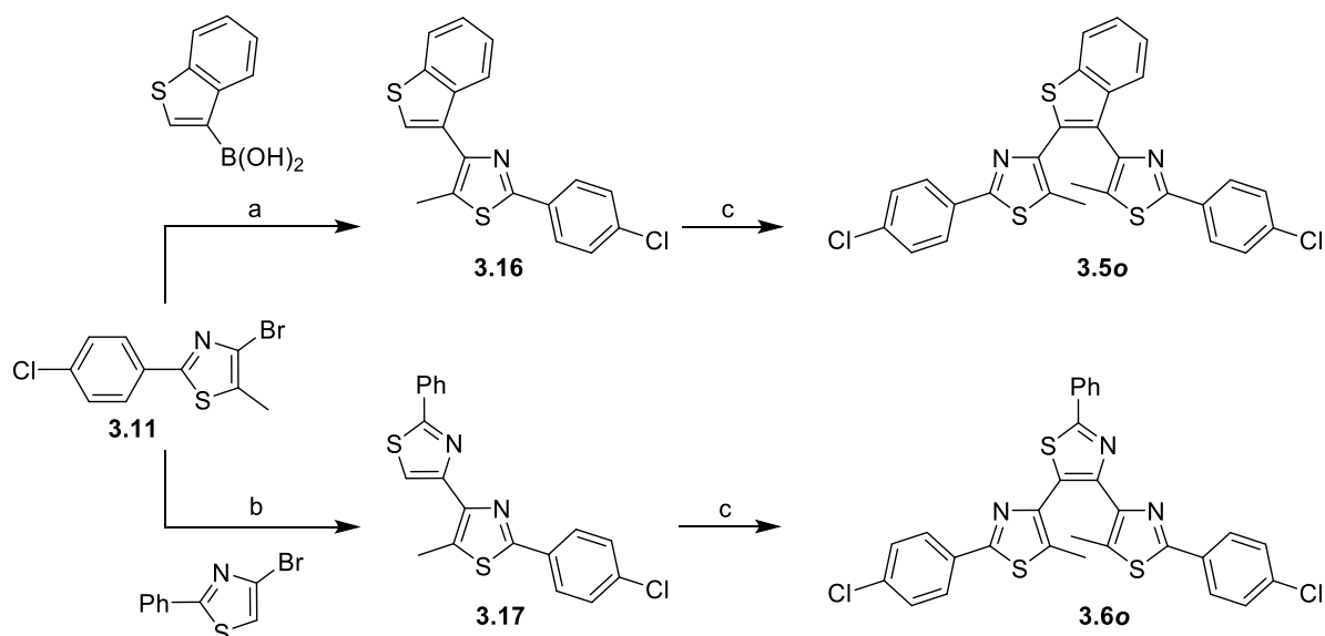
Scheme 3.4. Synthesis of chloro-functionalized terarylenes 3.5o and 3.6o . a) benzo[b]thien-3-ylboronic acid \text{Pd}(\text{PPh}_3)_4 , \text{K}_3\text{PO}_4 , DME, \text{H}_2\text{O} ; b) 1. n\text{-BuLi} , \text{B}(\text{OMe})_3 , THF; 2. 4-bromo-2-phenylthiazole, \text{Pd}(\text{PPh}_3)_4 , \text{K}_3\text{PO}_4 , DME, \text{H}_2\text{O} ; c) 3.11 , \text{Pd}(\text{OAc})_2 , \text{Cs}_2\text{CO}_3 , pivalic acid, di- tert -butyl(methyl)phosphonium tetrafluoroborate, mesitylene.
