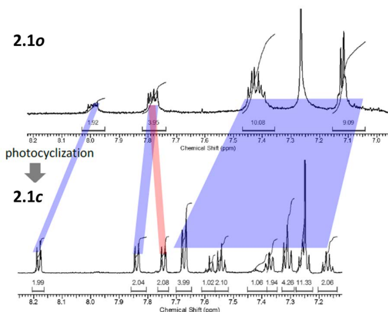
Figure 2.4. Comparison between ^1\text{H} NMR spectra of the aromatic regions of 2.1o and 2.1c in \text{CDCl}_3 showing the resolution of more aromatic peaks in c forms.
