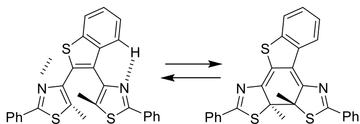
Scheme 1.7. Photochromism of 1.8 showing S-N and N-H interactions. [31]
