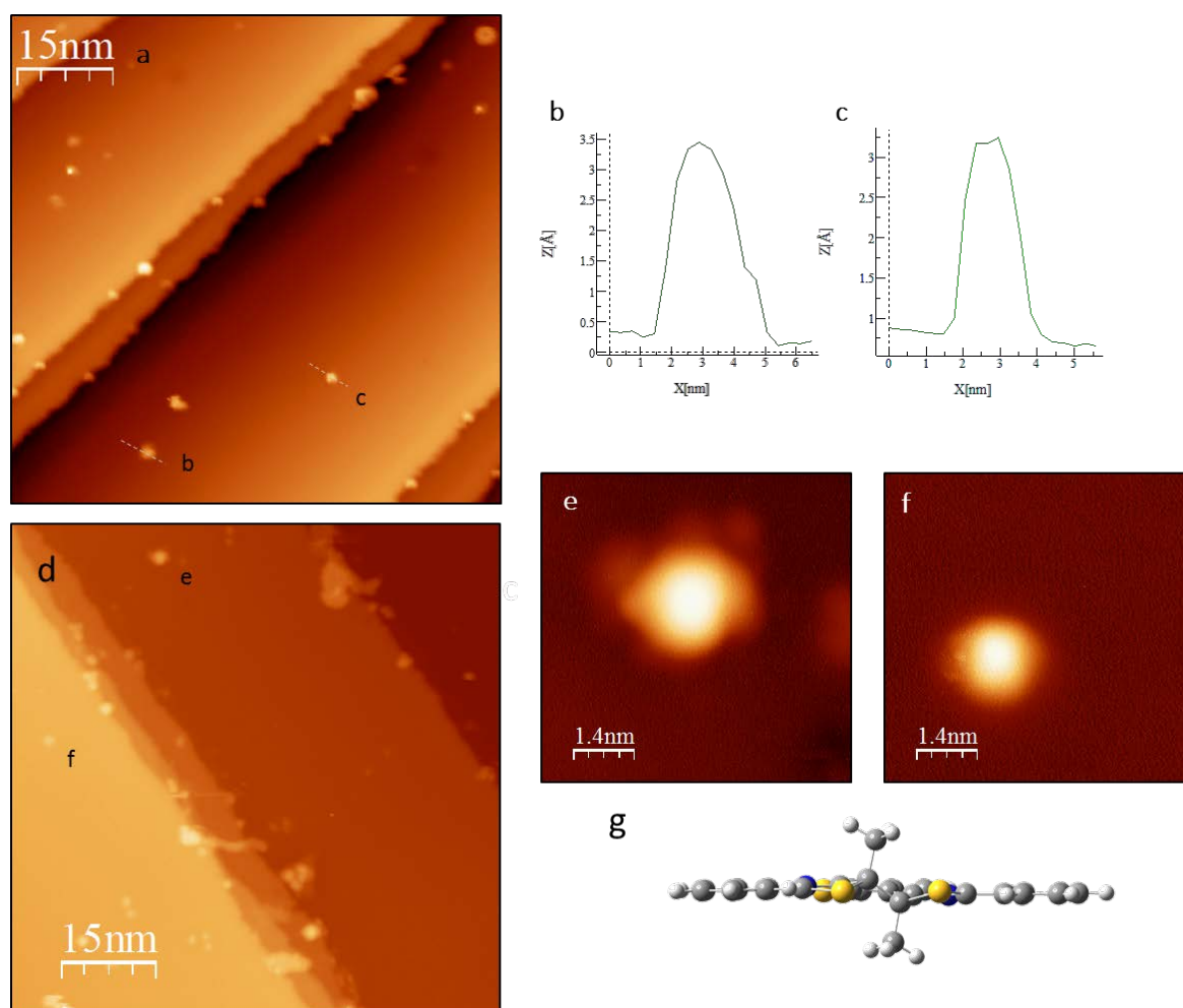
Figure 5.3. (a,d) shows Ag(111) deposited with 3.1c . (b-c) show line scans of spots as labelled in (a) while (e-f) show zoom in on the spots as labelled in (d). Imaging conditions: -1 V, 1 pa. (g) shows the DFT-optimized structure of 3.1c as seen from the plane of the photoswitching unit.
