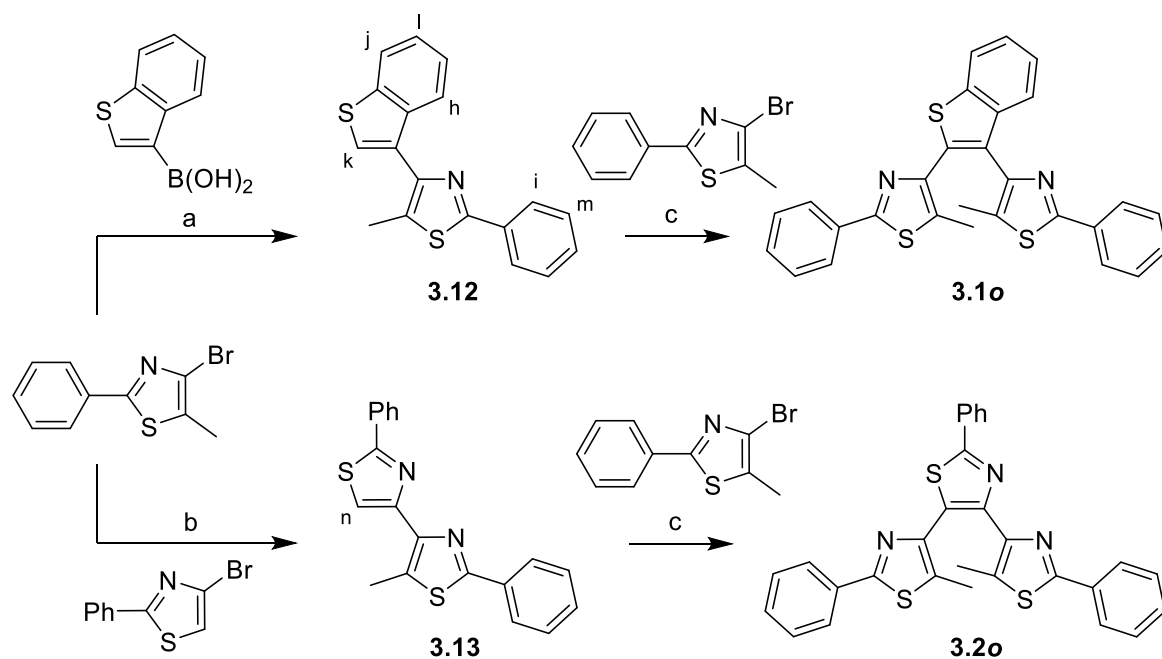
Scheme 3.2. Synthesis of model compounds 3.1o and 3.2o by a new synthetic pathway. a) benzo[b]thien-3-ylboronic acid \text{Pd}(\text{PPh}_3)_4 , \text{K}_3\text{PO}_4 , DME, \text{H}_2\text{O} ; b) 1. n\text{-BuLi} , \text{B}(\text{OMe})_3 , THF; 2. 4-bromo-2-phenylthiazole, \text{Pd}(\text{PPh}_3)_4 , \text{K}_3\text{PO}_4 , DME, \text{H}_2\text{O} ; c) 4-bromo-5-methyl-2-phenylthiazole, \text{Pd}(\text{OAc})_2 , \text{Cs}_2\text{CO}_3 , pivalic acid, di- tert -butyl(methyl)phosphonium tetrafluoroborate, mesitylene.
