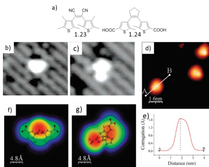
Figure 1.7. a) Structure of 1.23 and 1.24 . b) and c) are STM images of the o and c forms of 1.23 from ref. 85. d) Deposition of 1.24 results an assymetric one which is highlighted by the line scan in (e). By ESQC calculations on the parallel (f) and anti-parallel (g) conformation of 1.24 , the experimental images were assigned to the anti-parallel conformation.
