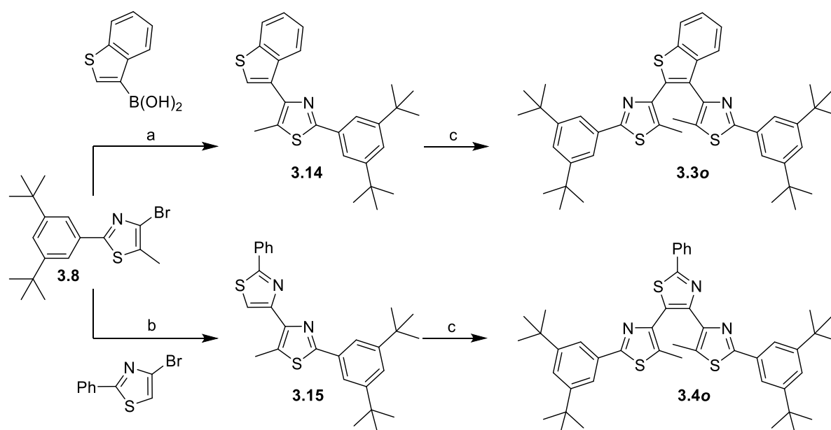
Scheme 3.3. Synthesis of the tert -butyl-functionalized terarylenes 3.3o and 3.4o . a) benzo[b]thien-3-ylboronic acid \text{Pd}(\text{PPh}_3)_4 , \text{K}_3\text{PO}_4 , DME, \text{H}_2\text{O} ; b) 1. n\text{-BuLi} , \text{B}(\text{OMe})_3 , THF; 2. 4-bromo-2-phenylthiazole, \text{Pd}(\text{PPh}_3)_4 , \text{K}_3\text{PO}_4 , DME, \text{H}_2\text{O} ; c) 3.8 , \text{Pd}(\text{OAc})_2 , \text{Cs}_2\text{CO}_3 , pivalic acid, di- tert -butyl(methyl)phosphonium tetrafluoroborate, mesitylene.
