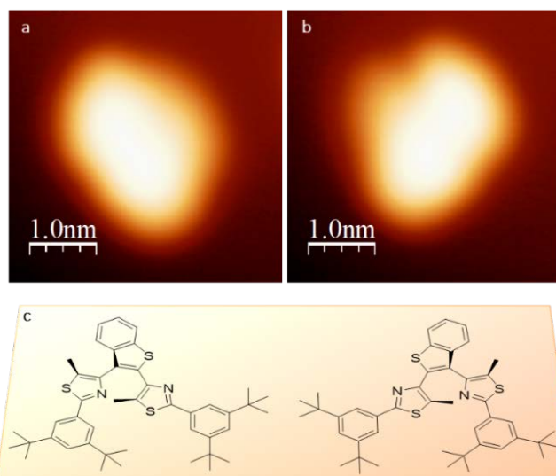
Figure 5.8. a-b) Enantiomeric forms of Form 2. Imaging conditions: 1.0 V, 1pA, T=4.5 K. c) Illustration of chirality of 3.3o - C_2 when in contact with a 2D surface.
