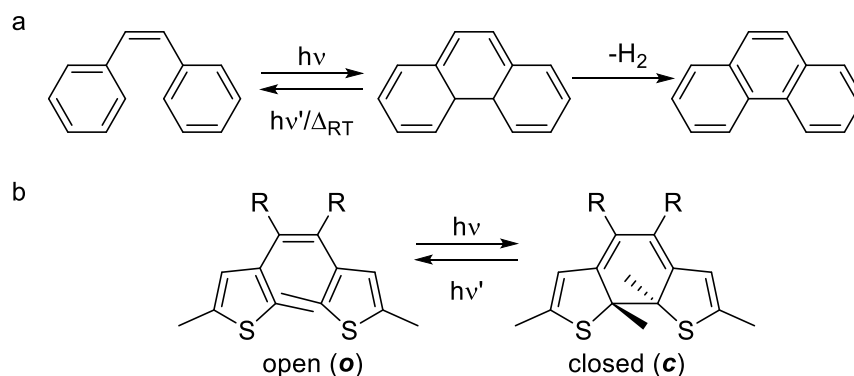
Scheme 1.3. a) Irie's initially attempted to prevent this irreversible \text{H}_2 elimination by synthesizing 2,3-dimesitylbutadiene. b) Synthesis failed due to steric hindrance so they replaced the compound with a smaller thiophene derivative which surprisingly did not show thermal reversion but could be reverted back by visible light instead. [20]
