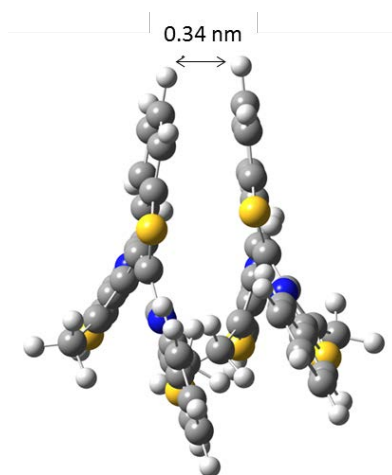
Figure 4.6. Molecular mechanics(Materials Studio 7.0) calculation of \pi - \pi interaction stacking distance.
