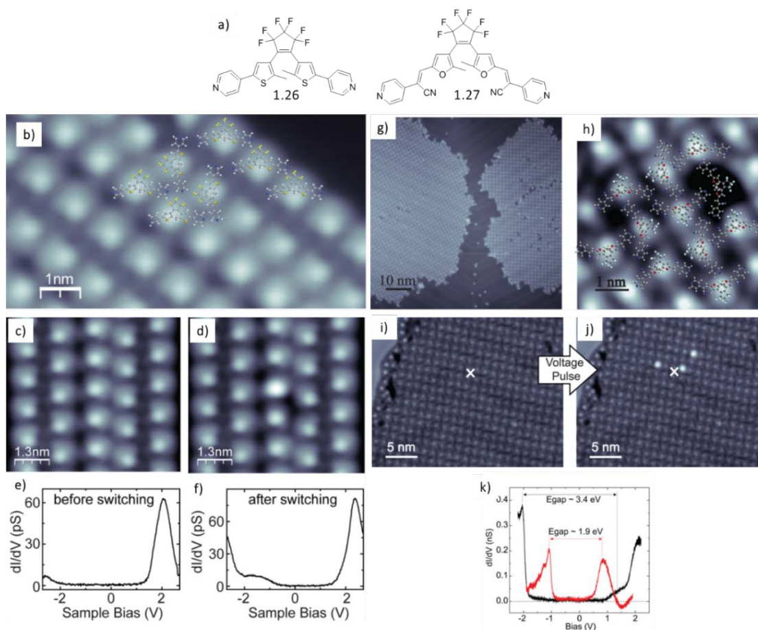
Figure 1.9. a) Structure of 1.26 and 1.27. (b) Deposition of 1.26 showed assemblies of the compound stabilized by H-bonding interactions. c) and d) show the same area before and after a switch-inducing bias pulse was applied. e) and f) show STS spectra before and after the switching event. Data from ref. 89. g) and h) show large-scale and zoom-in images on assemblies of 1.27. A higher contrast was seen upon switching (i and j). k) STS spectrum of the unswitched (dark) and switched (red) molecules. Data from ref. 91.
