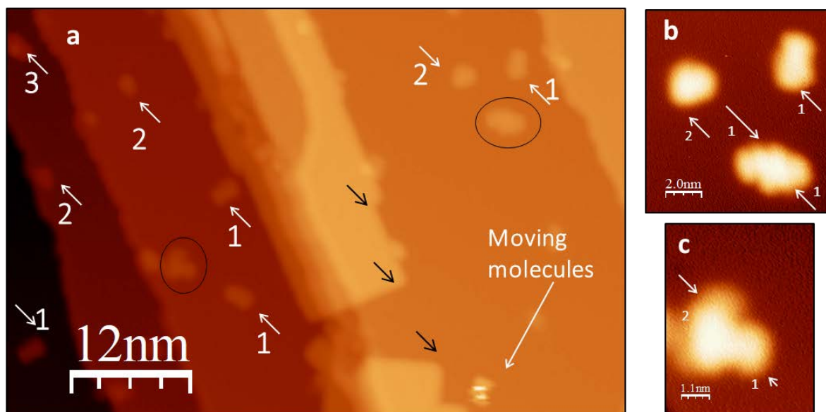
Figure 5.5. a) Sample of a large scale image (1.4 V, 1 pA, T = 4.5 K) of Ag(111) with 2 monolayers of NaCl followed by subsequent deposition of 3.30 . Dark arrows point to 90^\circ corners characteristic of NaCl(001) crystal structure; dark ovals on aggregates of molecules; white arrows point to different forms of the compound with their corresponding label. b-c) Zoom in on the species inside the dark arrows
