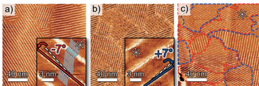
Figure 1.6. STM images of the (a) (R,R) isomer, (b) (S,S) isomer, and (c) racemic mixture of 1.15c . Adapted from ref. 84.
