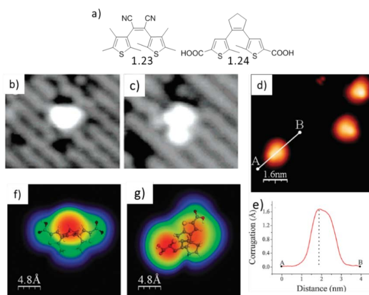
Figure 1.7. a) Structure of 1.23 and 1.24 . b) and c) are STM images of the o and c forms of 1.23 from ref. 85. d) Deposition of 1.24 results an asymmetric one which is highlighted by the line scan in (e). By ESQC calculations on the parallel (f) and anti-parallel (g) conformation of 1.24 , the experimental images were assigned to the anti-parallel conformation.
