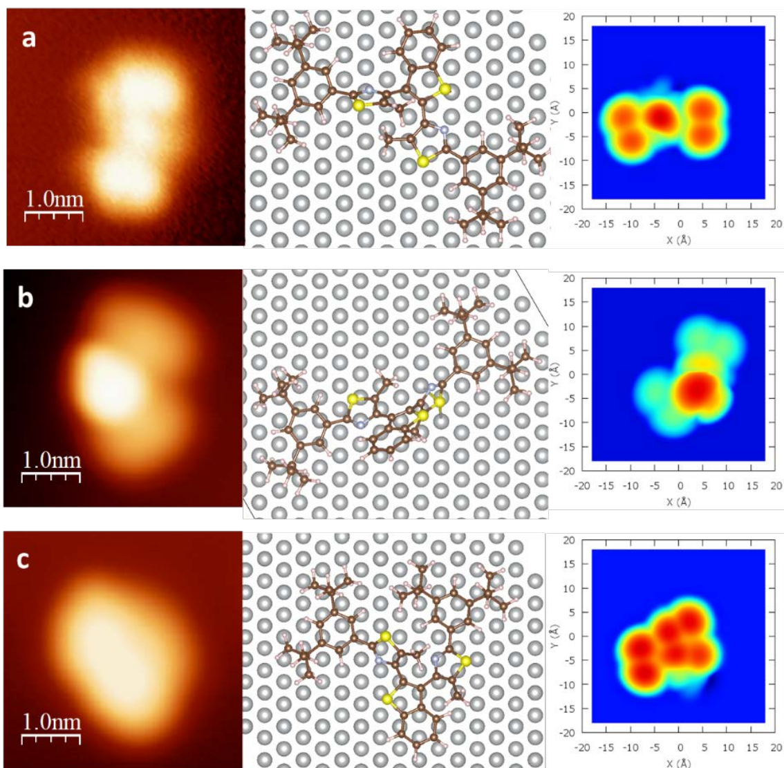
Figure 5.15. With the aid of ESQC calculations, we ascribe form 1 to the 3.30 trans form in (a) while that of form 2 to (b). (c) Form 3 refers to a cis isomer of 3.30 deposited on the surface.
