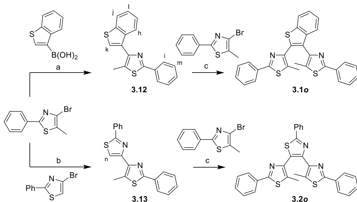
Scheme 3.2. Synthesis of model compounds 3.1o and 3.2o by a new synthetic pathway. a) benzo[b]thien-3-ylboronic acid Pd(PPh 3 ) 4 , K 3 PO 4 , DME, H 2 O; b) 1. n-BuLi, B(OMe) 3 , THF 2. 4-bromo-2-phenylthiazole, Pd(PPh 3 ) 4 , K 3 PO 4 , DME, H 2 O; c) 4-bromo-5-methyl-2-phenylthiazole, Pd(OAc) 2 , Cs 2 CO 3 , pivalic acid, di- tert -butyl(methyl)phosphonium tetrafluoroborate, mesitylene.
