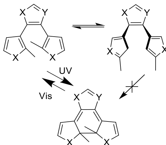
Scheme 2.1. The reactive and non-reactive conformation of diarylethenes/terarylenes.
