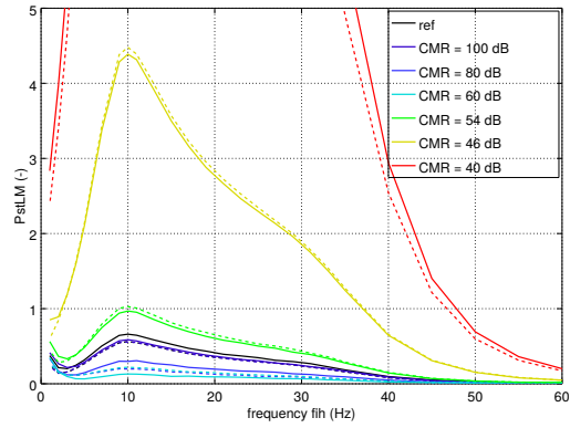
(b) Several values of CMRR ; first three lines almost overlap
