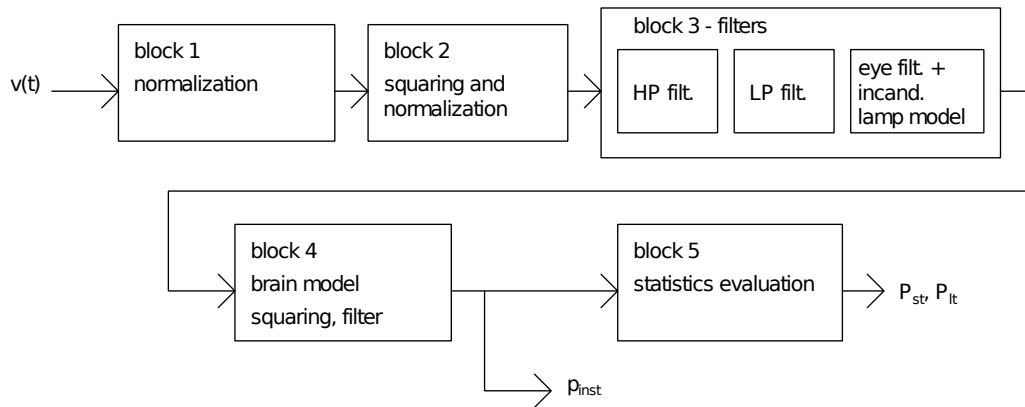
Figure A.1: The diagram of the IEC flickermeter
