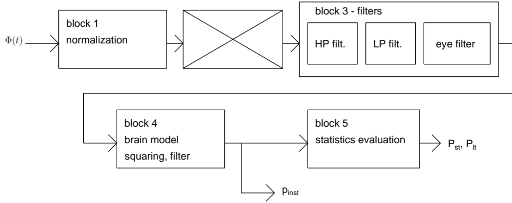
Figure B.1: A diagram of an objective flickermeter
