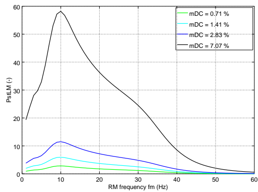
(b) LED 1—rectangular modulation
