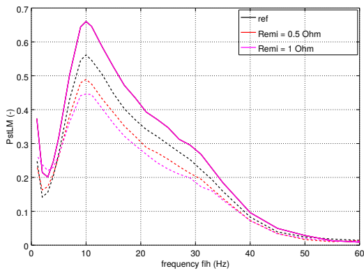
(c) Several values of R_{EMI}
