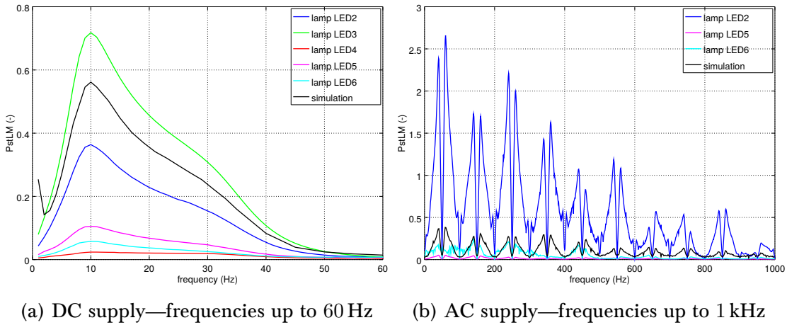
Figure 7.12: Active driver—model verification, frequency domain
