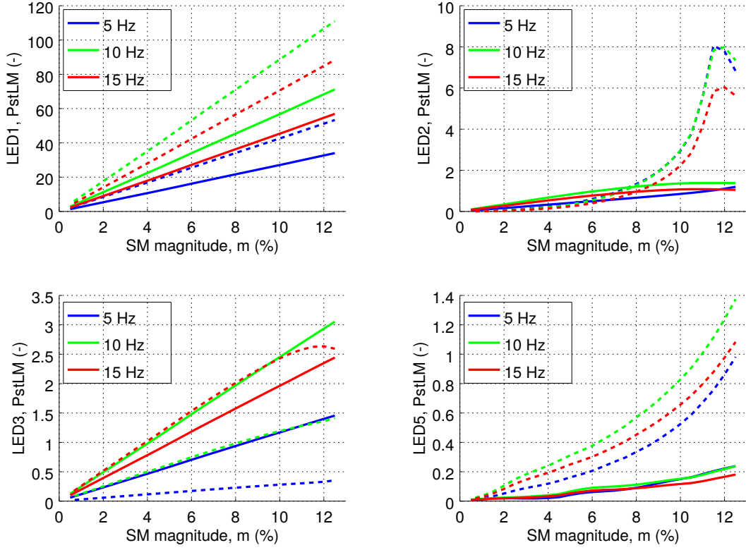
Figure 6.21: m\text{-}P_{\text{st}}^{\text{LM}} characteristics of the analysed lamps; dotted lines—with DB, solid lines—without DB
