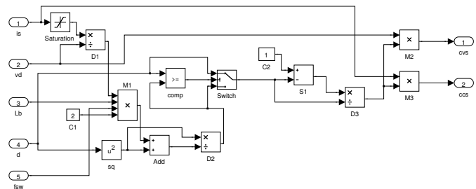
(c) The averaged switch model—calculation of the equivalent duty ratio \tilde{D} according to Eq. (7.9)
