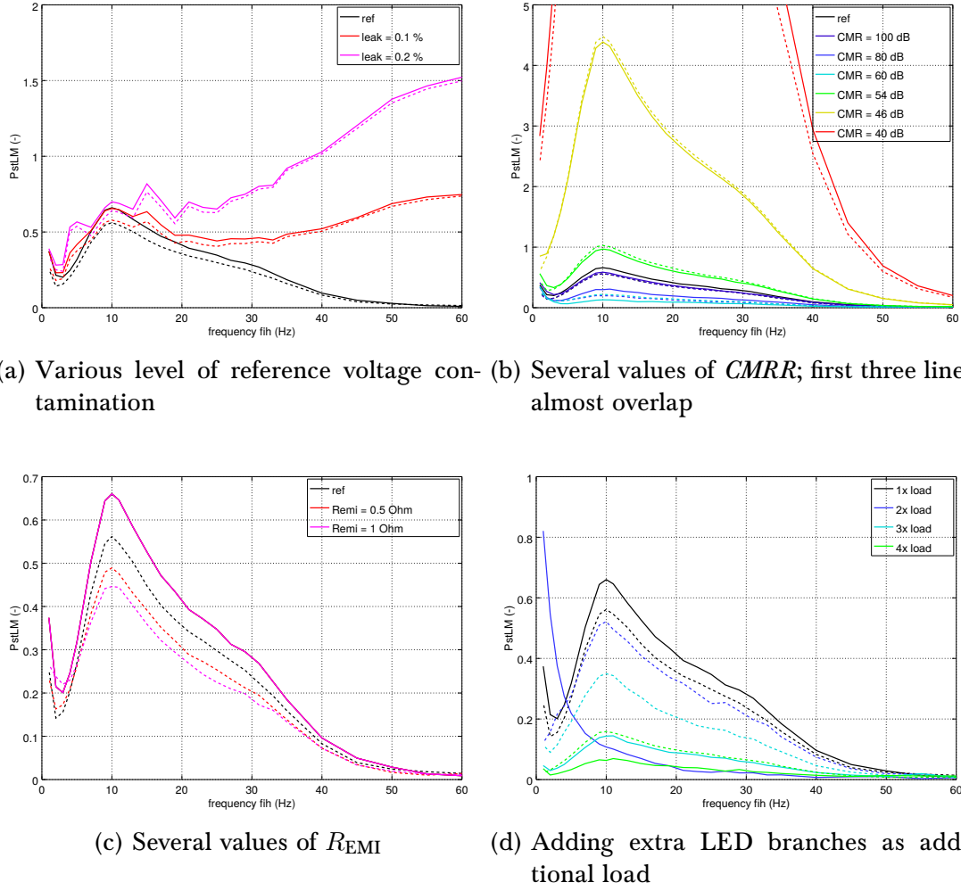
Figure 7.15: Simulated P_{st}^{LM} with various changes to the model; dotted line with DB, solid line without DB
