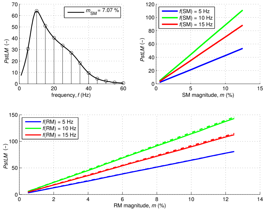
(a) LED1 (passive driver); approximation is successful because the m-P_{st}^{LM} response is linear, the error is less than 5 %
