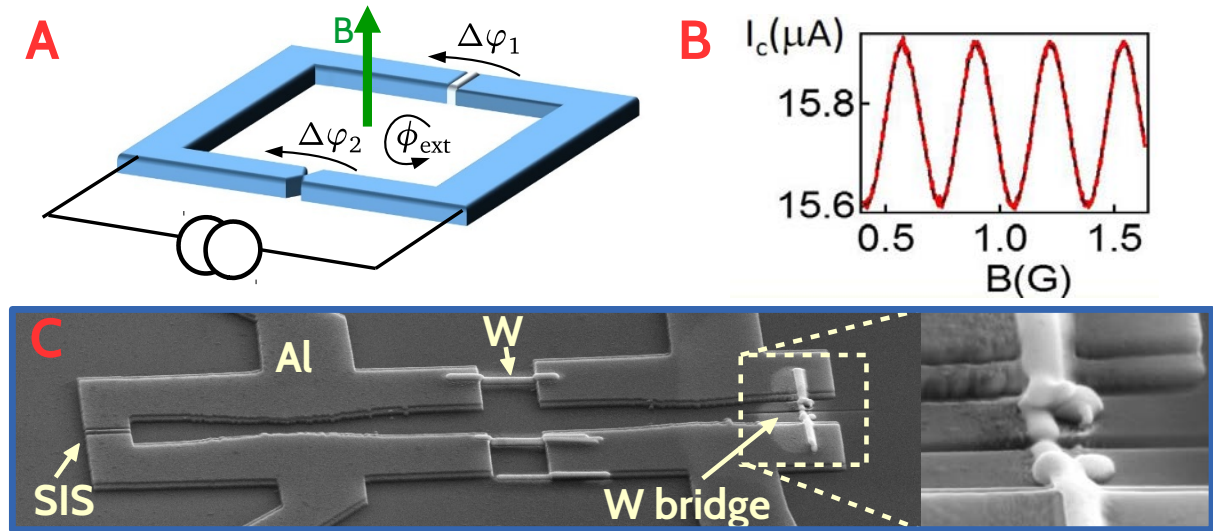
Figure 3.3: Proof of principle of the current phase relation measurement using an asymmetric SQUID technique with a W constriction as the reference junction. A : Schematics of the asymmetric SQUID. The superconducting tunnel junction is symbolized by the white junction and the W constriction is located opposite to it. B Critical current of the asymmetric SQUID. Red : measurement after performing the \beta correction. Black dashed line : sinus function fit. C : SEM image of the measured SQUID. The long part of the SQUID is 20 microns long. Inset : Zoom of the W constriction.
