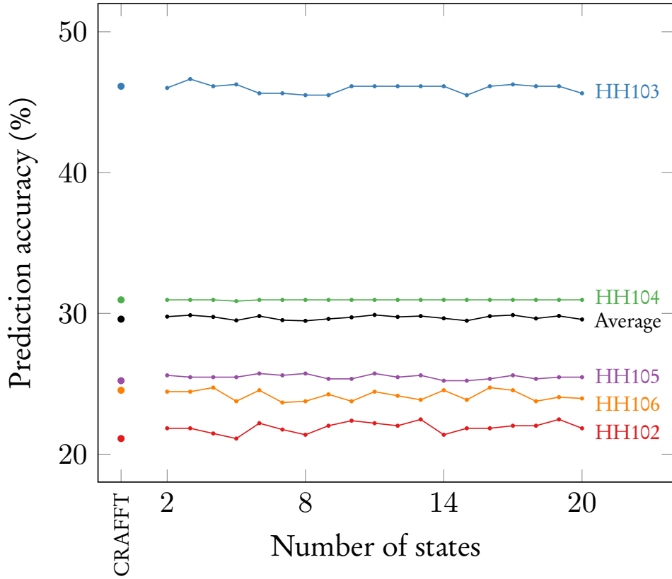
Figure 4.10 – Prediction accuracy of the latent CSCRAFT DBN with varying number of states for the latent cognitive state node on the CASAS datasets.
