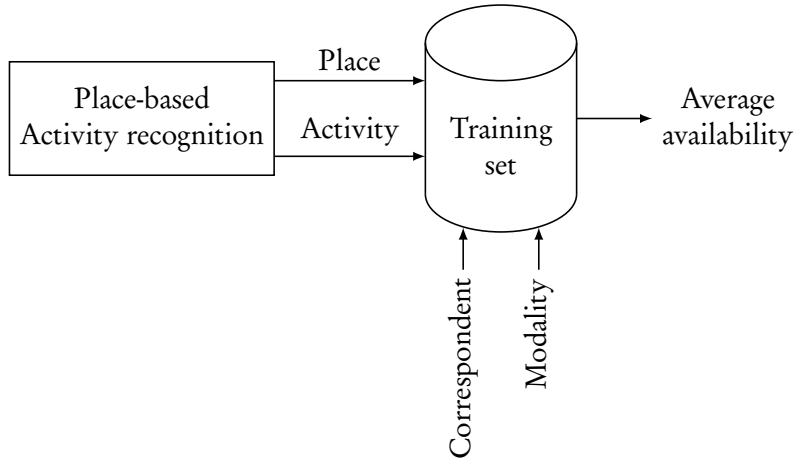
Figure 5.1 – Availability inference workflow.
