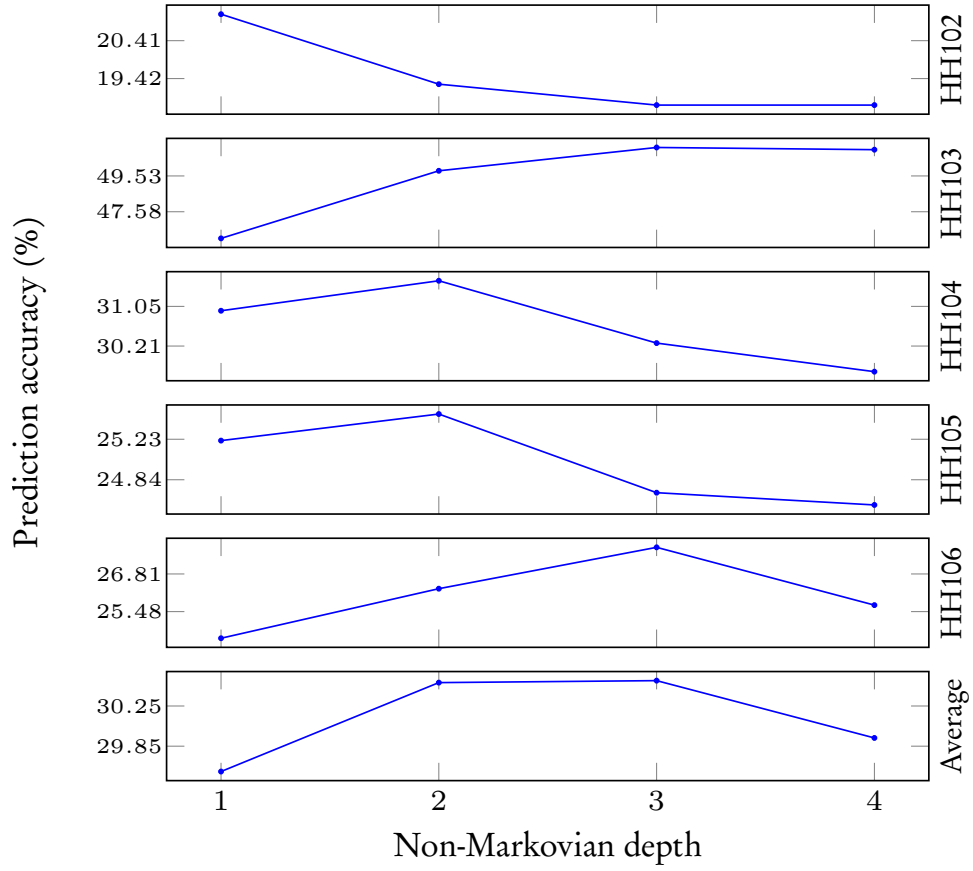
Figure 4.9 – Prediction accuracy of the NMCRAFT DBN with varying non-Markovian depth on the CASAS datasets.
