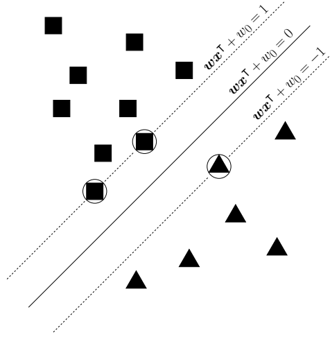
Figure 3.7 – Maximum margin hyperplane on a 2-dimensional training set of 2 classes (squares and triangles), in a linearly separable case. The support vectors are circled.
