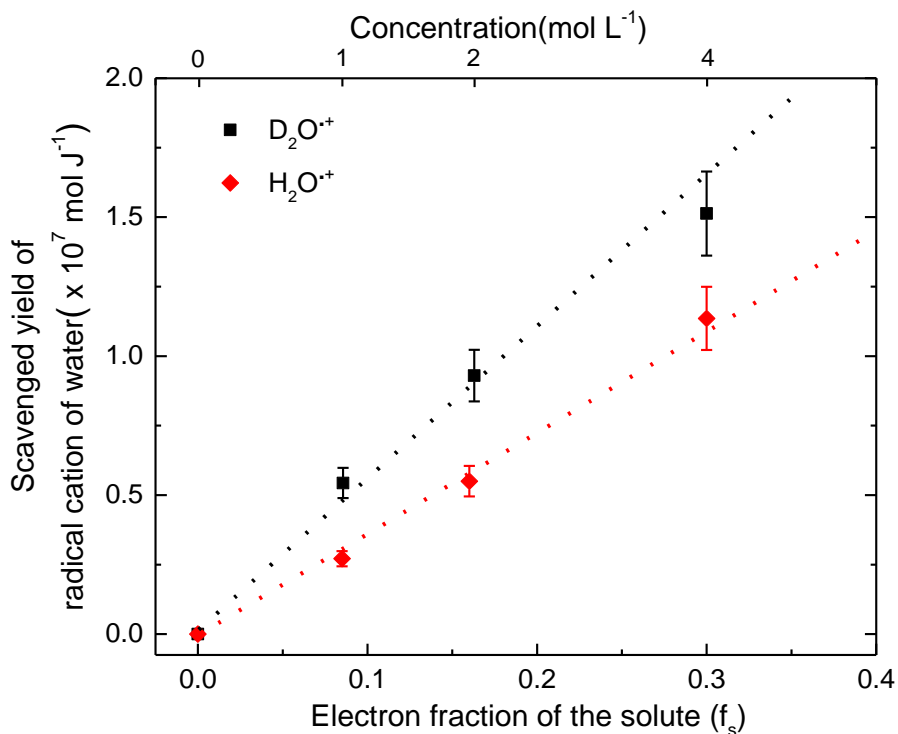
Figure 4.25 Yield of scavenged radical cation ( \text{H}_2\text{O}^+ and \text{D}_2\text{O}^+ ).
