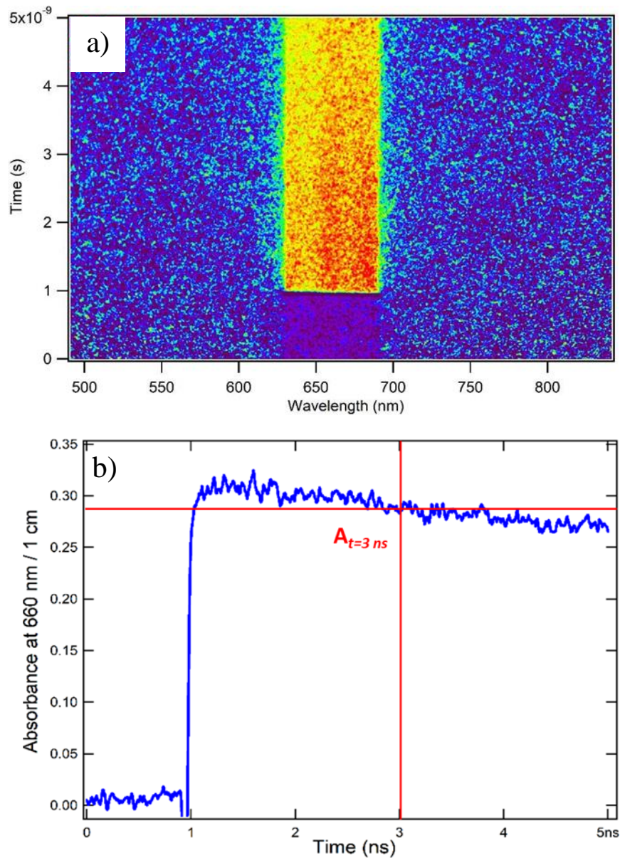
Figure 2.23 The decay of solvated electron in H 2 O recorded by streak camera. a) Image in 2D form, and b) Kinetics at 660 nm.
