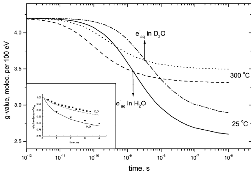
Figure 3.2 Simulation of the time dependent decay of solvated electron in H 2 O and D 2 O under low LET radiolysis at 25 °C and 300 °C, respectively. 9 The inset was experimental results from C. D. Jonah et al. 2, 10
