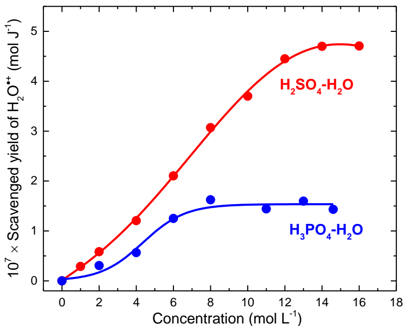
Figure 4.14 End of pulse radiolytic yield of scavenged radical cation \text{H}_2\text{O}^{+\bullet} in aqueous sulfuric and phosphoric acid solutions (Revised). Performed by Ma. et al 49 .
