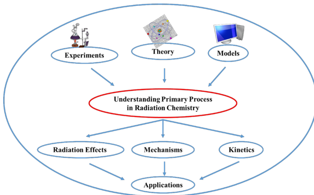
Figure 1.1 The key role of fundamental studies in radiation chemistry
