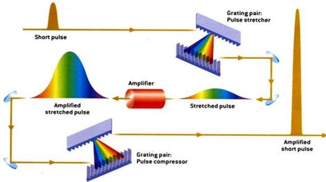
Figure 2.11 The principle of chirped pulse amplification for femtosecond laser.
