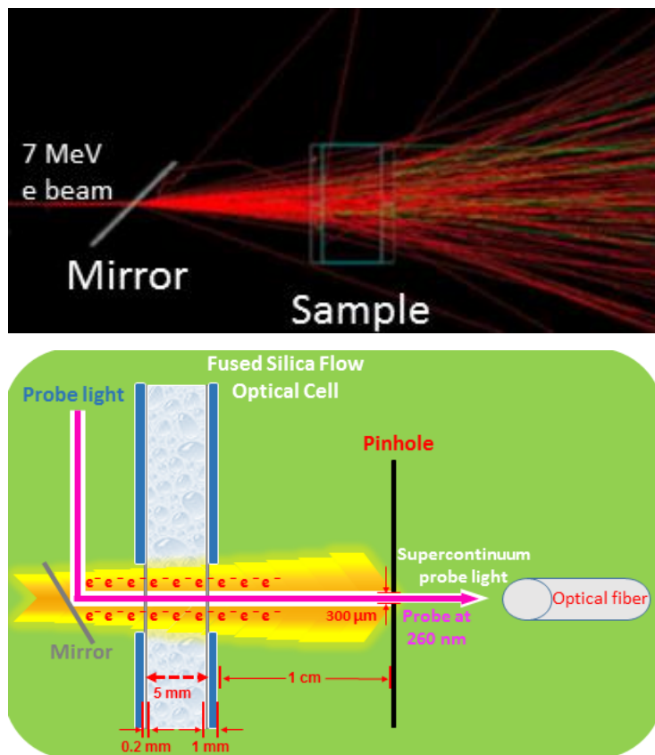
Figure 3.23 Top: Simulations of electron beam propagation and its scattering by the mirror, air, cell windows and the sample. Bottom: Scheme of the setup for measuring the yield of OD^{\bullet} at 260 nm by insuring that the supercontinuum probe light and 260 nm probe the same irradiated volume. For that purpose, a pinhole with 300 \mu\text{m} diameter is placed 1 cm after the sample.
