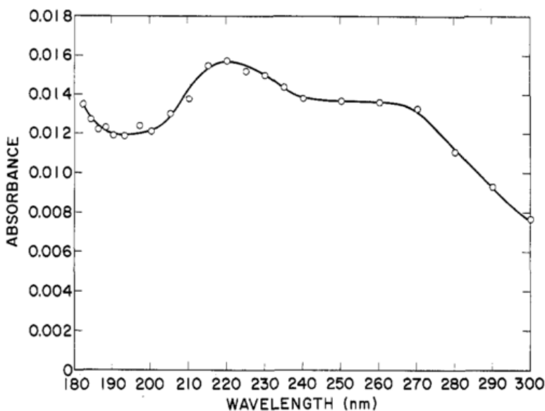
Figure 3.20 Transient absorption spectra in irradiated Suprasil sample of 1 mm thickness. Measured immediately after 3 \mu s electron pulse by Nielsen et al. 20 Dose per pulse is 240 Gy per pulse.
