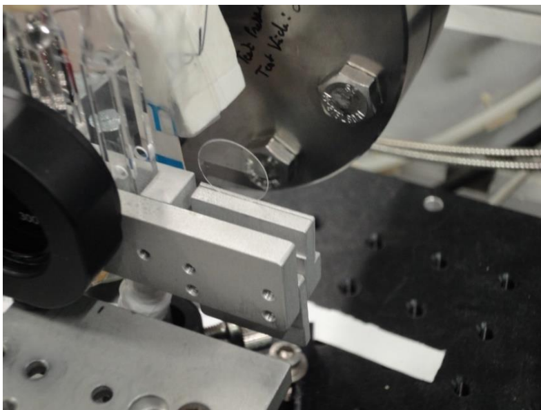
Figure 3.24 Measurement with an empty FSOFC and a plate of 200 \mu\text{m} under the same condition.
