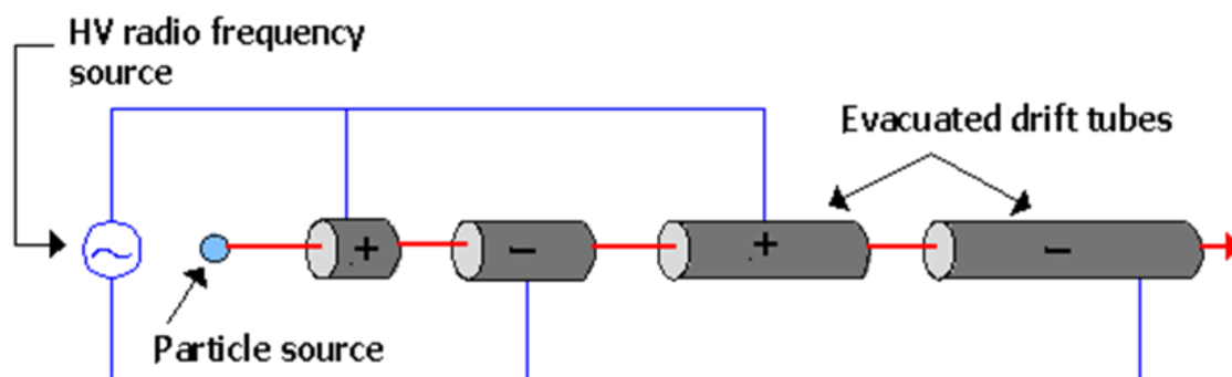
Figure 2.6 Diagram of LINAC.
