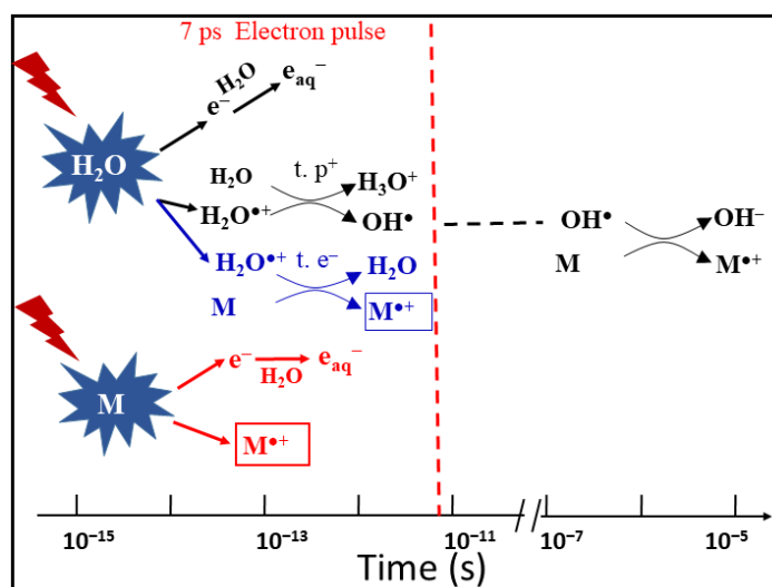
Figure 4.3 Schematic description of the reactions occurring in solutions containing a solute M at high concentration. At subpicosecond time scales involving proton transfer (t. p + , black), direct ionizing of solutes M (red), ultrafast electron transfer (t.e - , blue) and electron relaxation. Picosecond electron pulse radiolysis is ready to observe the formation of \text{M}^{\bullet+} within the pulse. The oxidation of M by \text{OH}^\bullet radical takes place at longer time, which does not affect our observation. 19
