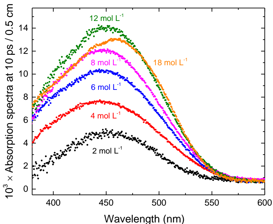
Figure 4.17 Example of the transient absorption spectra of the sulfate radical ( \text{HSO}_4^\bullet and \text{SO}_4^{\bullet-} ) recorded at 10 ps in \text{D}_2\text{SO}_4 at different concentration. The contribution of solvated electron and the transient induced in the optical cell are subtracted from the observed signal. The dose was 42.5 Gy per pulse.
