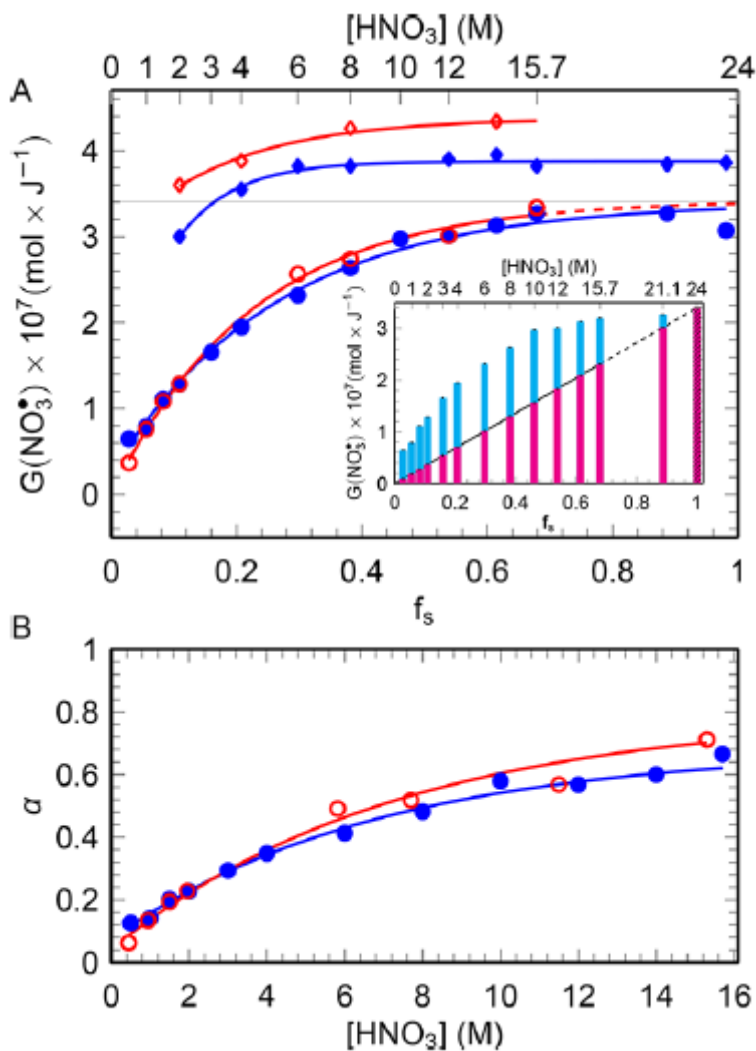
Figure 4.11 (A) Observed radiolytic yields of \text{NO}_3^\bullet after the 7 ps electron pulse as a function of the solvent electron fraction in the investigated solutions at 22.5 °C (blue) and 80 °C (red), and the maximum yield of \text{NO}_3^\bullet measured at different concentrations. For the lowest concentrations the presented yields are measured after the decay of the solvated electron. Inset: Observed radiolytic yields of \text{NO}_3^\bullet after the 7ps electron pulse as a function of the solvent fraction in the investigated solutions at 22.5 °C, displaying the contribution of direct effects (red) and indirect effects (blue) to the observed yield. (B) Contribution of the ultrafast indirect effect (value of \alpha ) to the observed \text{NO}_3^\bullet radiolytic yields as a function of the investigated solutions concentration at 22.5 °C (blue) and 80 °C (red). The work was performed by Musat et al. 10
