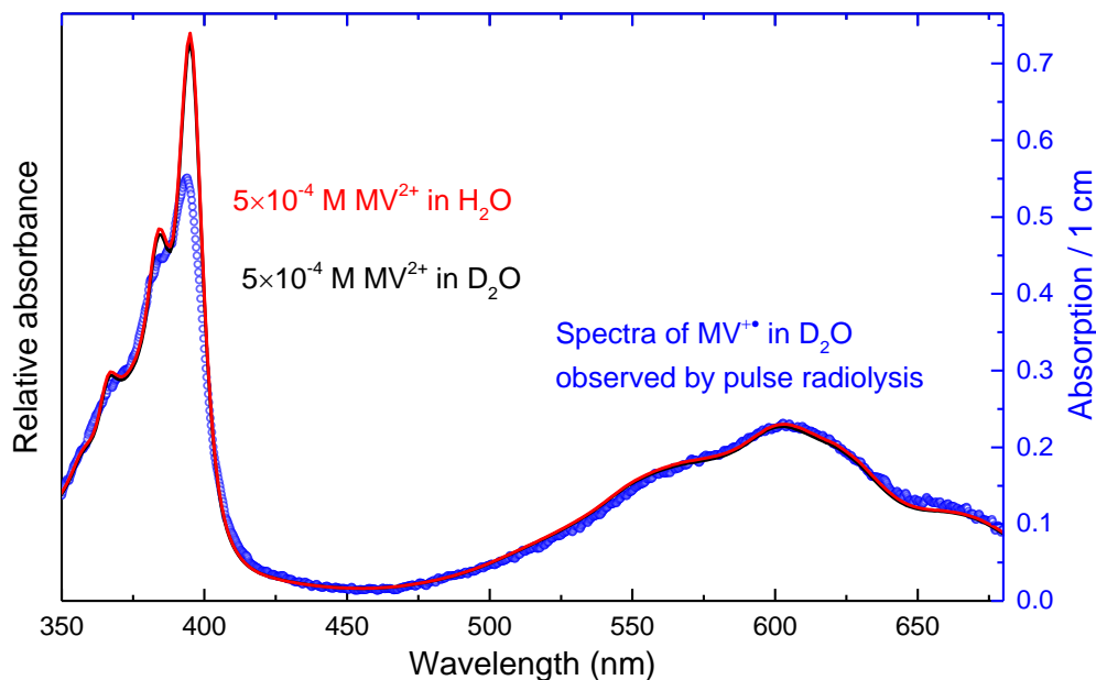
Figure 3.7 Left axis: UV-Visible absorption spectra of MV^{2+} in two solutions (containing 5 \times 10^{-4} M MV^{2+} , 0.2 M isopropanol and 2% acetone in H_2O and D_2O , respectively) after irradiation with \gamma source. Isopropanol was used to scavenge hydroxyl radical and Acetone was used to slow down the reduction of MV^{2+} . The dose is 600 Gy. Right axis: The spectra of MV^{2+} detected by streak camera for a D_2O sample containing 5.5 \times 10^{-4} mol L^{-1} methyl viologena and 0.5 M tert-butanol (to scavenge OD^{\bullet} ). The dose was 54 Gy per pulse. It is clear that the spectra of MV^{2+} in D_2O observed by streak camera at ELYSE from 400 to 650 nm fits well with that obtained by \gamma source. The intensity of the absorption band from 350 to 400 nm measured by Streak Camera is lower than that measured by \gamma source because the resolution of streak camera is not enough high to detect the narrow peak of MV^{2+} around 394 nm.
