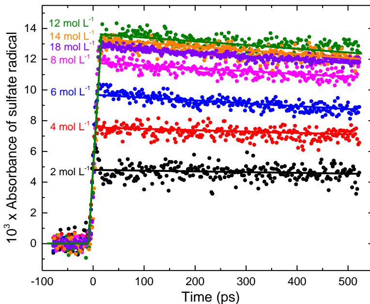
Figure 4.19 Kinetics of sulfate radical ( \text{SO}_4^{\bullet-} or \text{HSO}_4^\bullet ) on absorption maximum wavelength. The contribution of solvated electron has been subtracted from the signal. The dose per pulse was 42.5 Gy.
