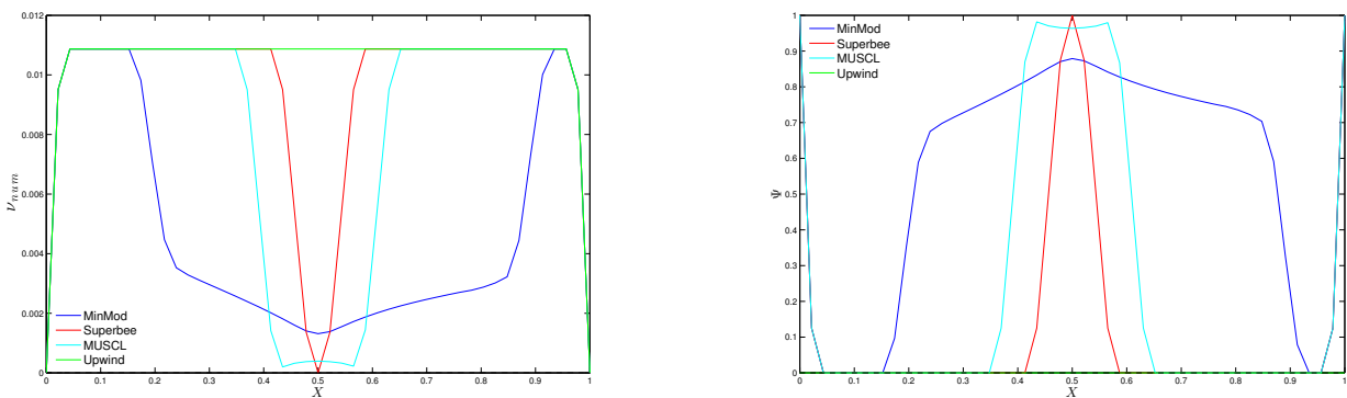
(a) Numerical Viscosity
