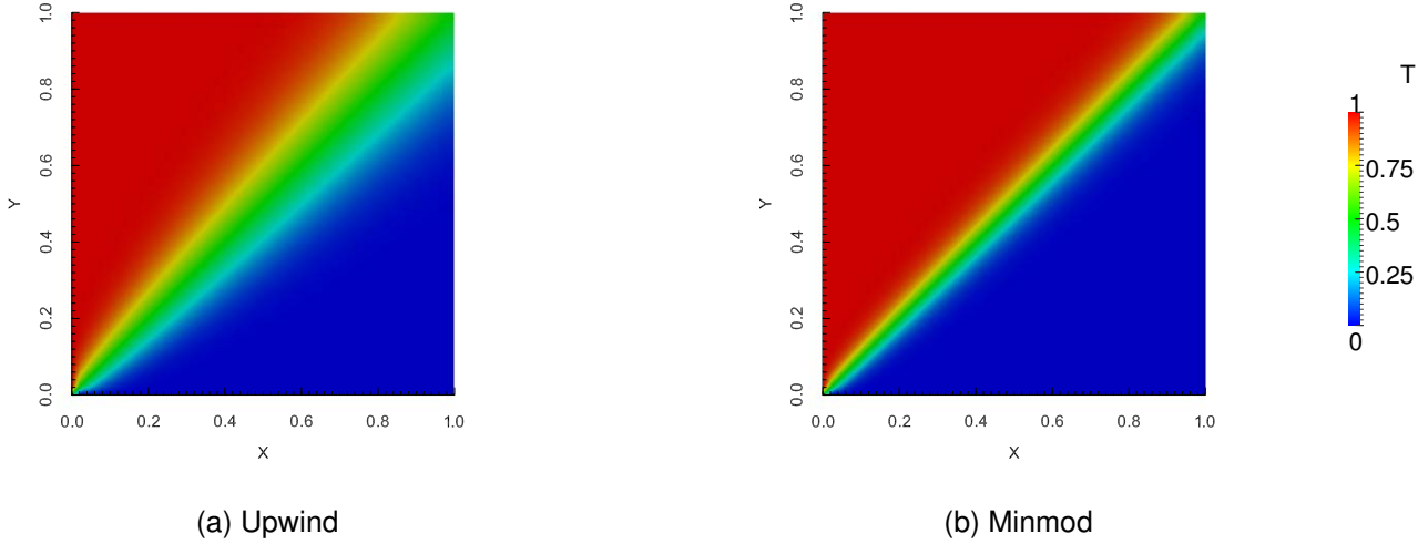
FIGURE A.1 – Plot of the solution for the 2D Step profile problem, left : Upwind, right : minMod
