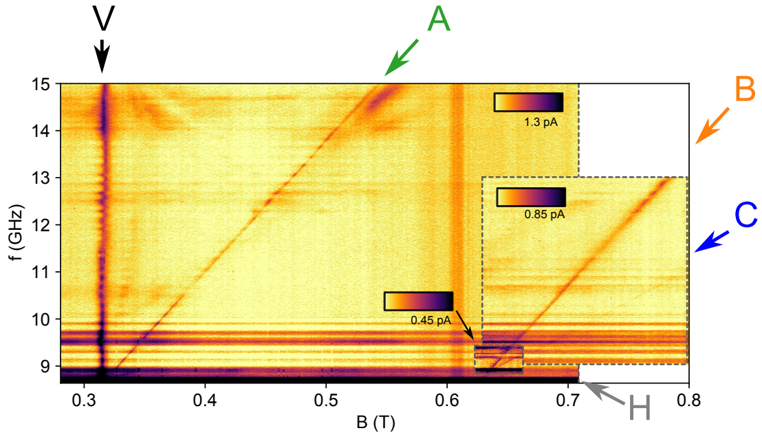
Figure 4.4: Experimental EDSR map. The measured current is plotted as a function of the frequency of the microwave signal and of the magnetic field amplitude. The relevant lines are labelled A, B, C, V, H. Adapted from Ref. [53].
