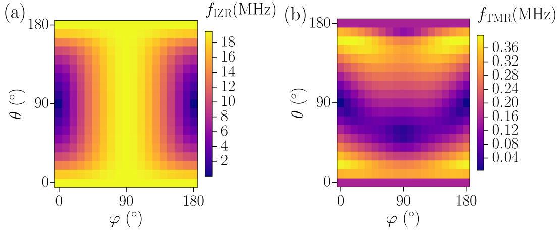
Figure 6.18: Rabi frequency cartography for a state located under between the two gates, at constant Zeeman energy (9 GHz), with tensile in-plane strain, without disorder. (a) IZ-EDSR contribution (b) g -TMR contribution.
