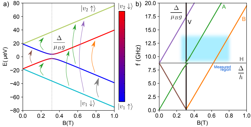
Figure 4.6: (a) Energy diagram of the first four states as a function of the magnetic field amplitude. An avoided crossing is supposed at B = \Delta/(g\mu_B) . The energy of |v_1 \downarrow\rangle is in light blue, and the energy of |v_2 \uparrow\rangle is in green. The spin and valley composition of the hybridized states is quantified by a colour scale. (b) Sketch of the possible transitions noted by the arrows in (a). The experimentally measured region is in light blue.
