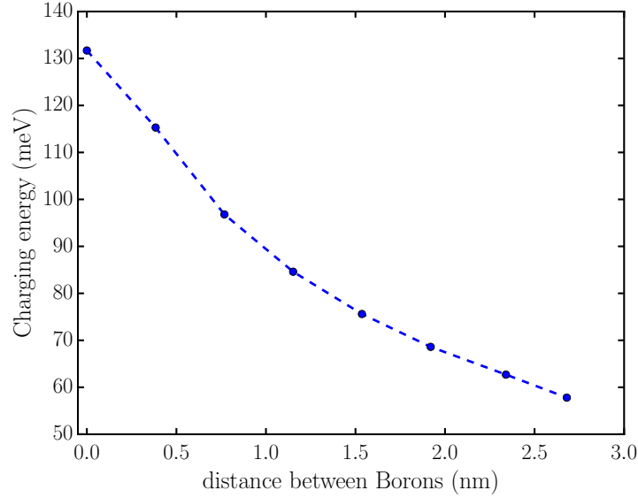
Figure 3.9: Charging energy of states bound to a cluster of two Boron impurities as a function of the distance between them.
