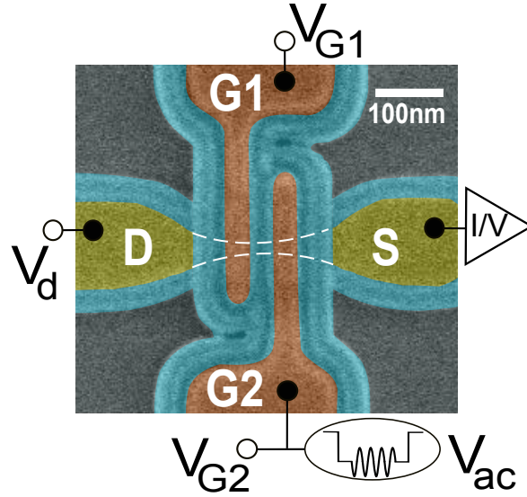
Figure 6.1: Scanning electron micrograph of a device similar to the one measured, with false colors. The white dashed lines outline the Si nanowire, 25 nm large and 8 nm thick, constituting the channel between S and D (yellow regions). Gates G1, G2 (in brown) are 35 nm long and separated by SiN 3 spacers (cyan); microwave bursts are applied to G2. The x , y , z axes define the lab frame. From Ref. [100].
