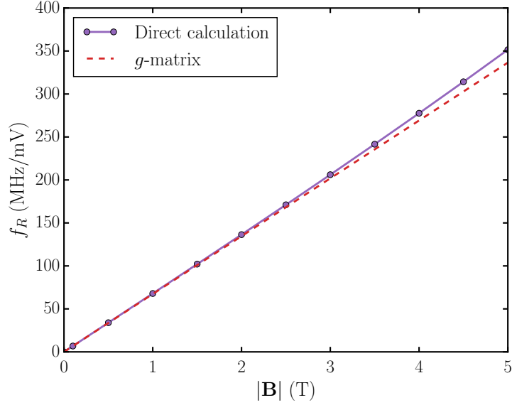
Figure 6.14: Rabi frequency from direct calculation and g -matrix formalism, as a function of magnetic field amplitude, with a field along \mathbf{x} + \mathbf{z} .
