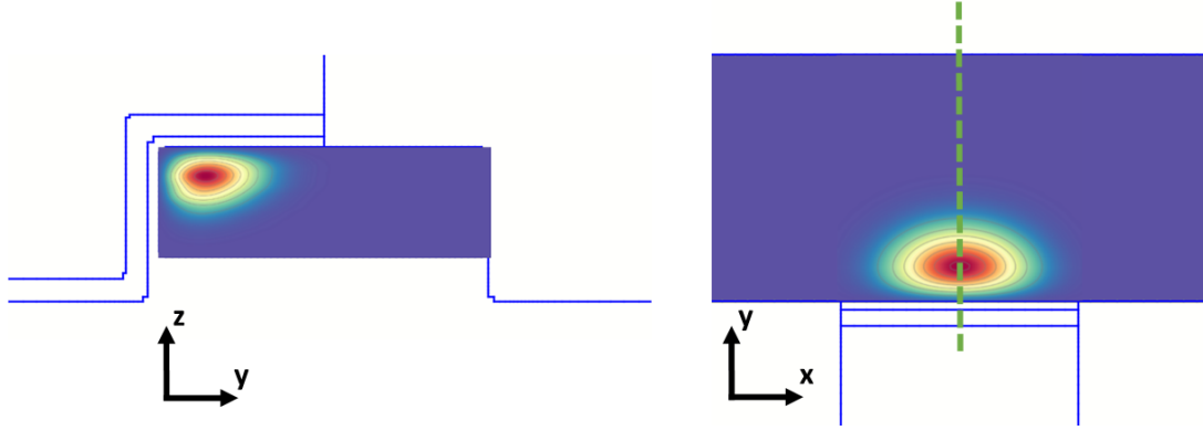
Figure 4.14: Symmetry plane in half-gated device. The mirror planes of the wavefunction are given by the dotted green lines.
