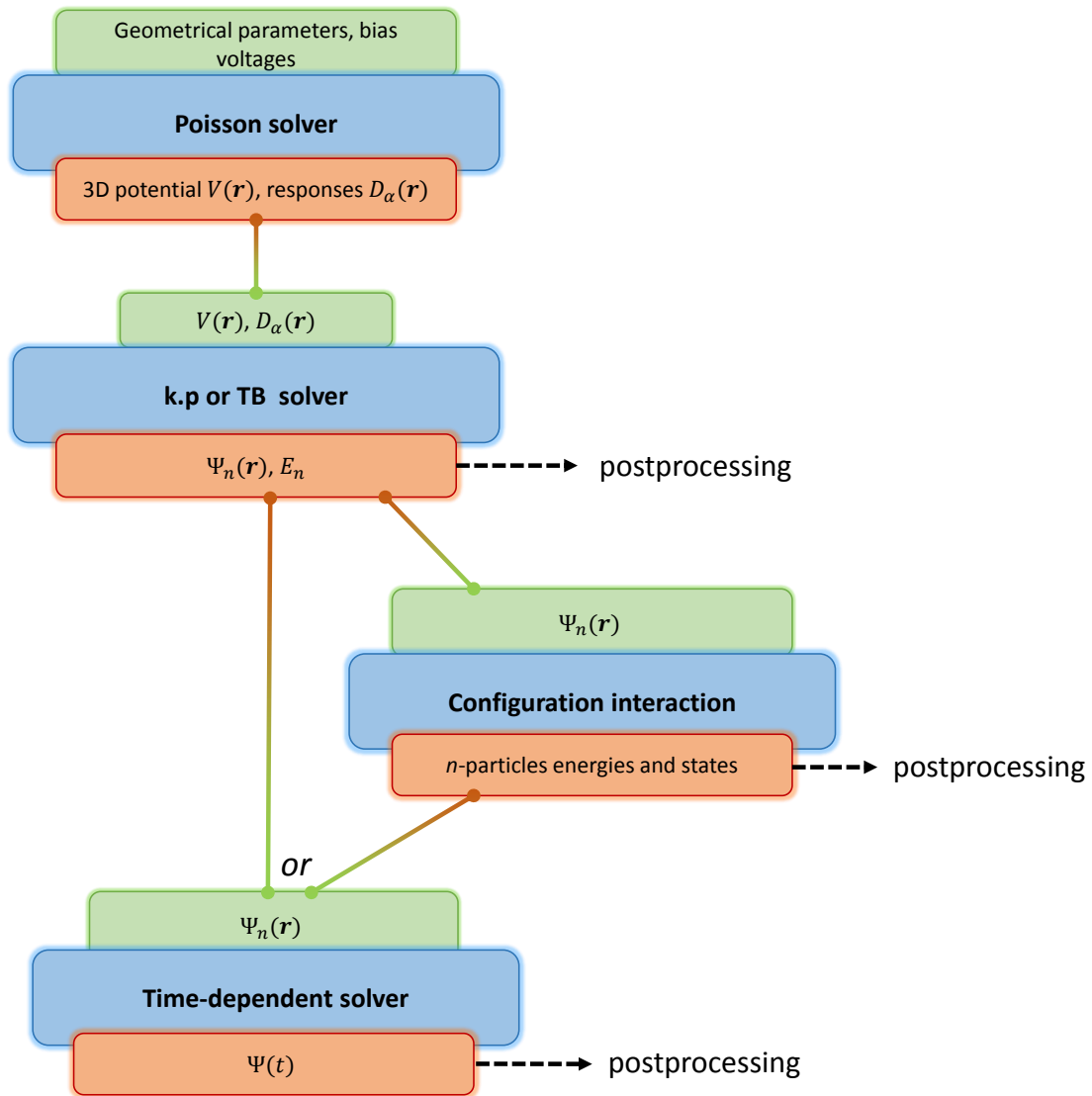
Figure 3.1: Workflow of possible simulations. The solvers are in blue, their inputs are in green and their outputs are in red.
