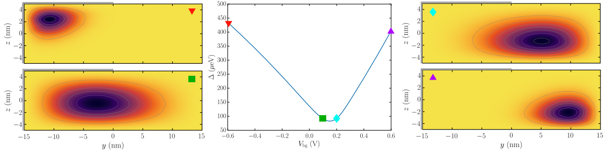
Figure 5.2: (Central panel) valley splitting as a function of backgate potential ( V_g = 0.1 V). The valley splitting shows a minimum \Delta^{\min} = 83 \mu\text{eV} at V_{\text{bg}}^{\min} = 0.15 V. (Lateral panels) The squared wavefunction of the ground state |0\rangle is plotted in the (yz) cross section, at the four bias points labelled by the symbols. The thick gray lines outline the position of the front gate.
