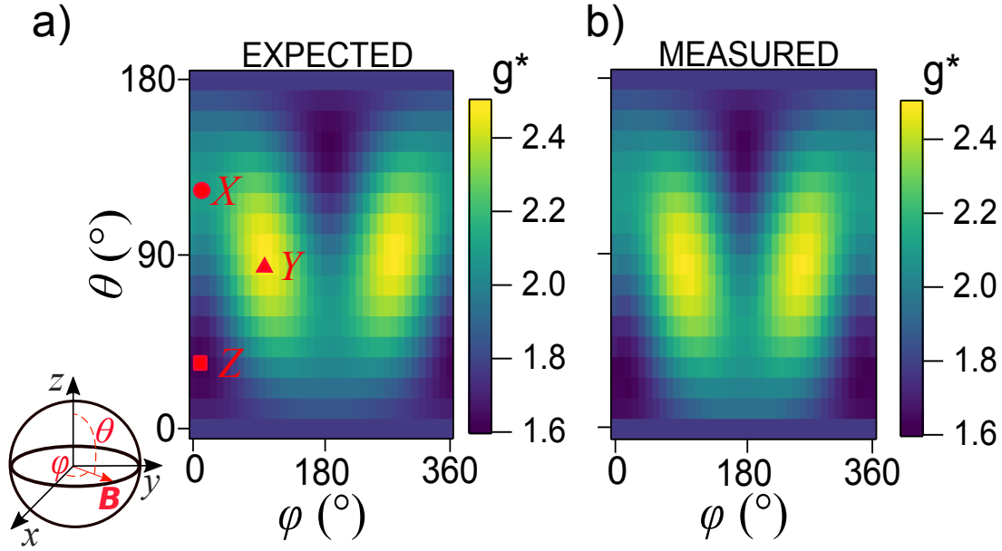
Figure 6.8: (a) g^* as a function of the field angles \theta and \varphi , reconstructed from the six values of g^* defining the Zeeman tensor. (b) Experimental cartography of g^* , same as Fig. 6.5b), for comparison. From Ref. [100].
