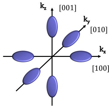
Figure 2.2: Iso-energy surfaces of the six valleys of silicon.
