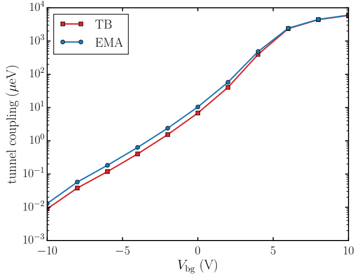
Figure 3.7: Tunnel coupling between the two dots of the face-to-face device as a function of V_{bg} , calculated using TB and EMA.
