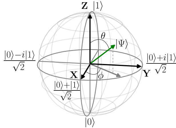
Figure 1.1: Bloch sphere representation of a two-level quantum state.
