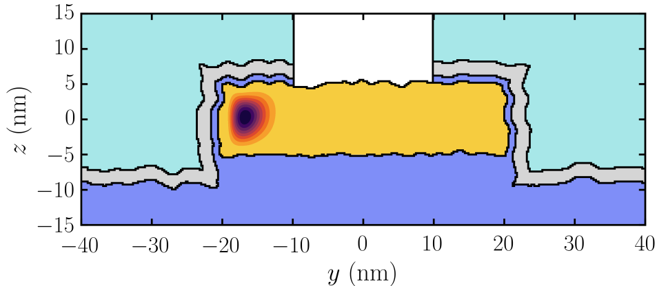
Figure 3.6: Iso-surfaces of the squared wavefunction of a hole obtained from 6-bands \mathbf{k}\cdot\mathbf{p} in the yz -plane at x = 0 . The same colors have been used for the materials as in Fig. 3.2.
