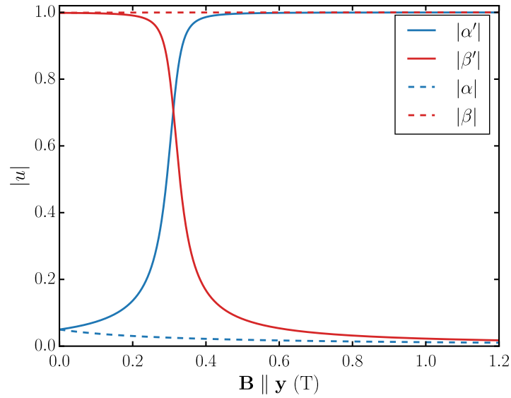
Figure 4.12: Norm of the coefficients \alpha , \alpha' , \beta , \beta' as a function of magnetic field amplitude.
