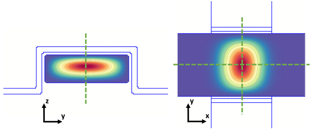
Figure 4.15: Symmetry plane in trigate device. The mirror planes of the wavefunction are given by the dotted green lines.
