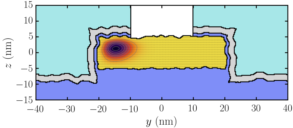
Figure 3.5: Cross-section of the squared TB wavefunction of an electron in the yz -plane at x = 0 , calculated with the potential of Fig. 3.3b. The iso-probability surfaces are in gray. The Si atoms are the black dots, and the same colors have been used for the other materials as in Fig. 3.2.
