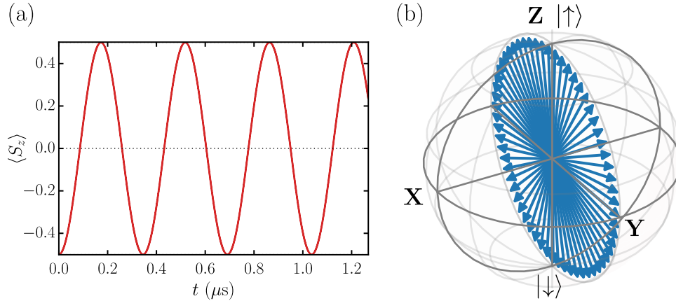
Figure 1.3: (a) Expected value of the spin along z , exhibiting Rabi oscillations. (b) Representation of the state evolution (in blue) in the rotating Bloch sphere.
