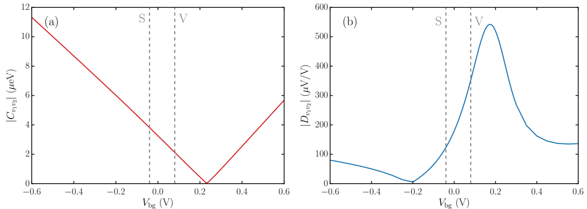
Figure 5.5: (a) Spin-orbit and (b) dipolar inter-valley matrix elements as a function of V_{bg} . The gray dashed lines highlight the spin and valley mode arbitrarily chosen for the qubit operation.
