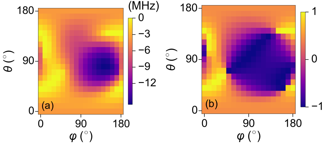
Figure 6.12: (a) Map of |\mathbf{f}_R| - |\mathbf{f}_{\text{IZR}}| - |\mathbf{f}_{\text{TMR}}| as a function of the orientation of the magnetic field. (b) Map of \cos(\theta_Z) as a function of the orientation of the magnetic field, where \theta_Z is the angle between \mathbf{f}_{\text{IZR}} and \mathbf{f}_{\text{TMR}} .
