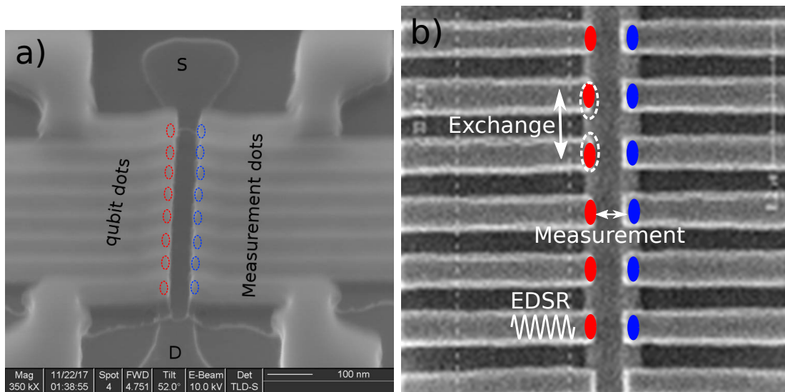
Figure 2.11: (a) SEM tilted top view of an array of face-to-face devices on a single nanowire. Schematics of the dots approximate position are given in red for the qubit dots and in blue for the measurement dots. (b) SEM top view with same color code. The possible operations (spin measurement, single spin control via EDSR, and exchange interaction) are outlined in white.
