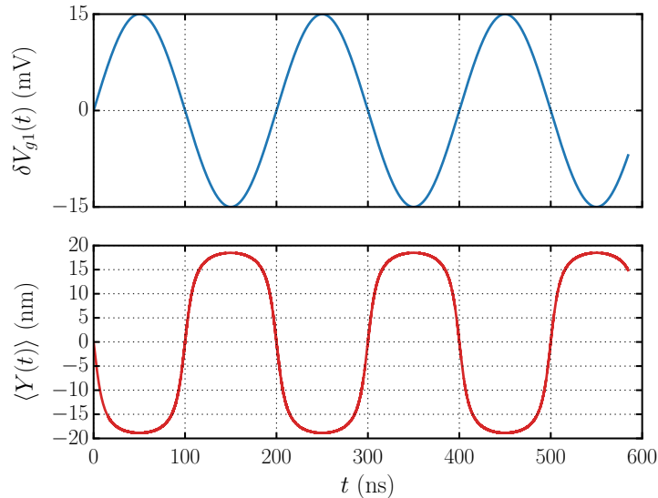
Figure 3.10: Signal on gate 1 \delta V_{g1}(t) and average position \langle Y(t) \rangle as a function of time.
