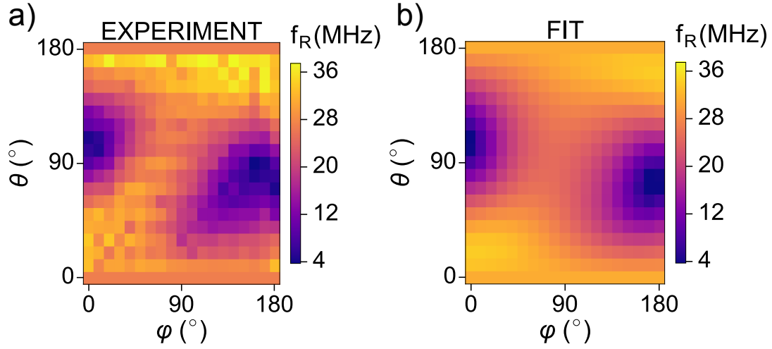
Figure 6.10: (a) Measured angular dependence of the Rabi frequency, as in Fig. 6.5a. (b) Analogous map obtained from the fit of (a) with Eq. 6.13.
