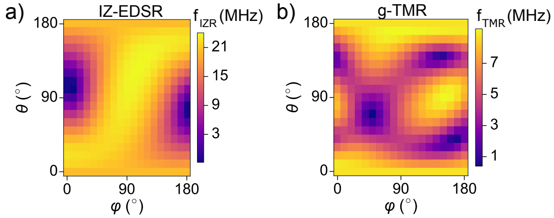
Figure 6.11: (a) IZ-EDSR and (b) g -TMR contributions to f_R .
