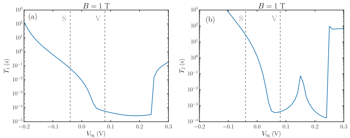
Figure 5.9: (a) Relaxation time including phonons and Johnson-Nyquist noises as a function of V_{\text{bg}} (b) Dephasing time for Johnson-Nyquist noise T_{2,jn}^* as a function of V_{\text{bg}} . For both panels B = 1 T, and the vertical gray dotted lines mark the spin and valley operation points of part 5.2.
