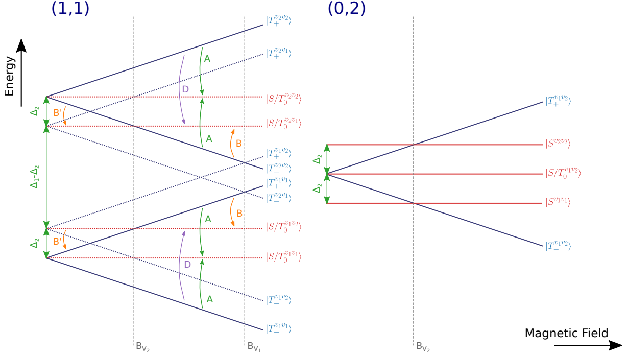
Figure B.1: Scheme of the energy levels for a system with two dots, filled with two electrons in the (1, 1) and (0, 2) charge configurations, as a function of magnetic field. We assume different valley splittings in the two dots (respectively \Delta_1 > \Delta_2 ). Triplets in the (0, 2) configurations with two electrons in the same valley are not represented, since they are energetically far away.
