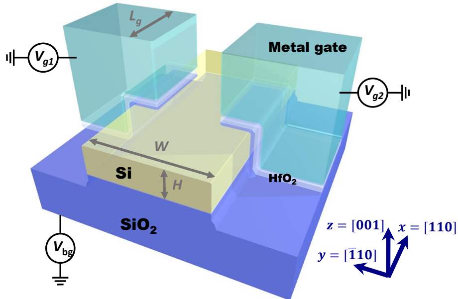
Figure 3.2: Geometry of the "face-to-face" device. The silicon nanowire is in yellow, \text{HfO}_2 is in light gray, \text{SiO}_2 is in dark blue and the metal gates are in light blue. The buried \text{SiO}_2 lies on top of a Si substrate, not shown.
