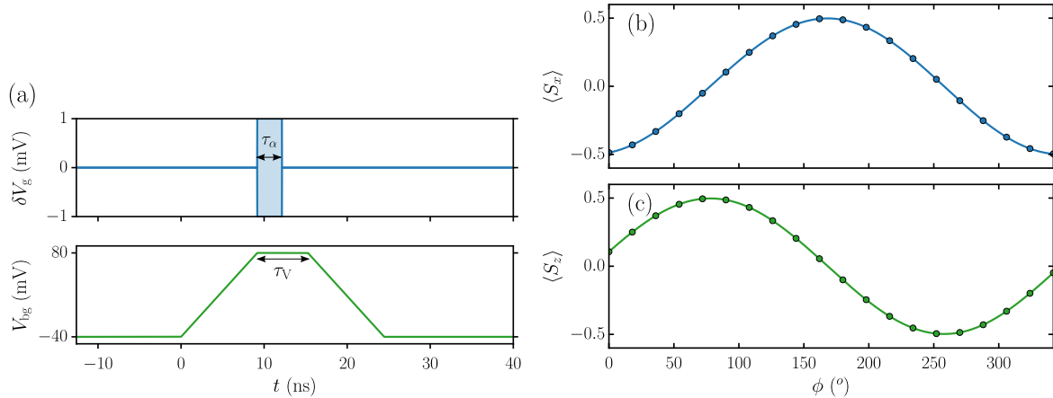
Figure 5.8: (a) Time series for a \pi/2 rotation from the |v_1 \downarrow\rangle state (b,c) Expectation value of S_x and S_z in the rotating Bloch sphere after that \pi/2 rotation as a function of the phase \phi of the driving RF signal.
