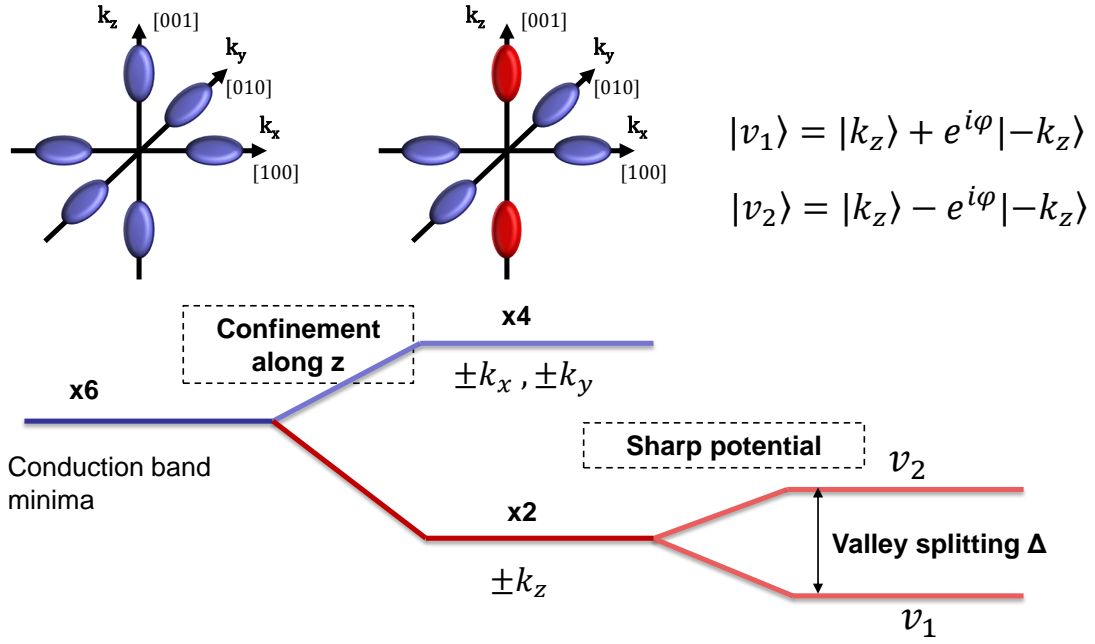
Figure 2.3: Schematic of the effect of the confinement and potential on the valley states and their degeneracy.
