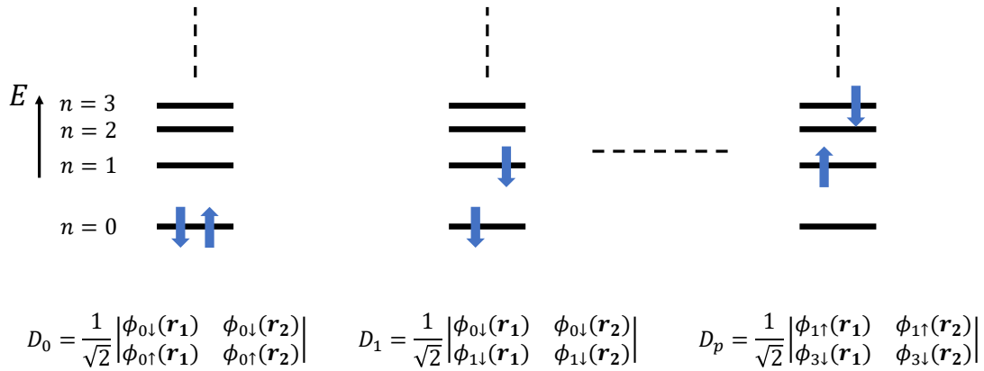
Figure 3.8: Illustrations of a few possible configurations for two-electrons states and their corresponding Slater determinants.
