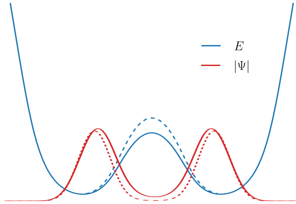
Figure 1.5: Sketch of two qubits coupled by exchange interaction. The height of the barrier between dots tunes t and thus J . Dotted lines correspond to the high-barrier regime ( t \simeq 0 ) and full lines to the low-barrier regime (finite t ).
