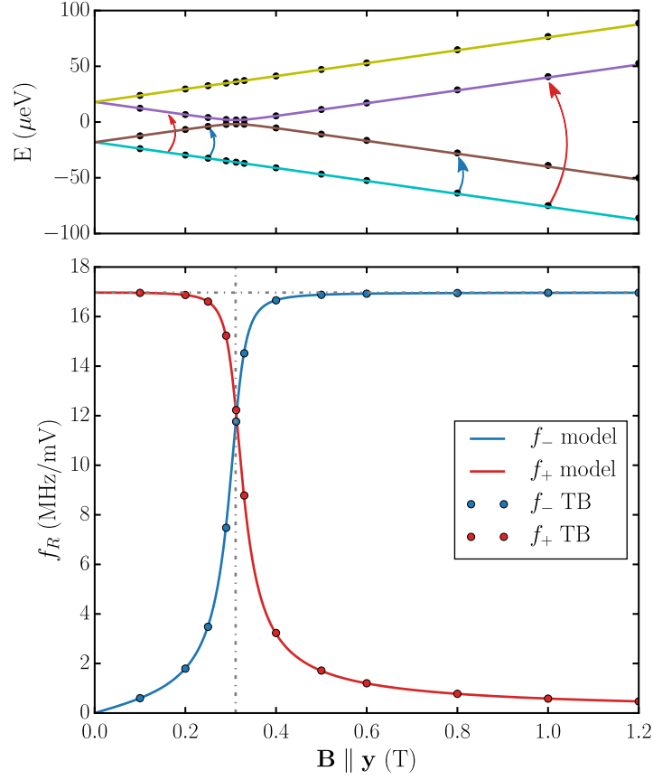
Figure 4.11: Energy levels and f_- and f_+ Rabi frequencies, corresponding to transitions between the ground state and respectively |\Psi'_-\rangle and |\Psi'_+\rangle , as highlighted by the blue ( f_- ) and red ( f_+ ) arrows. Dots are for direct tight-binding calculations, the solid lines are for the analytical model with C_{v_1v_2} = 1.8 , D_{v_1v_2} = 70 \mu\text{eV}/\text{V} and \Delta = 36 \mu\text{eV} , extracted from the TB calculations.
