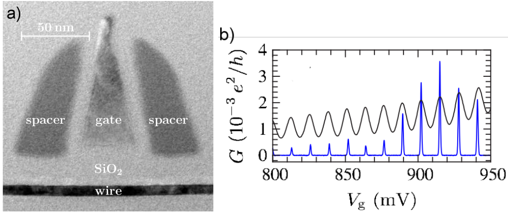
Figure 2.7: (a) MOSFET transistor with long spacers, isolating a quantum dot under the gate, capacitively coupled to the source and drain contacts. (b) Measured Coulomb oscillations at 4.2 K (black curve), and at 400 mK (blue curve). Adapted from Ref. [90].
