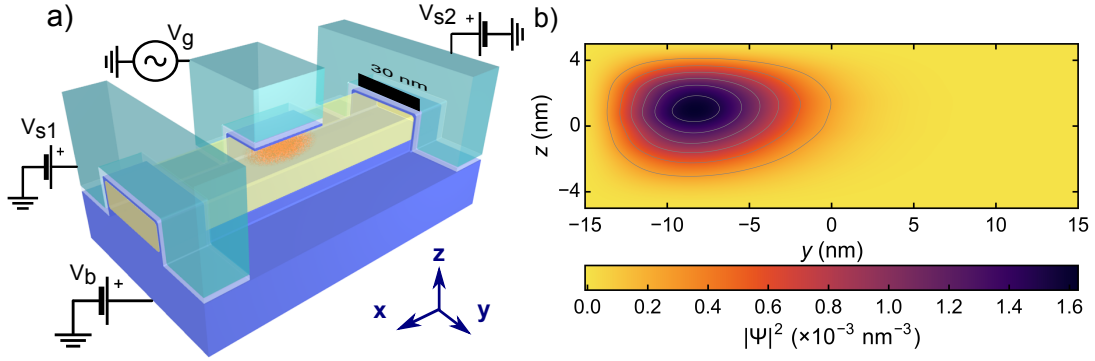
Figure 4.7: (a) Schematics of the device. The silicon nanowire is in yellow, \text{SiO}_2 in blue, \text{HfO}_2 in light gray and the gate are in dark green. The squared wavefunction is schematized in orange. (b) Cross-section of the squared wavefunction in the (yz) plane, computed with tight-binding.
