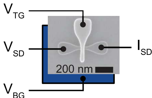
Figure 5.15: Device measured by David Ibberson at Hitachi Cambridge. From Ref. [57].
