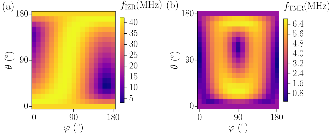
Figure 6.19: Rabi frequency cartography for a state located under between the two gates, at constant Zeeman energy (9 GHz), with tensile in-plane strain, with surface roughness and RCS charges with density n_{\text{RCS}} = 2 \times 10^{12} \text{ cm}^{-2} . (a) IZ-EDSR contribution (b) g -TMR contribution.
