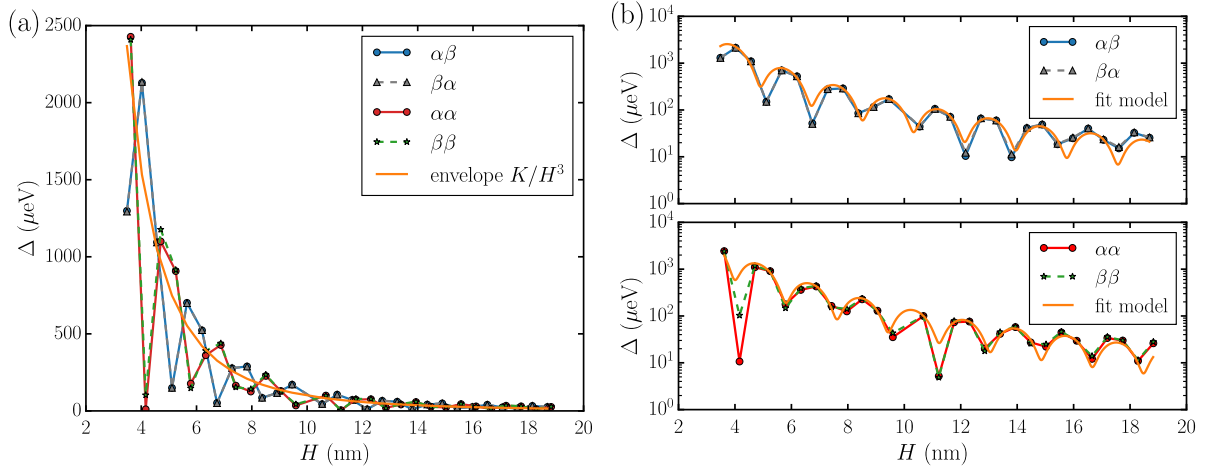
Figure 5.13: Valley splitting as function of the wire thickness H , for four sets of surface termination. The hydrogen bondings of top and bottom surfaces are either parallel (AA or BB) or orthogonal (AB or BA). (a) Linear scale, we fit the envelope from the model of Eq. 5.31. (b) Semilog scale, we fit the full model from Eq. 5.32 for orthogonal surface bondings (top panel) and parallel surface bondings (bottom panel).
