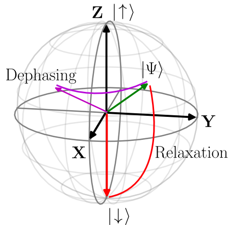
Figure 1.4: Bloch sphere of the spin qubit with sketch of a relaxation process (in red), and of a dephasing process (in violet).
