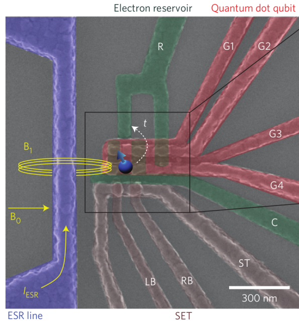
Figure 2.5: Silicon spin qubit. The set of gates define the quantum dot as well as a single electron transistor for readout. On the left, a microwave line is used to create an oscillating magnetic field for spin control. From Ref. [78]
