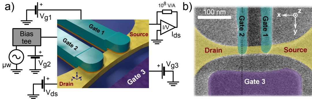
Figure 4.2: (a) Sketch of the sample and measurement setup. The silicon nanowire is coloured in yellow, the two top gates in green and the side gate in violet. The gate oxides are colored in orange and the buried oxide (BOX) is in blue. (b) Colourized device top view obtained by scanning electron microscopy before the deposition of the spacers of a device similar to the one used in the experiment, with same colour code. Adapted from Ref. [53]
