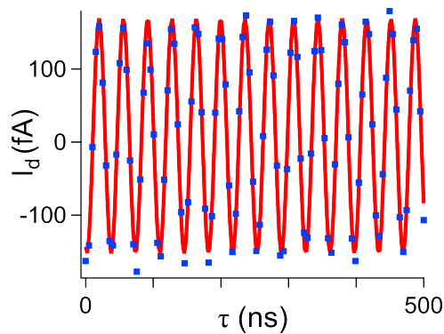
Figure 6.4: Rabi oscillations as a function of microwave burst time \tau for \mathbf{B} = (0, 0, -0.36) T. A current offset of 200 fA is subtracted for clarity. From Ref. [100].
