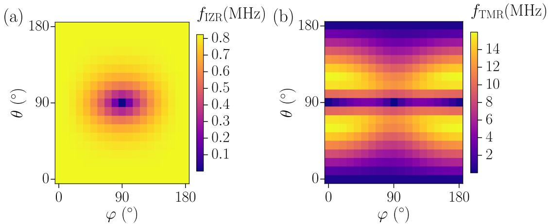
Figure 6.16: Rabi frequency cartography for a state located under the main gate, at constant Zeeman energy (9 GHz) (a) IZ-EDSR contribution (b) g -TMR contribution.
