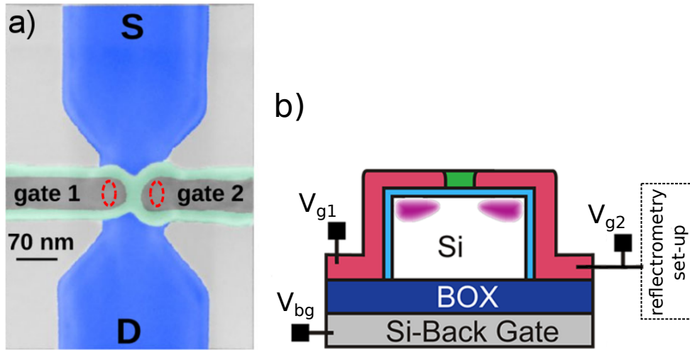
Figure 2.10: (a) Top view of a face-to-face device. The quantum dots approximate locations are shown by red lines. From Ref. [97]. (b) Schematic of the cross-section of the device and set-up. The position of the wavefunctions into the corner states is outlined in pink. Adapted from Ref. [94].
