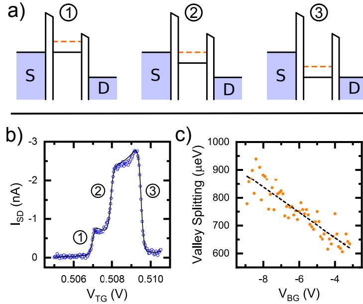
Figure 5.16: (a) Diagrams illustrating the respective alignment of the quantum dot and source and drain electrochemical levels at the three features observed in b). (b) Measured source-drain current (blue dots) in the first Coulomb oscillations at V_{BG} = -7.8 V. The black line is a fit considering that the system is in the sequential multi-level transport regime [43]. (c) Plot of valley splitting against V_{BG} with a best-fit line gradient of -45 \pm 3 \mu\text{eV}/\text{V} . From Ref. [57].
