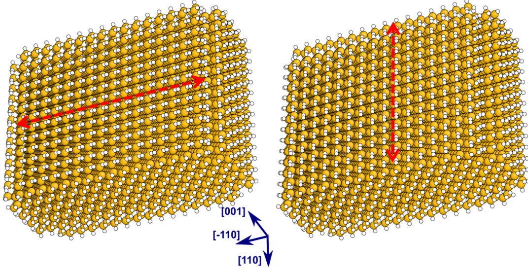
Figure 5.12: Small portion of a silicon nanowire passivated with hydrogen atoms. (Left) Type \alpha interface, the surface bondings are oriented perpendicularly to the wire direction. (Right) Type \beta interface, the surface bondings are oriented parallel to the wire direction.
