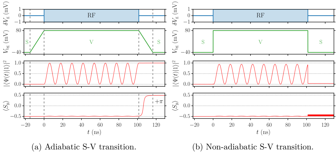
Figure 5.6: Time series for spin manipulations, monitored by the probability p(|1\rangle) to be in the |1\rangle state, and by the expectation value of the spin \langle S_y \rangle . Starting from the |0\rangle = |v_1 \downarrow\rangle state at point S, the qubit is pulsed (adiabatically in (a) or diabatically in (b)) to point V by the backgate, and the RF signal with resonant frequency is applied on the front gate to drive rotations between |0\rangle and |1\rangle . Once the RF signal is switched off, the qubit is brought back to point S (again adiabatically in (a) or diabatically in (b)).
