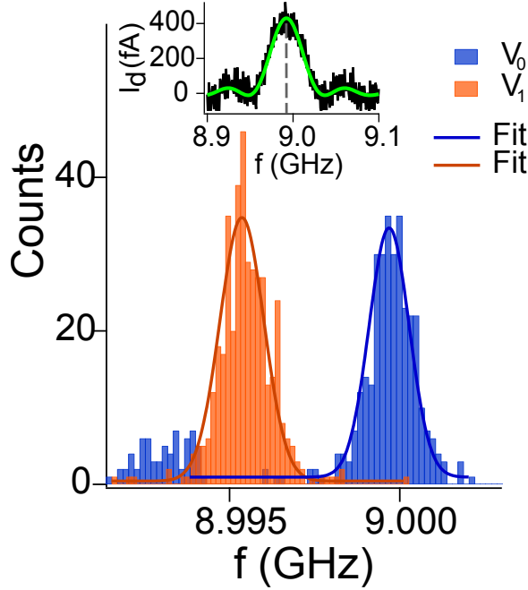
Figure 6.6: Inset: current trace as a function of microwave frequency f for burst duration \tau = 20 ns at \mathbf{B} = (0, 216, 216) mT. Blue and orange histograms display the dispersion of the resonance frequency when V_{G2} is pulsed to point V_0 and V_1 , respectively. The Gaussian fits yield g^*(V_0) = 2.013 \pm 0.001 and g^*(V_1) = 2.010 \pm 0.001 , taking into account the field uncertainty. From Ref. [100].
