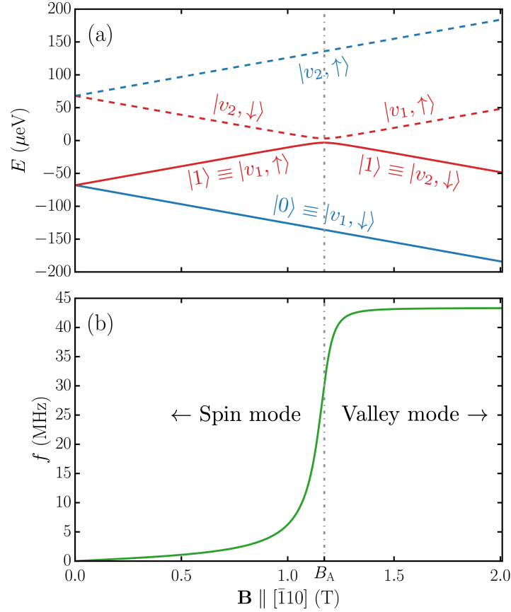
Figure 5.1: (a) Energy levels of the quantum dot in a magnetic field B . The solid blue line is the energy of the |v_1, \downarrow\rangle state, the dotted blue line the energy of the |v_2, \uparrow\rangle state, and the solid and dashed red lines the energies of the |\psi'_-\rangle and |\psi'_+\rangle states (which are mixtures of the |v_1, \uparrow\rangle and |v_2, \downarrow\rangle states that anti-cross at B = B_A = 1.172 T). (b) Computed Rabi frequency for the transition between |0\rangle \equiv |v_1, \downarrow\rangle and |1\rangle \equiv |\psi'_-\rangle (solid lines in (a)). The parameters of the model are \Delta = 136 \mu\text{eV} , |C_{v_1v_2}| = 3.25 \mu\text{eV} , and |D_{v_1v_2}| = 179.26 \mu\text{V/V} . They have been extracted from tight-binding simulations on the device of chapter 4 (Fig. 4.7) at V_g = 0.1 V and V_{\text{bg}} = 0 V. The amplitude of the RF excitation on the front gate is V_{ac} = 1 mV.
