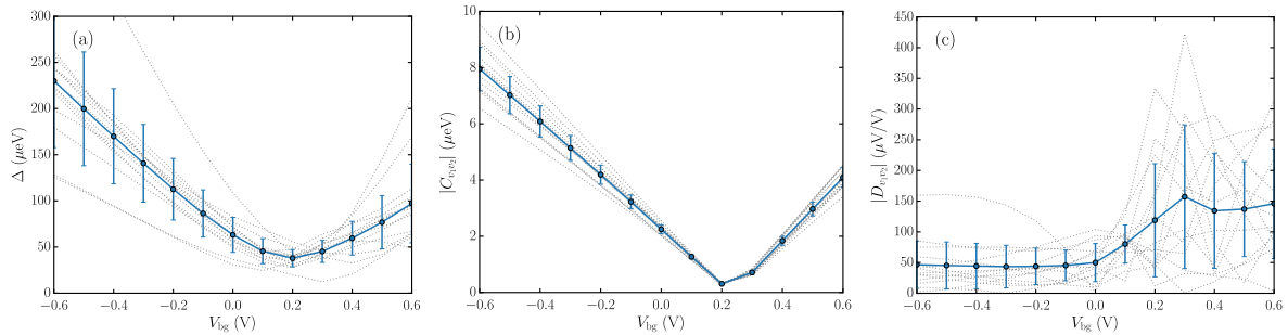
Figure 5.10: (a) Valley splitting \Delta as a function of the back gate voltage V_{bg} , for different realizations of the surface roughness disorder (dotted gray lines). The average and standard deviation are plotted as the blue line and error bars. (b) SOC matrix element C_{v_1 v_2} as a function of the back gate voltage V_{bg} , for different realizations of the disorder (c) Gate coupling matrix element D_{v_1 v_2} as a function of the back gate voltage V_{bg} , for different realizations of the disorder. V_g = 0.1 V in all plots.
