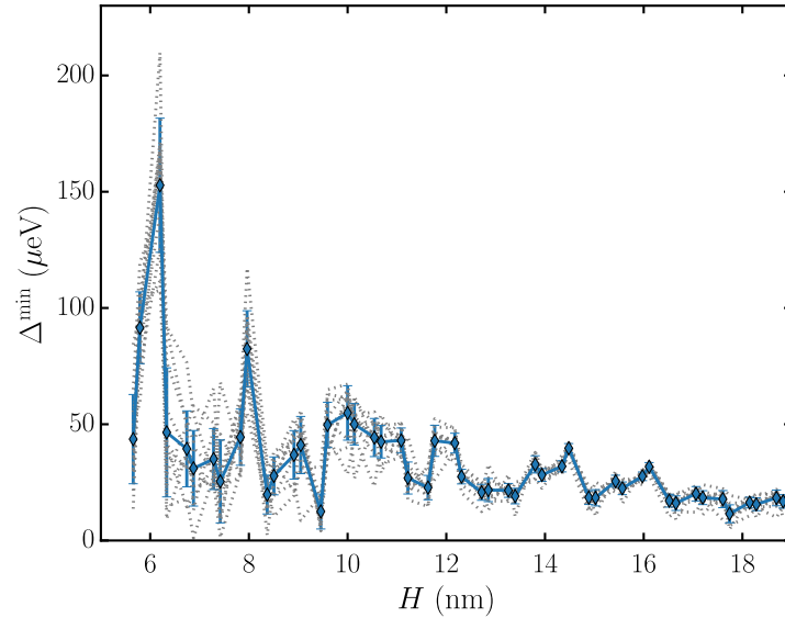
Figure 5.14: Valley splitting as function of the wire thickness H , with surface roughness. The individual samples are in dotted lines, the blue line is for the average valley splitting, and the error bars show the standard deviation.
