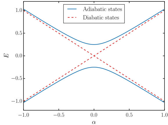
Figure 5.7: Diabatic and adiabatic states of an avoided crossing described by the Hamiltonian of Eq. 5.7.
