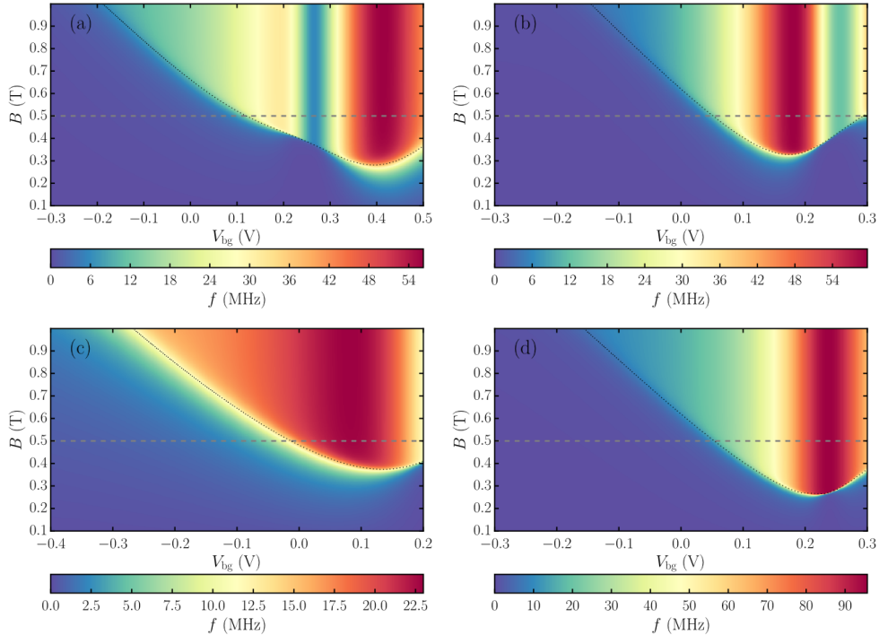
Figure 5.11: Map of the Rabi frequency as a function of the magnetic field and V_{bg} , for different realizations of the disorder. The dotted black line is the anti-crossing condition E_Z = g\mu_B B = \Delta(V_{bg}) . The horizontal dashed line is a target magnetic field B = 0.5 T for qubit operation. V_g = 0.1 V and \mathbf{B} \parallel y in all plots.
