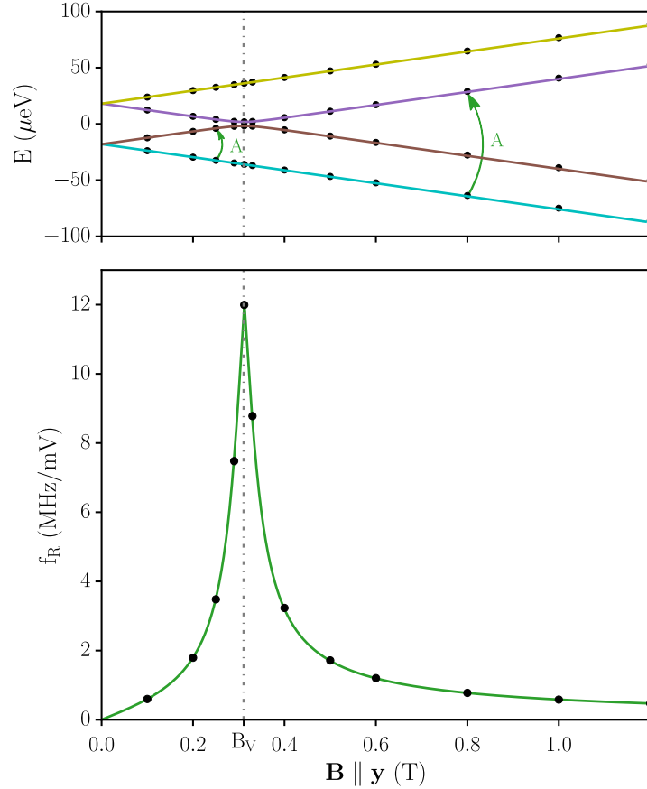
Figure 4.13: Energy levels and Rabi frequency as a function of magnetic field. Here f_R = \min(f_-, f_+) . Coloured lines are from the analytical model, black dots are tight-binding simulations.
