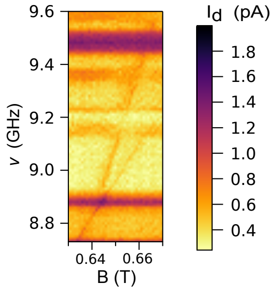
Figure 4.5: Zoom on lines H, B, C of the EDSR map. This scan comes from a different measurement than the one of Fig. 4.4, there are less parasitic lines.
