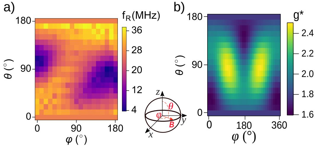
Figure 6.5: (a) Cartography the angular dependence of the Rabi frequency. The measurement is performed at constant Zeeman splitting (9 GHz). (b) Measured g^* cartography. \theta, \varphi are stepped by 10^\circ between 0^\circ and 180^\circ . The whole plot can be obtained by symmetry ( \mathbf{B} \rightarrow -\mathbf{B} ).
