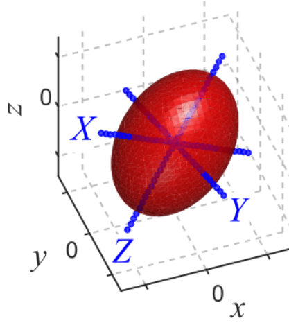
Figure 6.7: Isosurface of \Delta E^2 = g^{*2} \mu_B^2 B^2 in the measurement frame \{\mathbf{x}, \mathbf{y}, \mathbf{z}\} . The blue lines are the principal magnetic axes \mathbf{X}, \mathbf{Y}, \mathbf{Z} of the ellipsoid at V_{G2} = V_0 . From Ref. [100].
