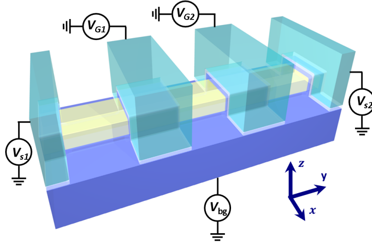
Figure 6.15: Schematic of the device. The silicon nanowire is in yellow, \text{SiO}_2 is in blue, \text{HfO}_2 in light gray and the gates are in dark green.
