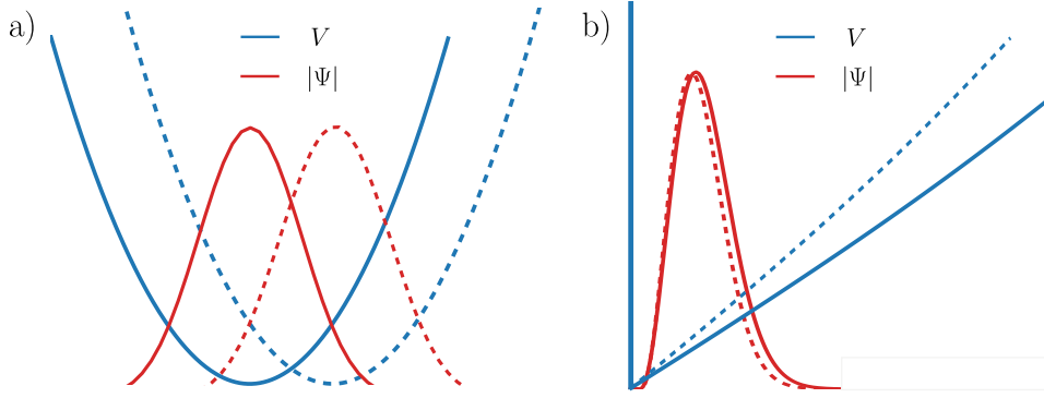
Figure 6.9: Potential and squared wavefunction; the dashed lines represents the same potential with a constant electric field added. (a) State confined in a harmonic confinement potential, an oscillating constant electric field leads to IZ-EDSR. (b) State confined at an interface, an oscillating constant electric field mostly leads to g -TMR.
