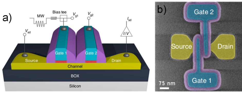
Figure 2.8: (a) 3D schematic of a double quantum dot sample. (b) Top view of the device. From Ref. [93].
