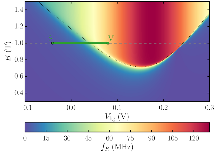
Figure 5.3: Map of Rabi frequency as a function of the magnetic field amplitude and V_{\text{bg}} . The dotted black line is the anticrossing condition E_z = g\mu_B B = \Delta(V_{\text{bg}}) . The RF amplitude is V_{ac} = 1 mV. The green line is the path chosen for qubit operation at B = 1 T.
