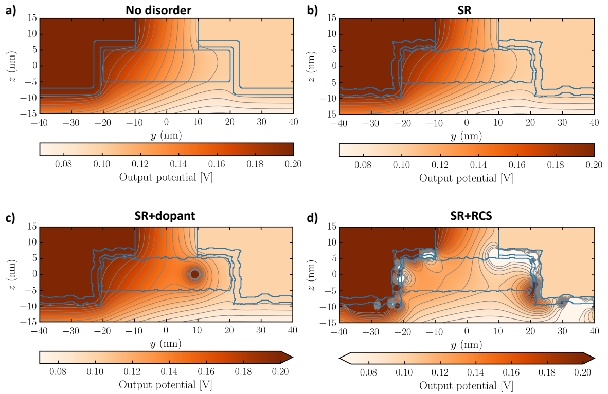
Figure 3.3: Cross-section of the calculated potential in the yz -plane at x = 0 , for different cases. (a) Perfect device without disorder. (b) Including surface roughness (SR). (c) Including SR and one dopant with charge +1 at (x, y, z) = (0, 9, 0) nm. The color scale is the same than (a), with open scale. (d) Including SR and positive RCS charges with surface density n_{\text{RCS}} = 10^{13} \text{ cm}^{-2} . The color scale is the same than (a), with open scale.
