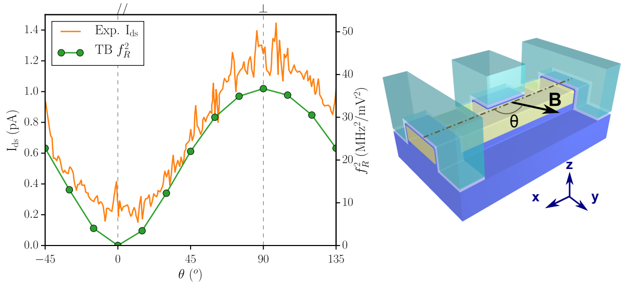
Figure 4.16: Comparison of the dependence with in-plane magnetic orientation of the measured current and of the squared Rabi frequency computed in tight-binding. The directions parallel and perpendicular to the nanowire are highlighted with dashed lines. The definition of the angle \theta is given in the right panel, on the schematic of the device.
