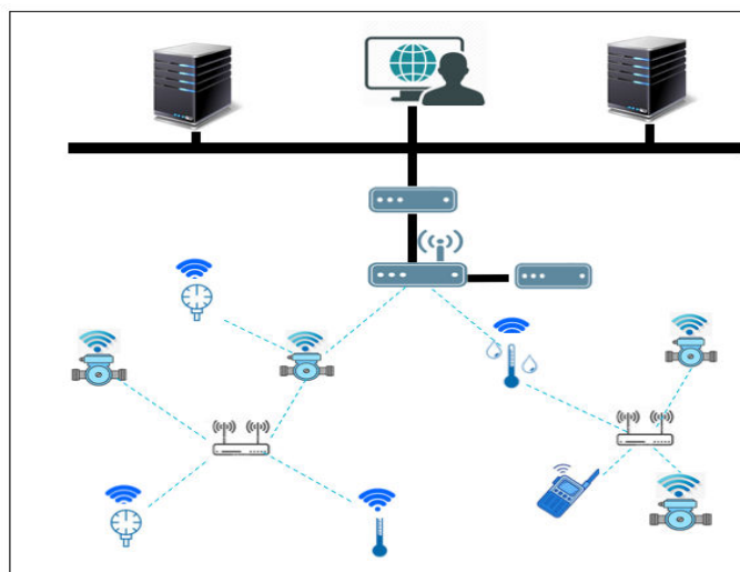
Figure 3.1: Example of a WirelessHART network
