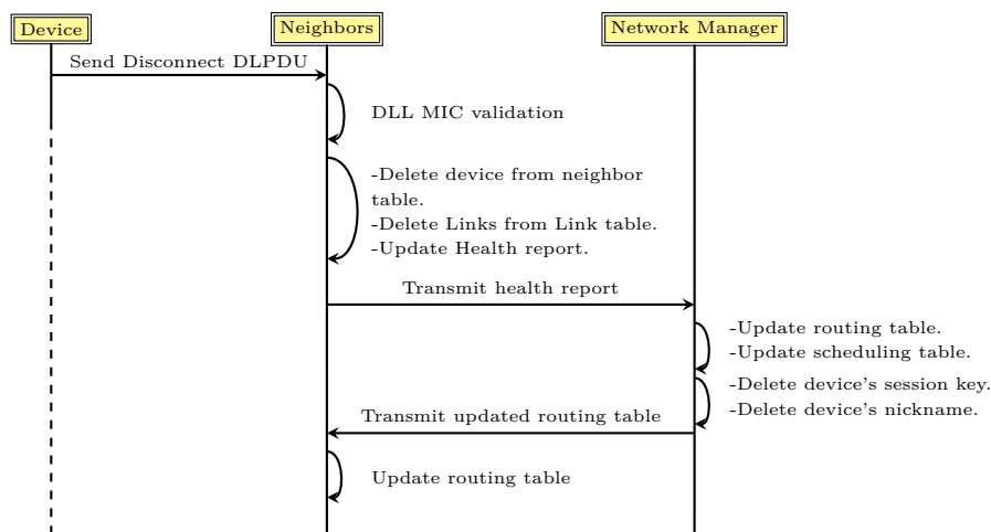
Figure 4.3: Disconnect message exchange sequence
