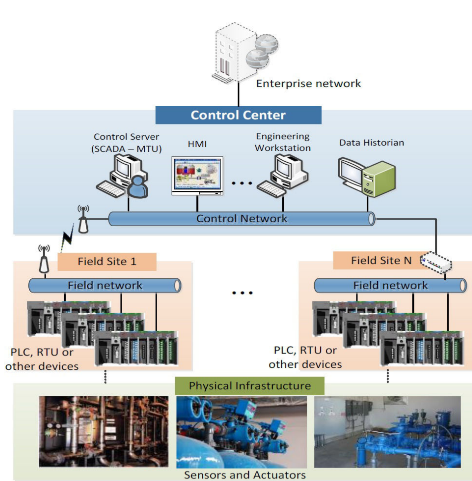
Figure 2.1: ICS Architecture
