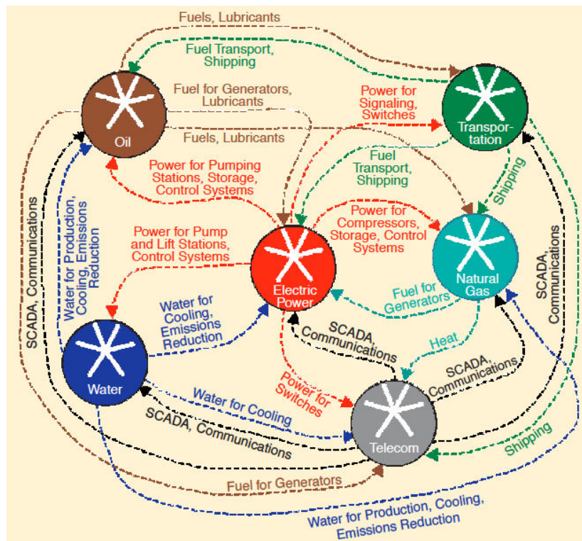
Figure 2.2: Critical infrastructures interdependencies [Rinaldi et al. 2001]
