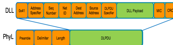
Figure 3.4: WirelessHART DLPDU structure
