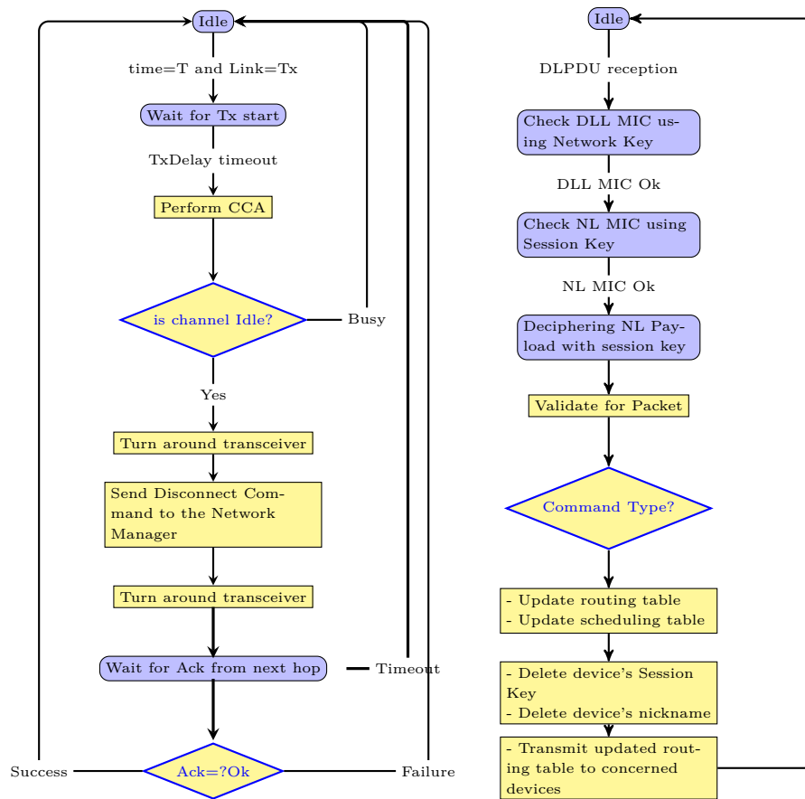
(a) Modified Disconnect DLPDU Command by device (b) Modified Disconnect Command reception by NM
