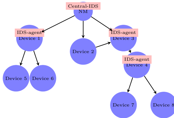
Figure 5.2: IDS-agents deployment
