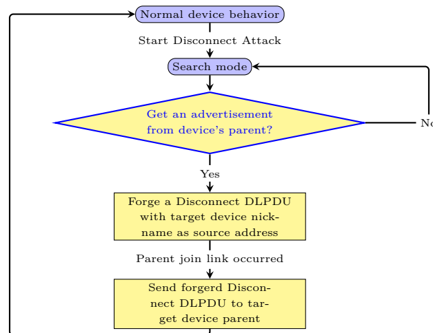
Figure 4.4: Sybil Disconnect Attack
