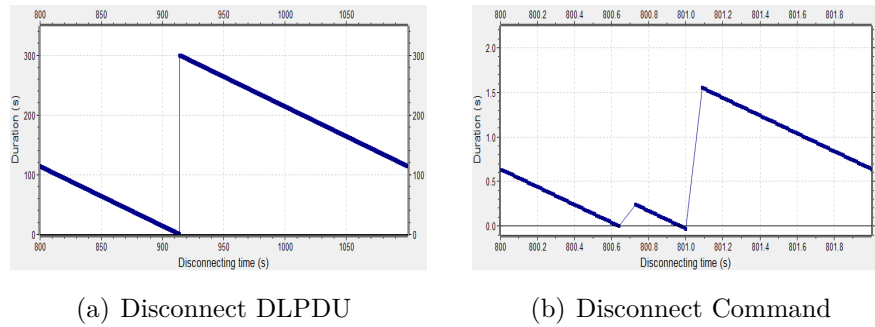
Figure 4.11: Time duration before the NM is informed about a device disconnection
