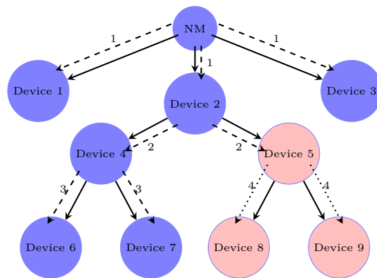
Figure 4.16: On-the-fly Broadcast attack
