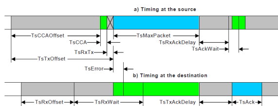
Figure 3.6: Slot timing
