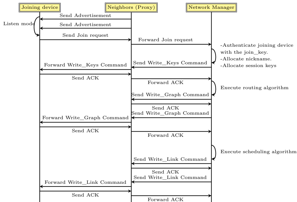
Figure 4.1: Joining message exchange sequence
