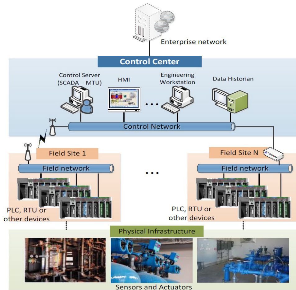
Figure 2.1: ICS Architecture
