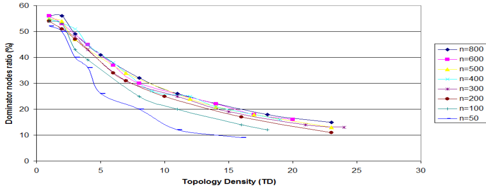
Figure 6.4: Dominating nodes ratio compared to the Topology Density
