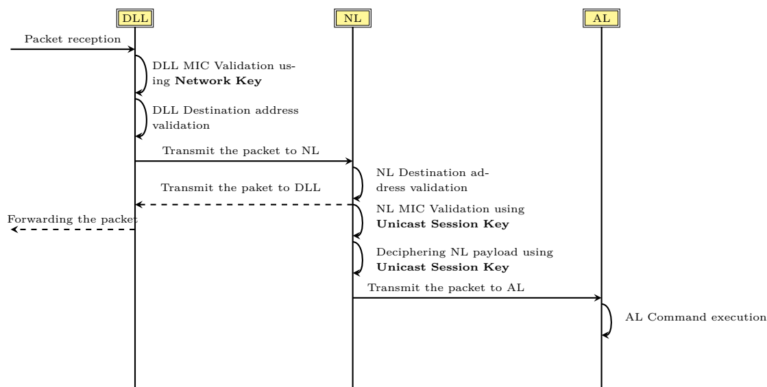
Figure 4.12: Unicast packet processing sequence
