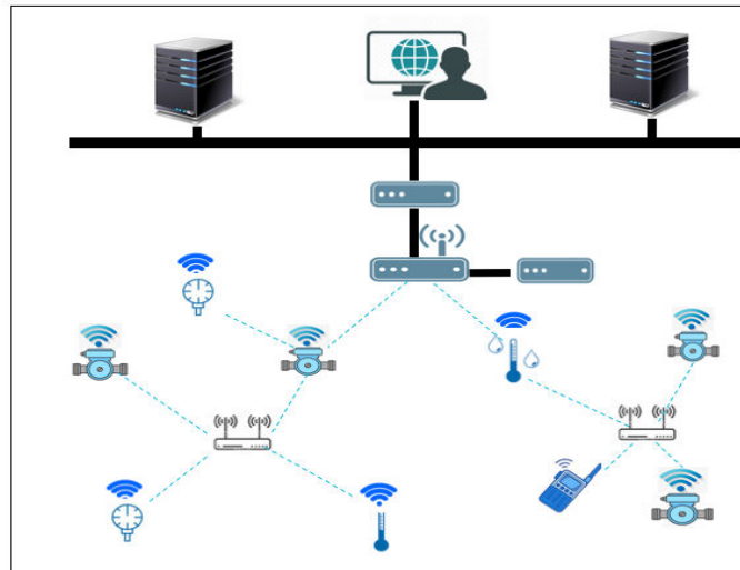
Figure 3.1: Example of a WirelessHART network
