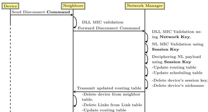
Figure 4.10: Modified Disconnect message exchange sequence
