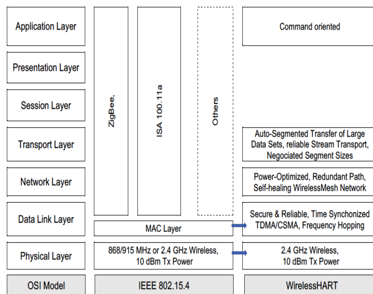
Figure 3.2: WirelessHART protocol stack [Deji et al. 2010]
