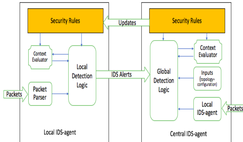
Figure 5.1: The Central IDS-agent and IDS-Agents Architecture
