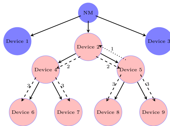
Figure 4.15: Bounced Broadcast attack
