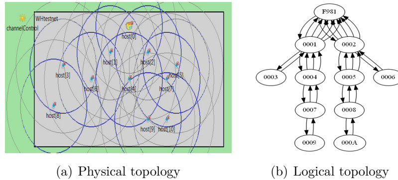
Figure 4.5: Simulation network topology
