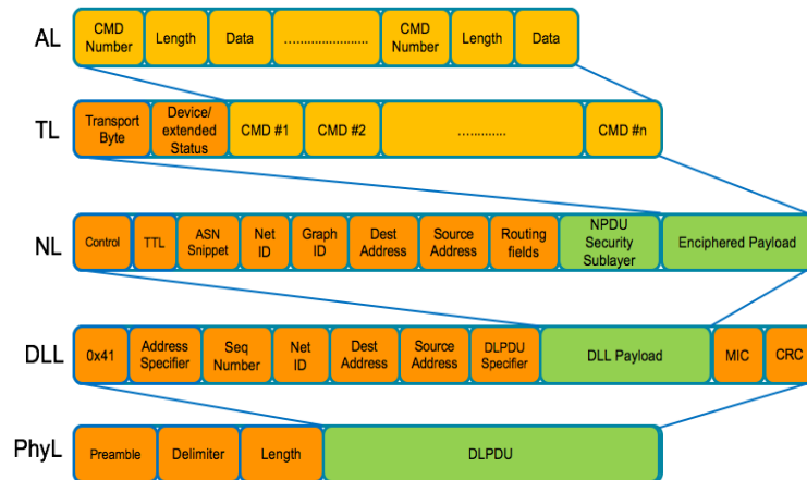
Figure 3.3: WirelessHART packets structure
