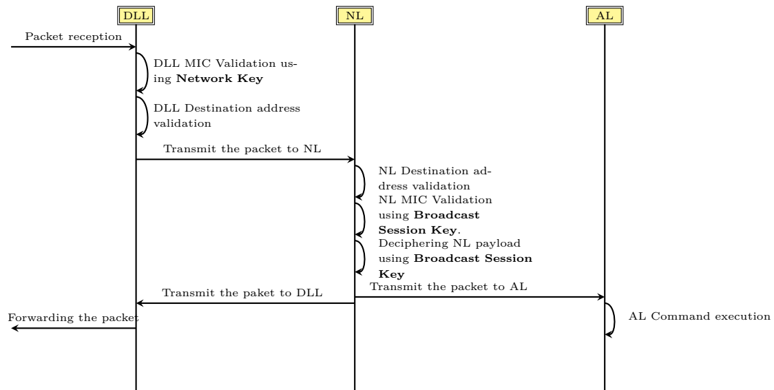
Figure 4.13: Broadcast packet processing sequence
