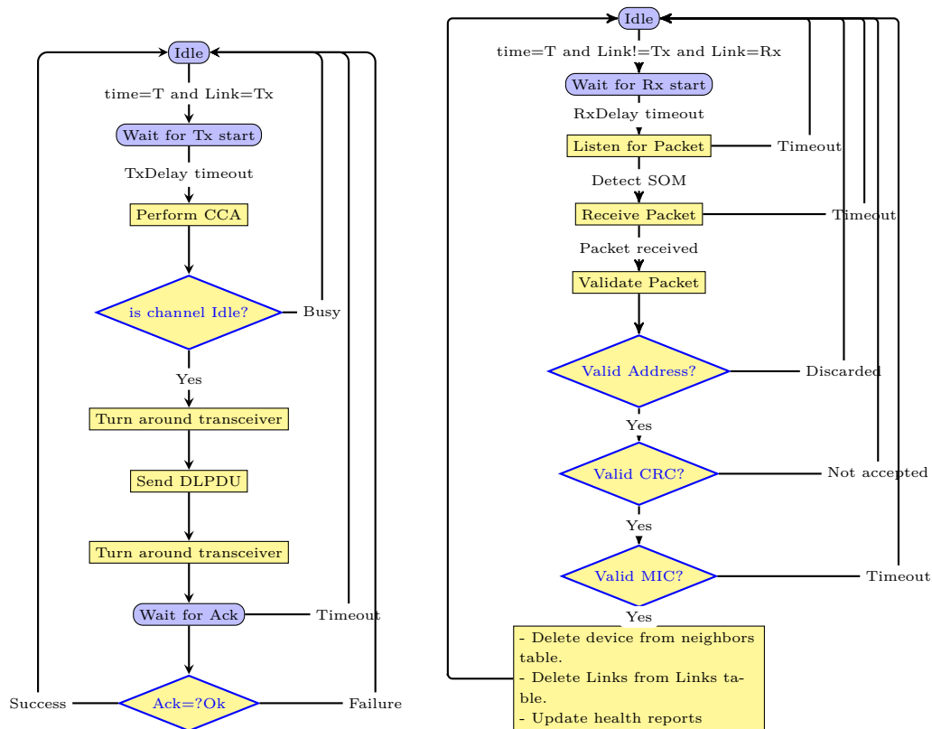
(a) Disconnect DLPDU transmission by device (b) Disconnect DLPDU reception by neighbors
