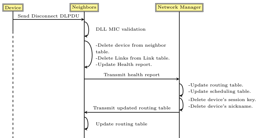
Figure 4.3: Disconnect message exchange sequence
