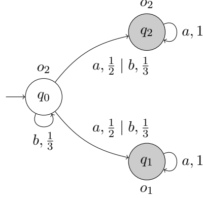
Figure 7.5: An example of OMDP where the initial distribution is a Dirac distribution on q_0 . Transitions are labelled by a set of pairs of actions and of the probability to take this transition under that action.
