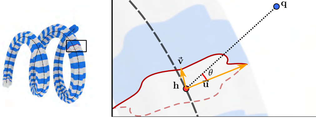
Figure 2.5: Evaluation of an extrusion surface field function: the point \mathbf{q} is projected on the axis curve \mathcal{C} on point \mathbf{h} . The evaluation is the difference between the distance \|\overrightarrow{\mathbf{qh}}\| and the radius of the profile curve R(s(\mathbf{q}), \theta) , defined in the orthogonal plane (\vec{\mathbf{u}}, \vec{\mathbf{v}}) .
