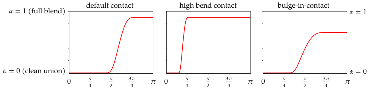
Figure 3.5: Controller functions used for Implicit Skinning.
