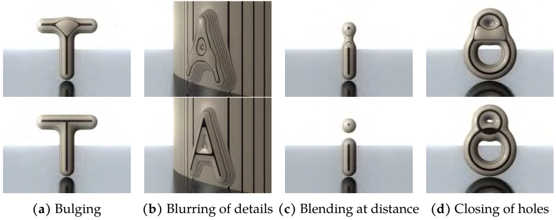
Figure 2.11: Top row: common blending artefacts. Bottom row: expected solutions.
