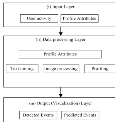
Figure 7.2 – The overall framework of Event detection method including modules
