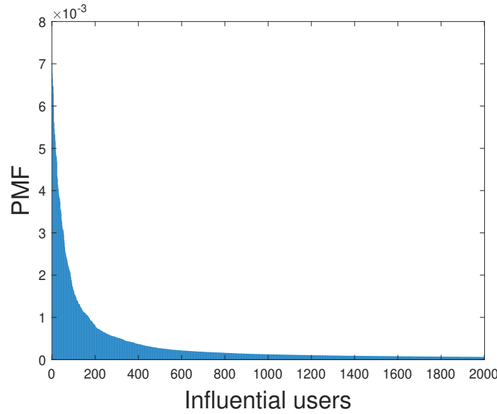
Figure 5.1 – The probability mass function of credibility in Etsy data-set influential and the rest ones in comparison with Epinions.
