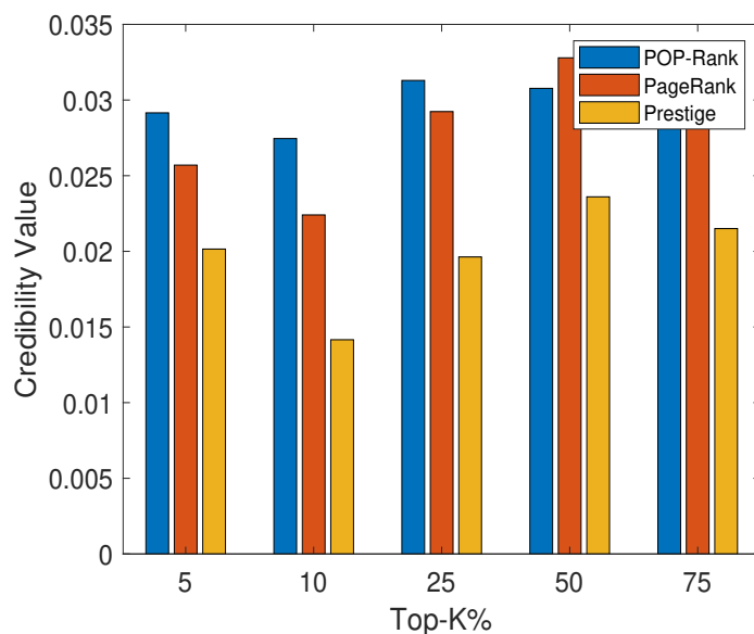
Figure 5.2 – Normalized Credibility of each ranking algorithm regarding different percentages of found influential users in Etsy. X axis represents different percentages of top found users and Y axis shows the normalized credibility value of found users
