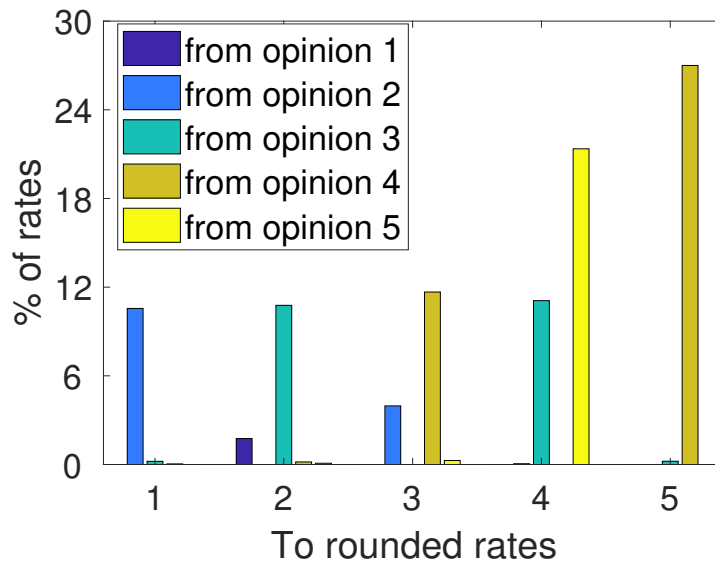
Figure 4.3 – Users rates changed to other rates (rounded) in Epinion Dataset
