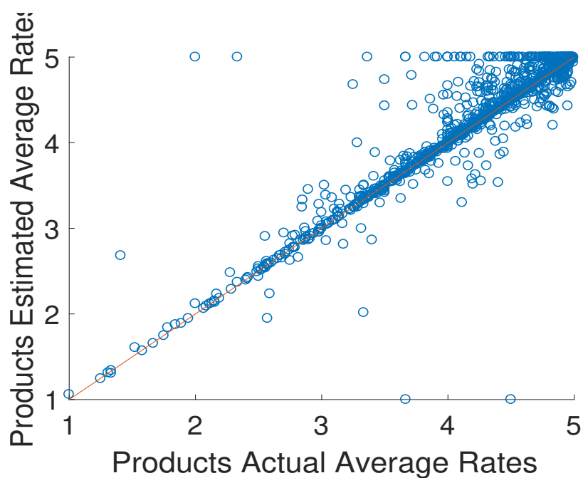
Figure 4.12 – Etsy dataset - The spread of different average rates of products.
