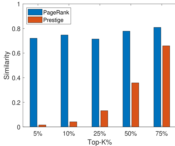
Figure 3.2 – Similarity of POPRank with each approach in found influential users. X axis represents different percentages of top found influential users and Y axis shows the similarity with POPRank
