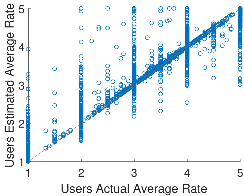
Figure 4.8 – Epinions dataset - The spread of different average rates of each user.
