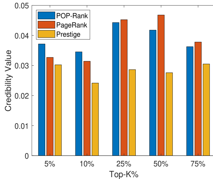
Figure 3.3 – Normalized Credibility of each ranking algorithm regarding different percentages of found influential users in Epinions. X axis represents different percentages of top found users and Y axis shows the normalized credibility value of found users
