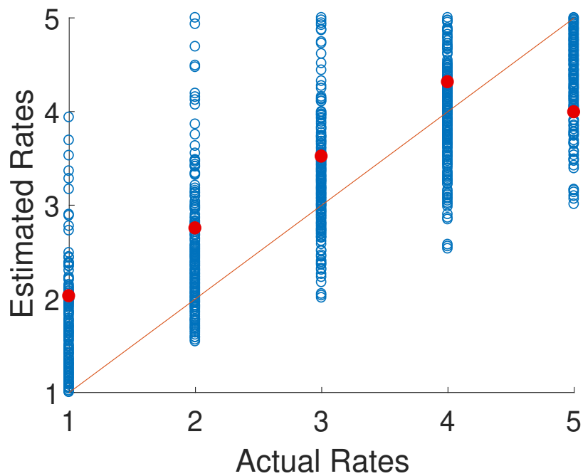
Figure 4.7 – Epinions dataset - The spread of different rates of users. The red circle is the average of estimated rates
