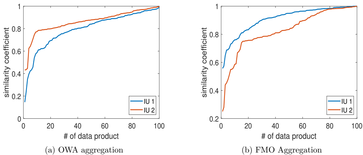
Figure 5.3 – Aggregation in Epinions dataset
