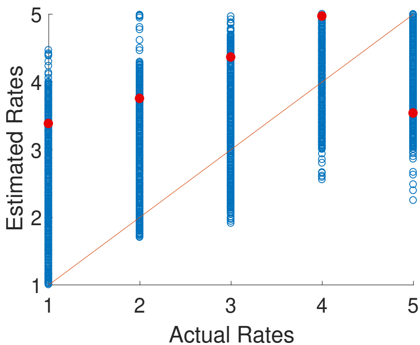
Figure 4.10 – Etsy dataset - The spread of different rates of users. The red circle is the average of estimated rates
