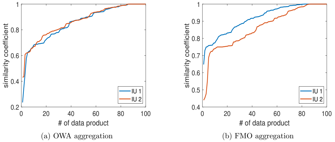
Figure 5.4 – Aggregation in Etsy dataset
