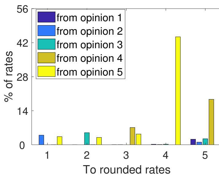
Figure 4.6 – Users rates changed to other rates (rounded) in Etsy Dataset
