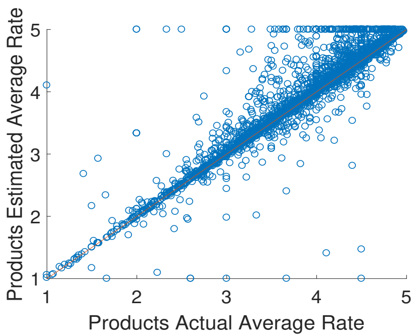
Figure 4.9 – Epinions dataset - The spread of different average rates of products.
