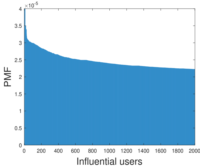
Figure 3.1 – The probability mass function of credibility in Epinions data-set
