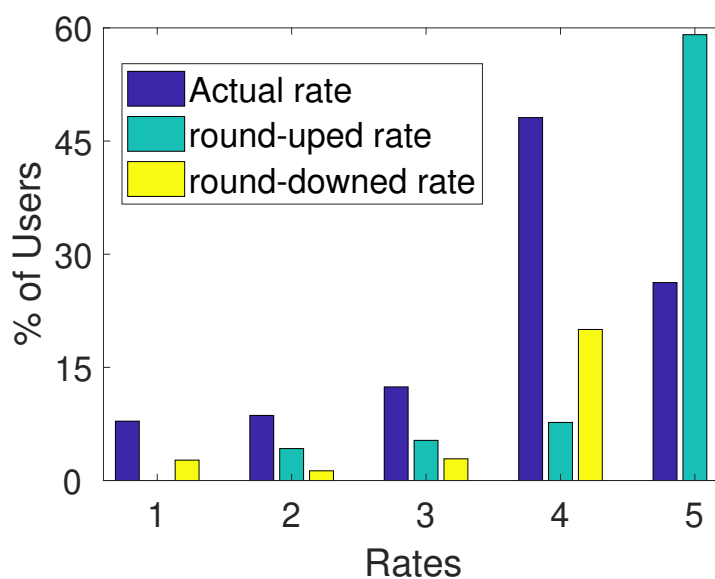
Figure 4.5 – Actual rates, round-up and round-down rates in Etsy Dataset
