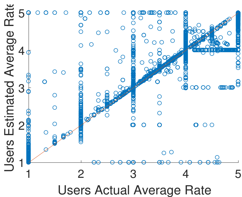
Figure 4.11 – Etsy dataset - The spread of different average rates of each user.
