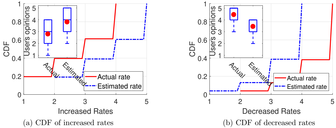
Figure 4.1 – CDF of Epinions dataset
