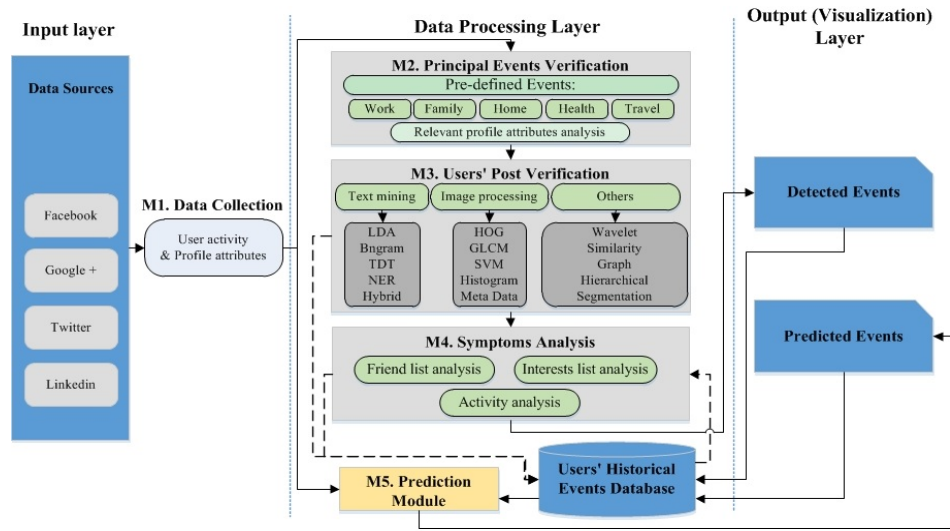
Figure 7.3 – The block diagram of the event detection framework including the three layers and different modules.
