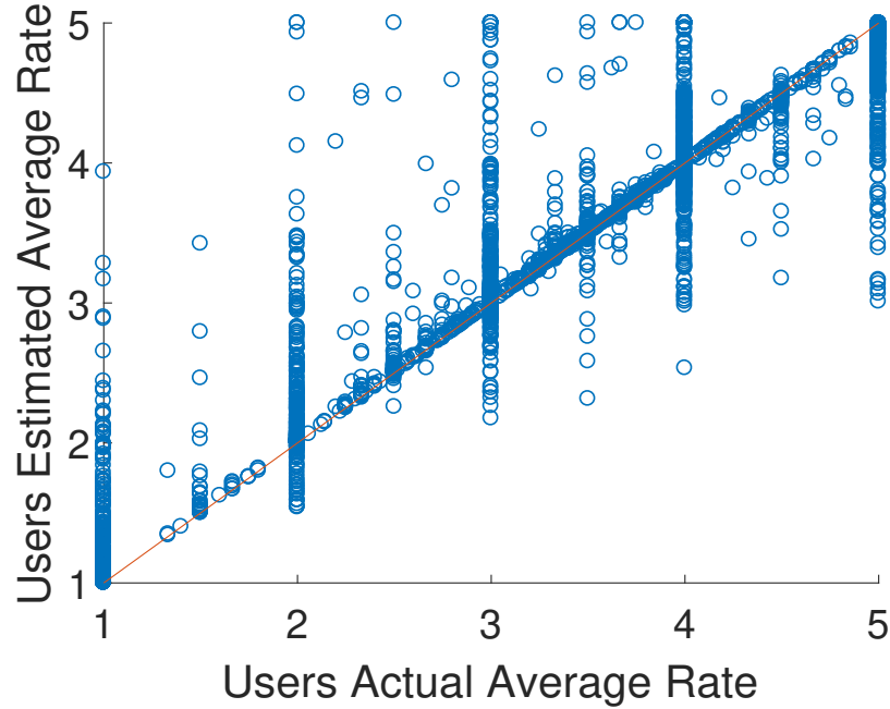
Figure 4.8 – Epinions dataset - The spread of different average rates of each user.
