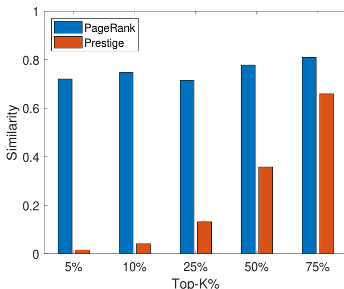
Figure 3.2 – Similarity of POPRank with each approach in found influential users. X axis represents different percentages of top found influential users and Y axis shows the similarity with POPRank
