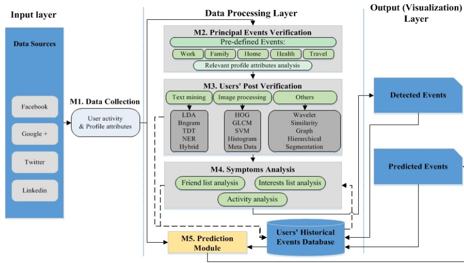
Figure 7.3 – The block diagram of the event detection framework including the three layers and different modules.
