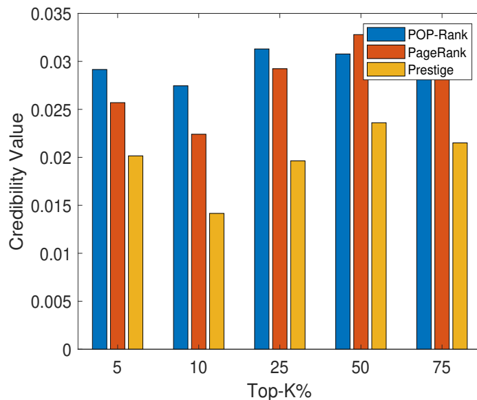
Figure 5.2 – Normalized Credibility of each ranking algorithm regarding different percentages of found influential users in Etsy. X axis represents different percentages of top found users and Y axis shows the normalized credibility value of found users
