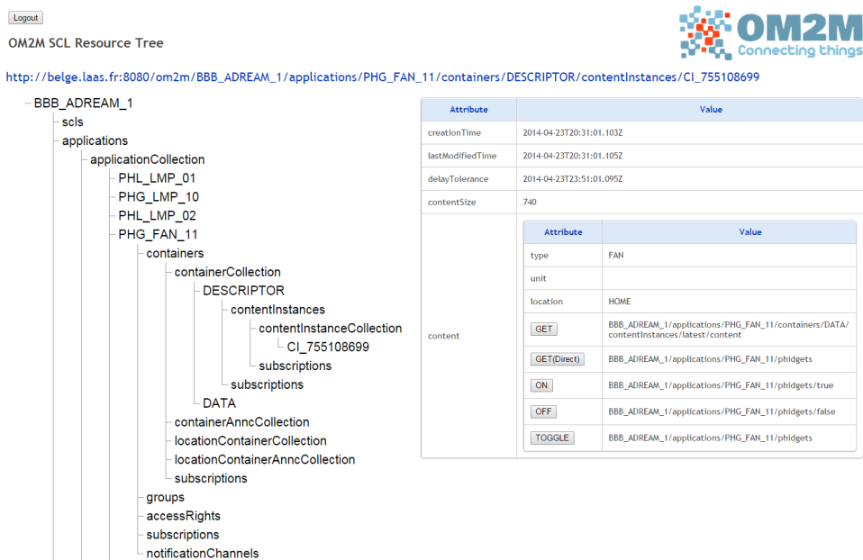
Figure 2.15: Resource tree browser web interface
