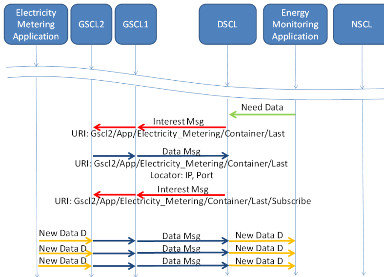
Figure 4.5: Message Sequence Chart with OSCL and ICN messages.
