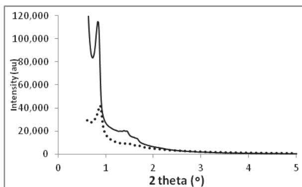
Fig. 2. Small angle XRD patterns of \text{SBA}^{20}\text{-COO}^-\text{N}^+ (dotted line) and \text{SBA}^{10}\text{-COO}^-\text{N}^+ (continuous line).
