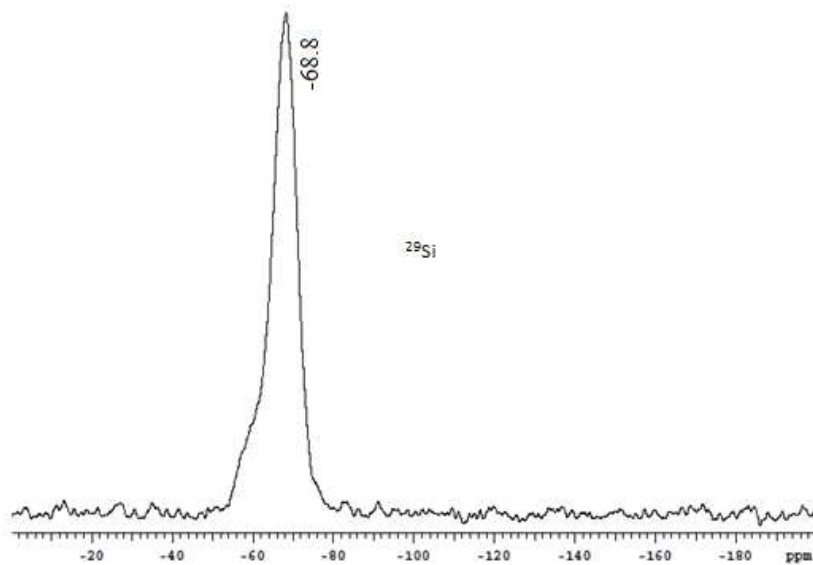
Figure 43 : Spectre RMN ^{29}\text{Si} du solide lamellaire \text{O}_{1.5}\text{Si}(\text{CH}_2)_3\text{-NH}_2
