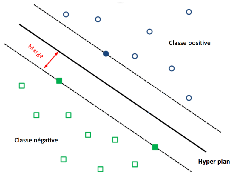
Figure 12 Classification SVM
