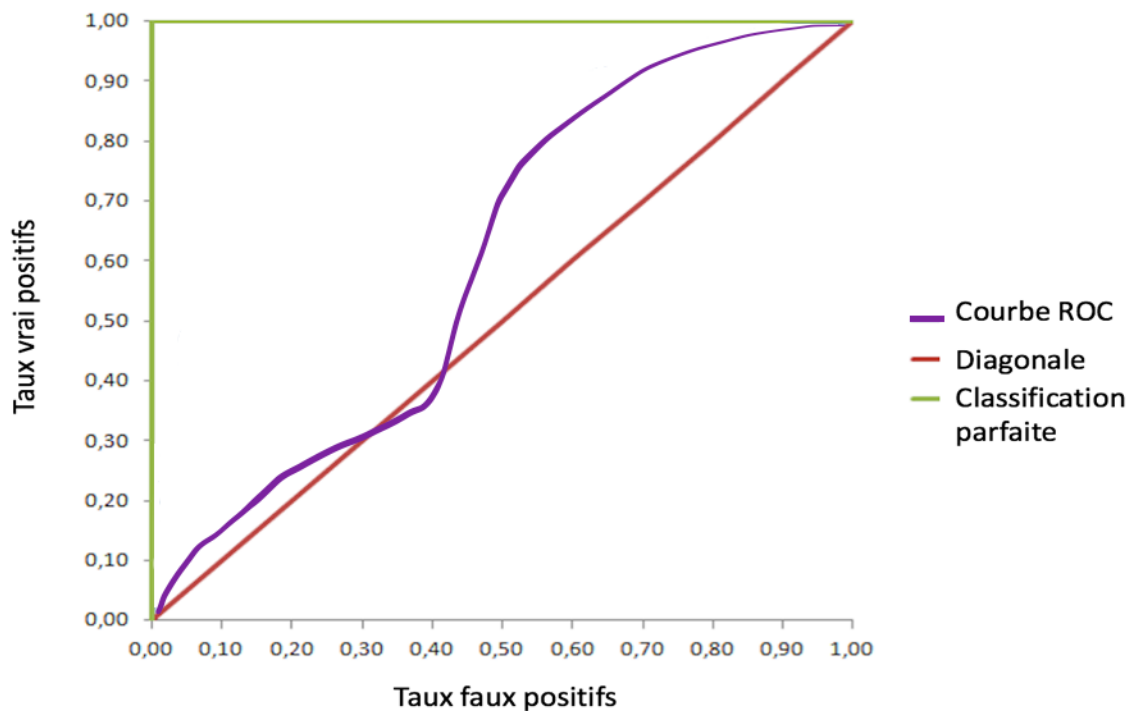
Figure 13 Courbes ROC
