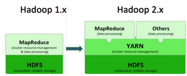
Figure 4: Hadoop 1.x vs Hadoop 2.x
