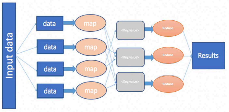
Figure 6: La phase MapReduce
