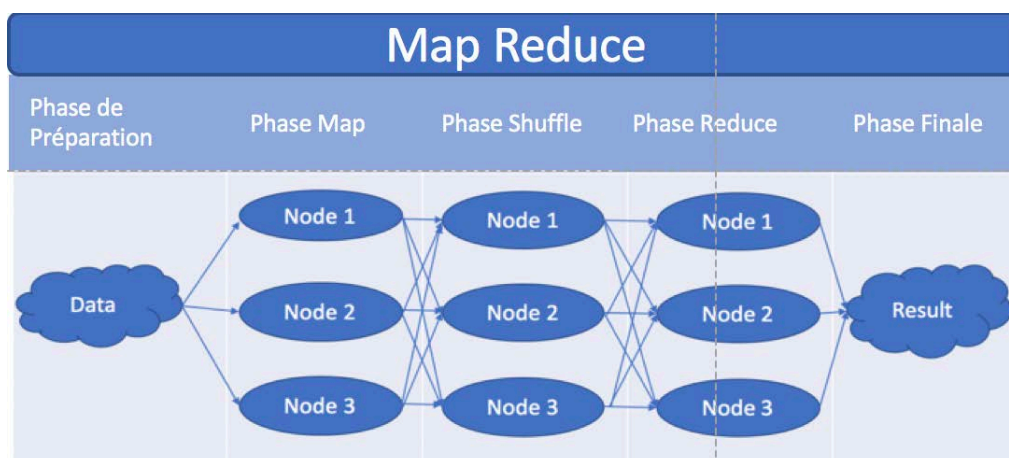
Figure 5: Le concept de MapReduce
