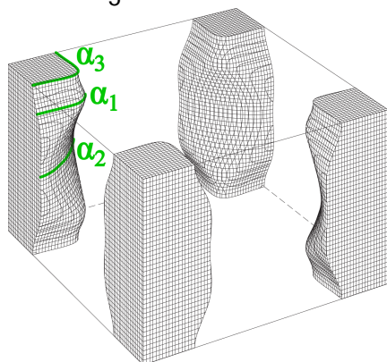
LaRhIn 5 band 15-electron
