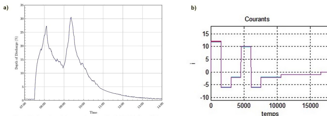
Figure 4. Mars Express battery DoD over approximately one orbit on DoY 2014-074. First peak is due to solar eclipse by Mars, the second due to science pointing that required suboptimal array pointing.
