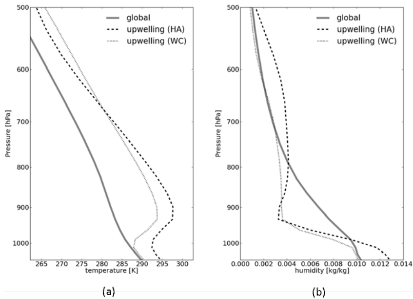
FIGURE 3.29 – Profiles of (a) temperature and (b) specific humidity averaged over WC (dotted lines) and HA (dashed lines) upwelling areas during June 2015. Profiles are compared to mean temperature and specific humidity profiles averaged over global ocean (grey continuous line) during June 2015
