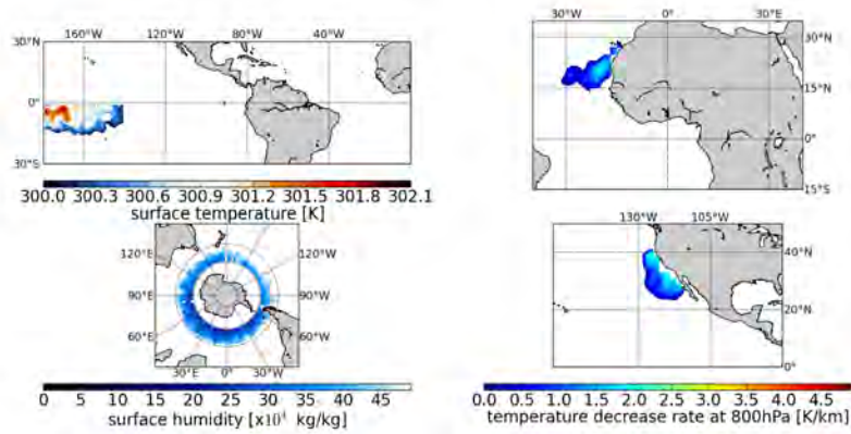
FIGURE 3.27 – Location of the four areas of study chosen according to different geophysical parameters averaged over June 2015 : the PWP-area driven by high surface temperatures (upper left panel), the HL-area characterized by surface humidity lower than 0.005 kg/kg (lower left panel) and the two HA-area and WC-area upwelling regions characterized by positive temperature decrease rate values (upper and lower right panels, respectively)
