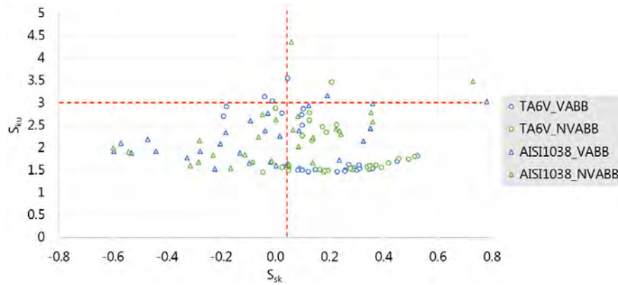
Figure 5.46. S_{sk} - S_{ku} plot of VABB and NVABB results obtained on AISI 1038 and Ti-6Al-4V tests.
