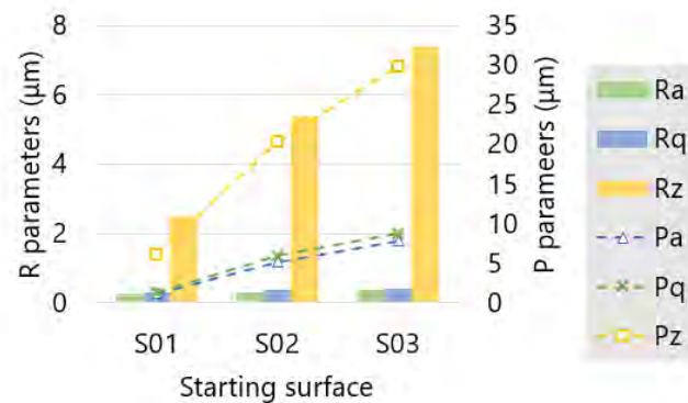
Figure 5.28. Bidimensional descriptors of original surfaces (Ti-6Al-4V).
