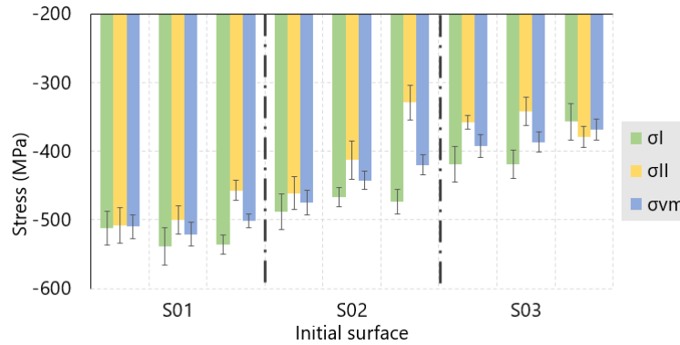
Figure 5.61. Residual stress descriptors at S_1^0 , S_2^0 and S_3^0 Ti-6Al-4V surfaces.
