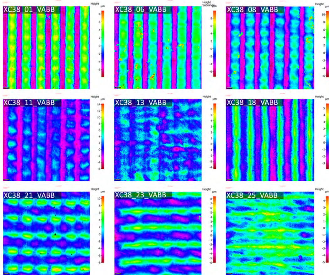
Figure B.1. Sequential height colour map of all VABB tests on AISI 1038 S_1^0 surfaces.
