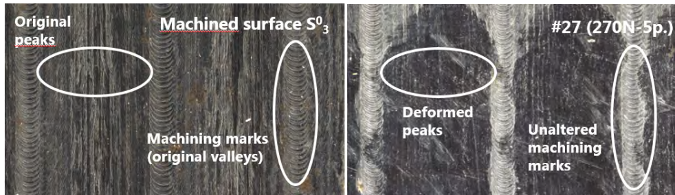
Figure 5.14. Optical images of S^0_3 and #27VABB surfaces.
