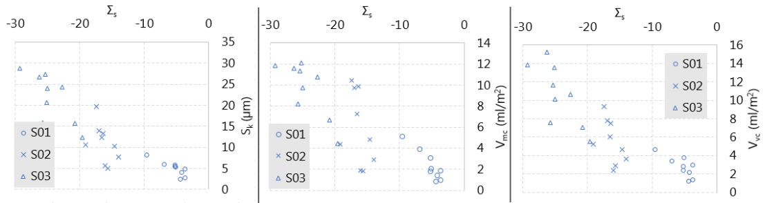
Figure 5.37. Correlation between \Sigma_s and S_k , V_{mc} and V_{vc} of VABB tests on Ti-6Al-4V.
