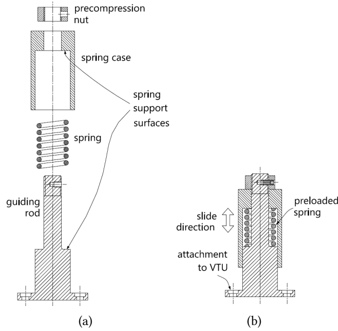
Figure 3.2. Diagram of the FTU. a. Exploded view. b. Assembled parts and spring compression.
