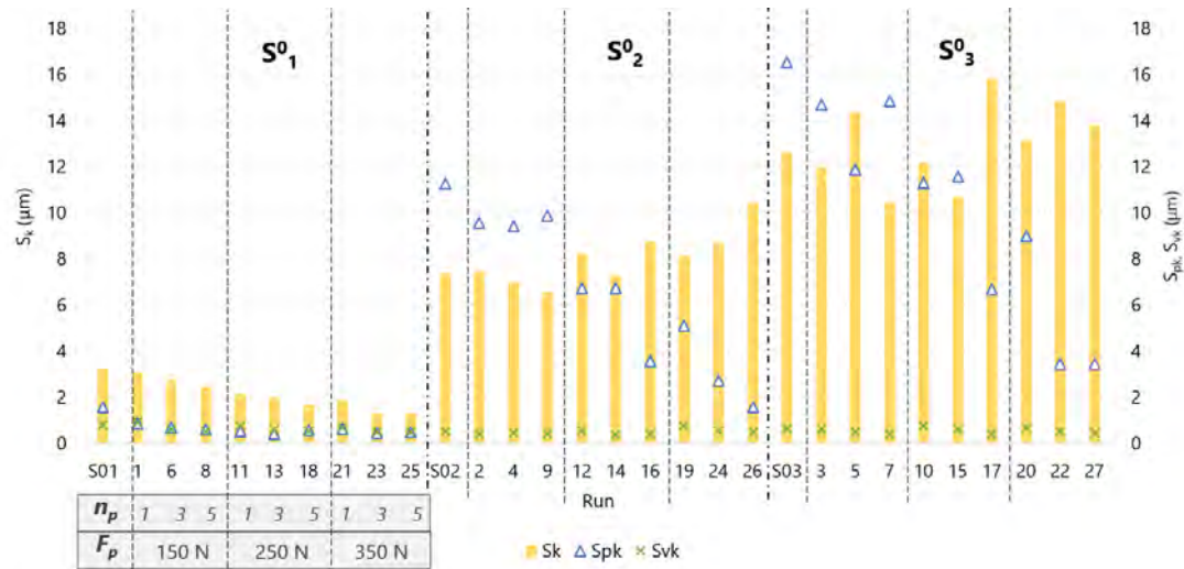
Figure 5.39. Abbott-Firestone amplitude parameters of Ti-6Al-4V burnishing patches.
