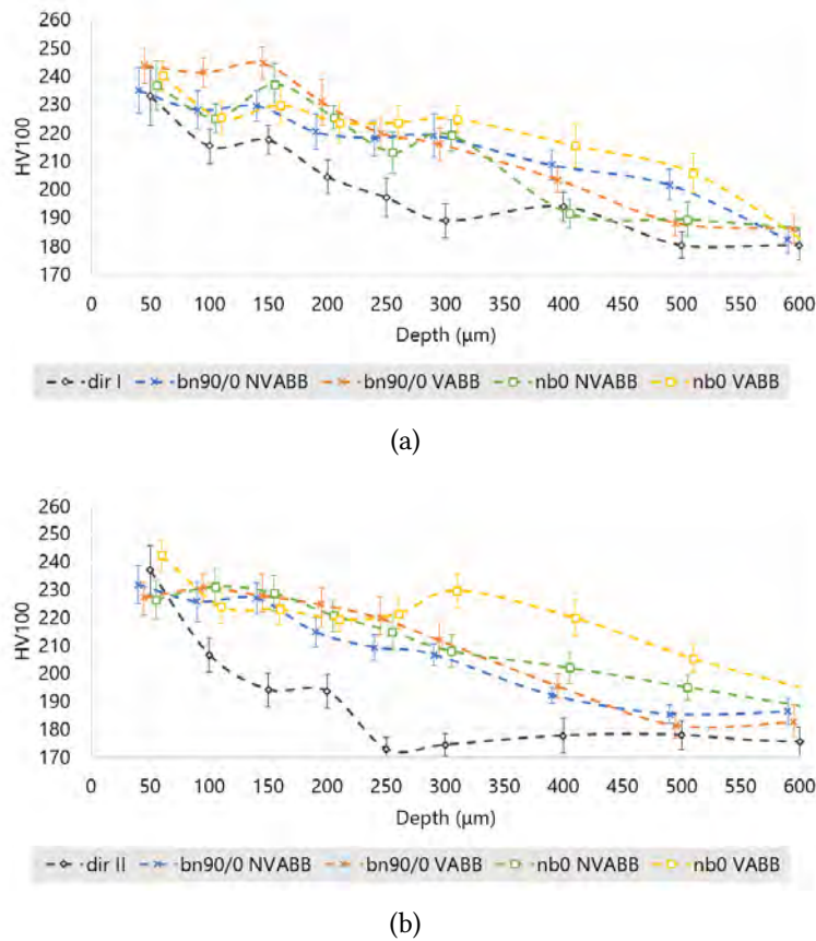
Figure 5.68. Hardness profiles of VABB and NVABB S_1^0 AISI 1038 surfaces. a. Along direction I. b. Along direction II.
