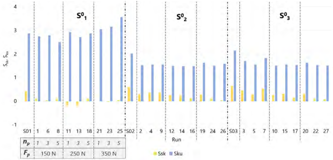
Figure 5.32. S_{sk} and S_{ku} amplitude parameters of Ti-6Al-4V burnishing patches.
