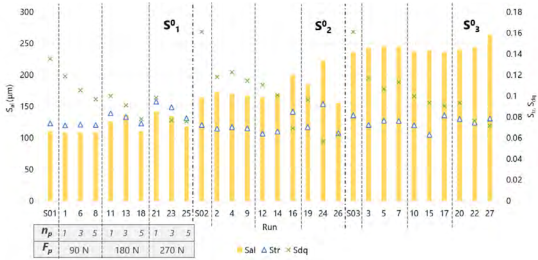
Figure 5.13. S_{al} and S_{tr} spatial parameters and S_{dq} hybrid parameter of AISI 1038 VABB patches.
