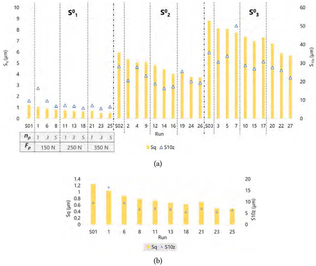
Figure 5.31. a. S_q and S_{10z} amplitude parameters of Ti-6Al-4V burnishing patches. b. Detail of S_1^0 results.
