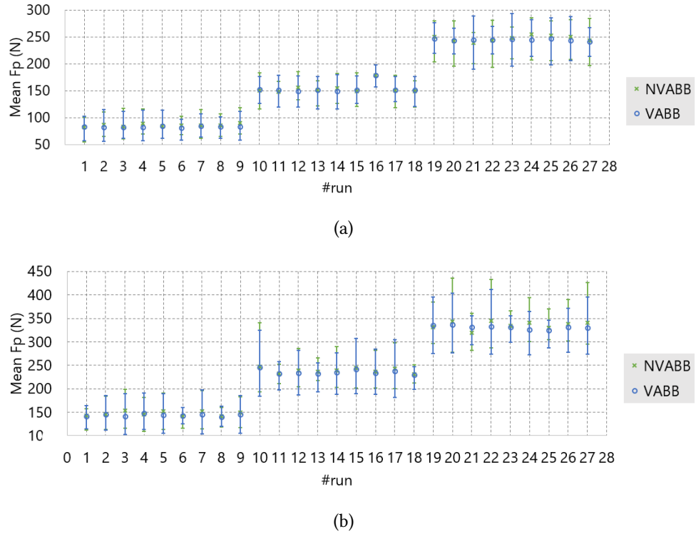
Figure 4.22. Mean F_z registered for all burnishing cycles, and maximum and minimum forces registered. a. AISI 1038. b. Ti-6Al-4V.
