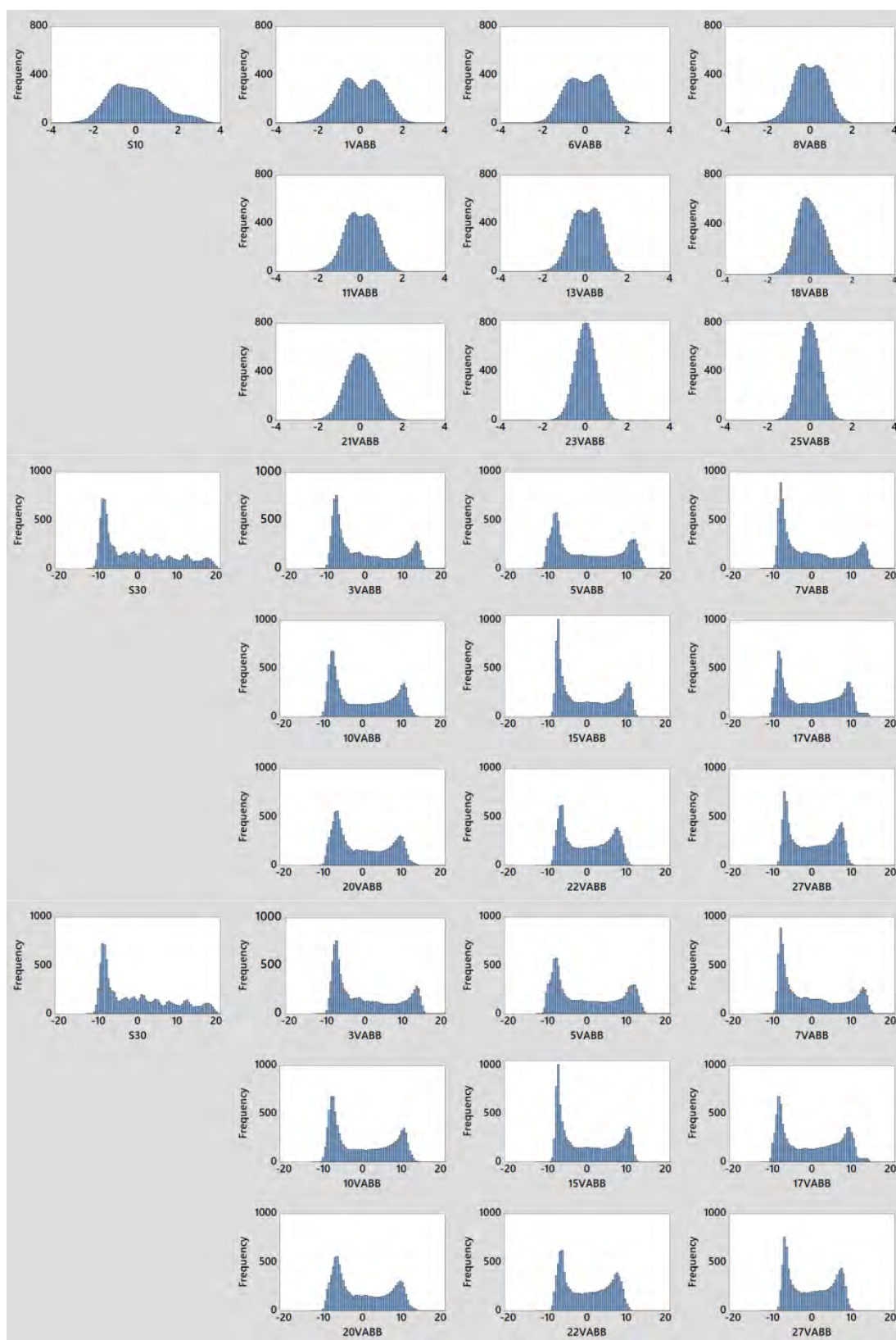
Figure C.4. VABB height distributions of Ti-6Al-4V surfaces.
