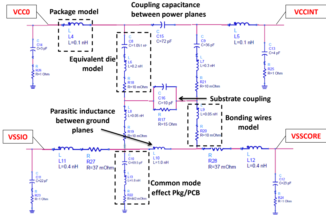
Figure II-25 Simplified view of the PDN model between VCCO/VSSIO and VCCINT/VCCINT
