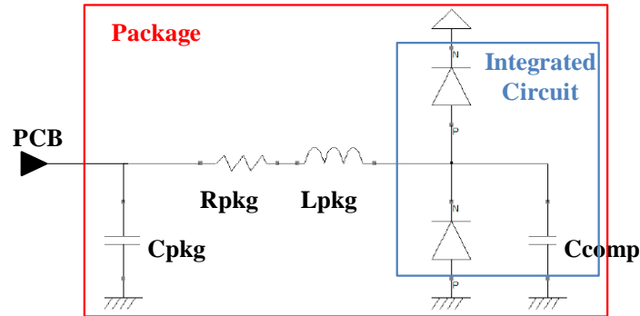
Figure II-3 IBIS model of an input
