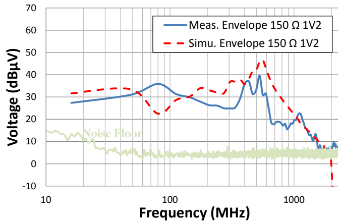
Figure II-81 Comparison between the measurement and simulation of CE on 1.2 V power plane using the 150 Ω probe for the industrial application
