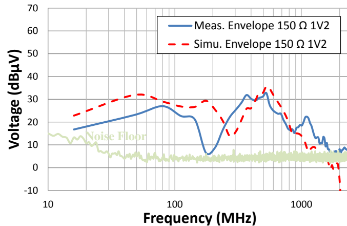
Figure II-69 Comparison between measured and simulated CE using the 150 \Omega probe on 1.2 V power plane for the 7-bits counter configuration
