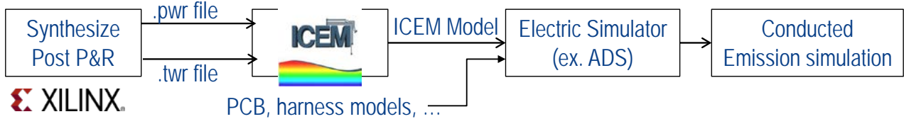
Figure II-76 Workflow of CE simulation using ICEM GENERATOR
