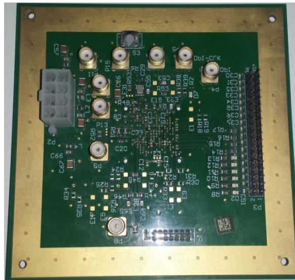
Figure II-15 The designed demonstrator ELECIS-F
