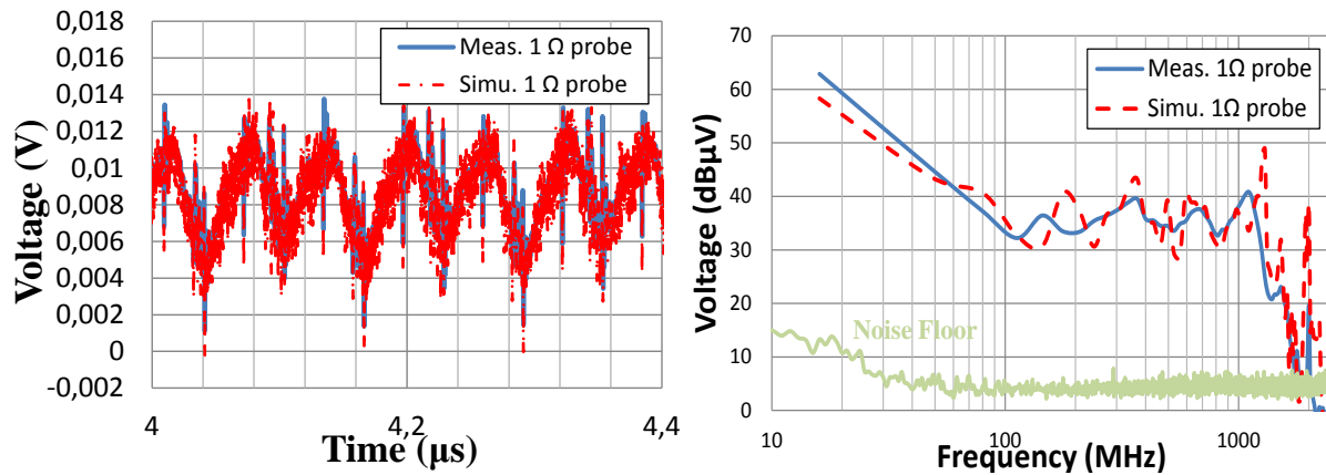
Figure II-51 Comparison between the simulated and measured CE using the 1 Ω probe in the time domain (left) and frequency domain (right)
