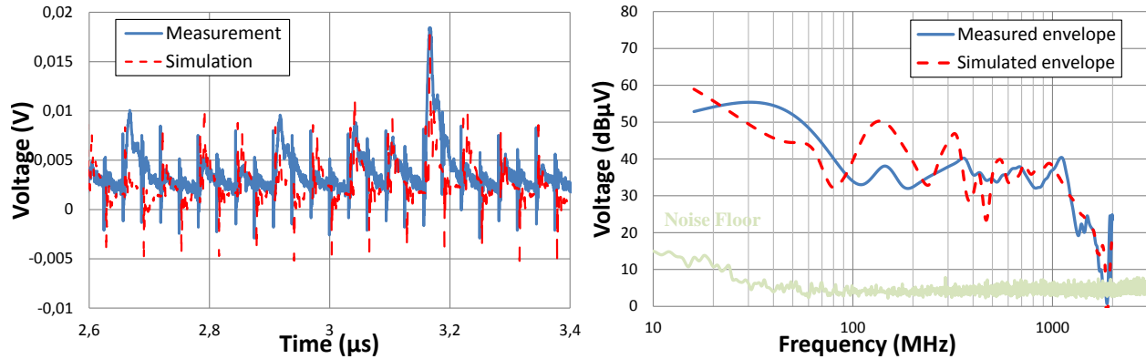
Figure II-68 Comparison between the measured and simulated CE with the 1 \Omega probe in the time domain (left) and the frequency domain (right) for the 7-bits counter configuration using the statistical approach
