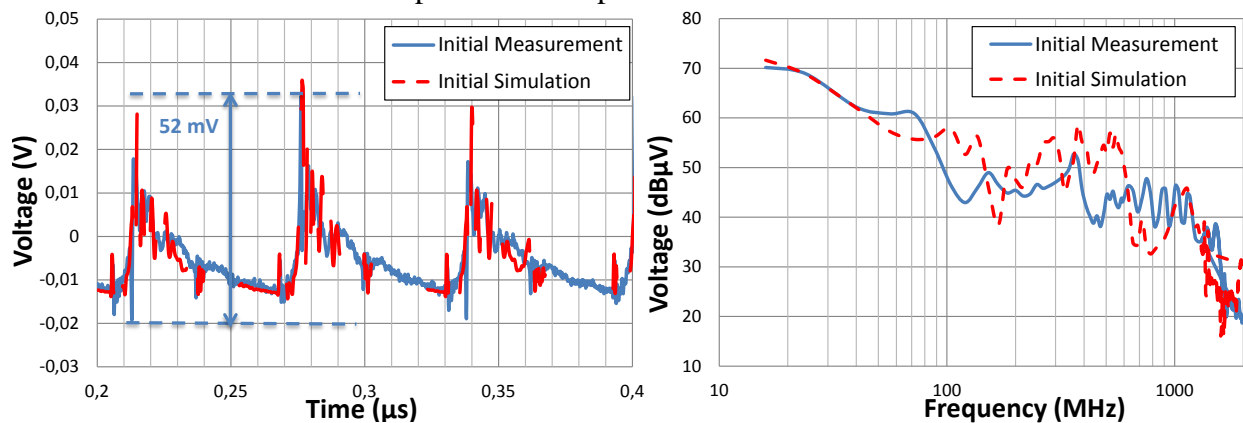
Figure IV-46 Comparison between measured and simulated CE using the 1\ \Omega probe before aging when the IOs are activated
