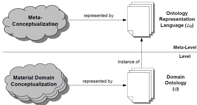
FIGURE 2.3: Relations between a material domain conceptualization, domain ontology, general meta-conceptualization, and ontology representation language (Guizzardi, 2005).
