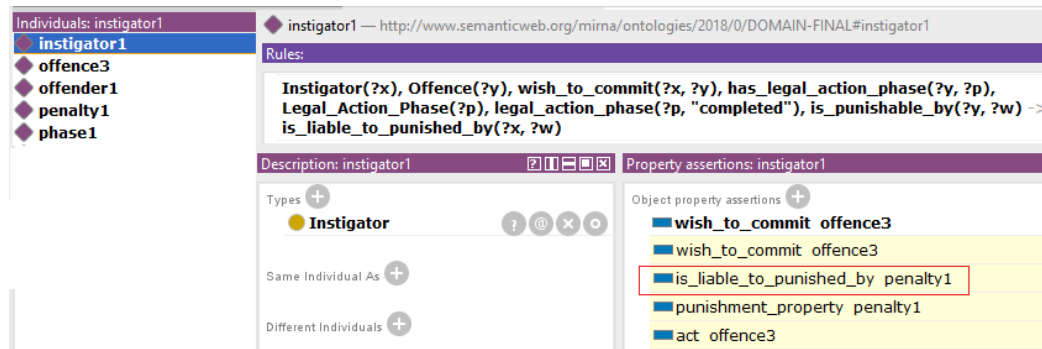
FIGURE 5.19: Article 218 using CriMonto and SWRL in Protégé.
