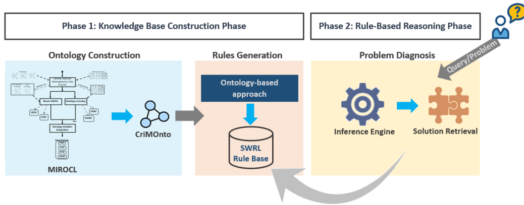
FIGURE 6.2: Hybrid approach for building CORBS.
