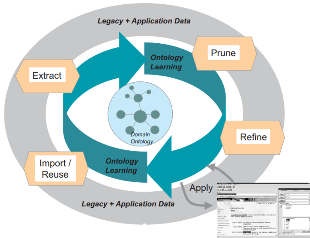
FIGURE 2.37: Ontology learning process steps (Maedche et al., 2001).
