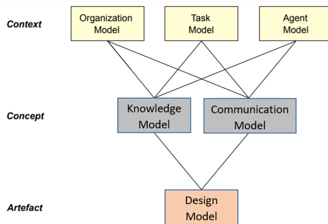
FIGURE 2.43: CommonKADS models (Schreiber et al., 2000).
