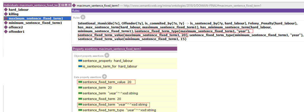
FIGURE 5.17: Inferring Article 547 using CrimOnto and SWRL in Protégé.
