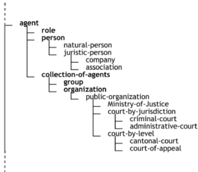
FIGURE 2.17: Concept anchoring in OCL.NL/LRI-Core (Breuker et al., 2002).
