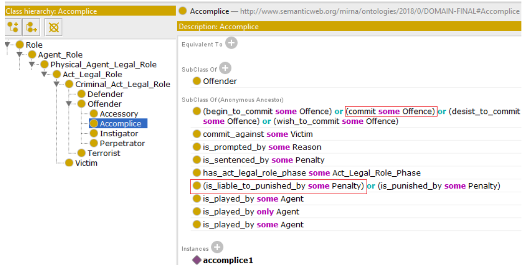
FIGURE 5.6: The class Accomplice in Protégé.
