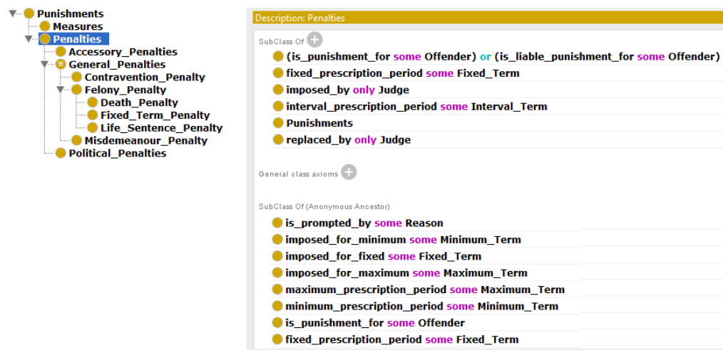
FIGURE 4.31: Penalty in Protégé.
