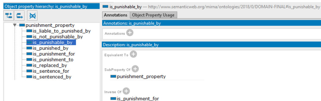
FIGURE 5.7: The object property is_punishable_by in Protégé.
