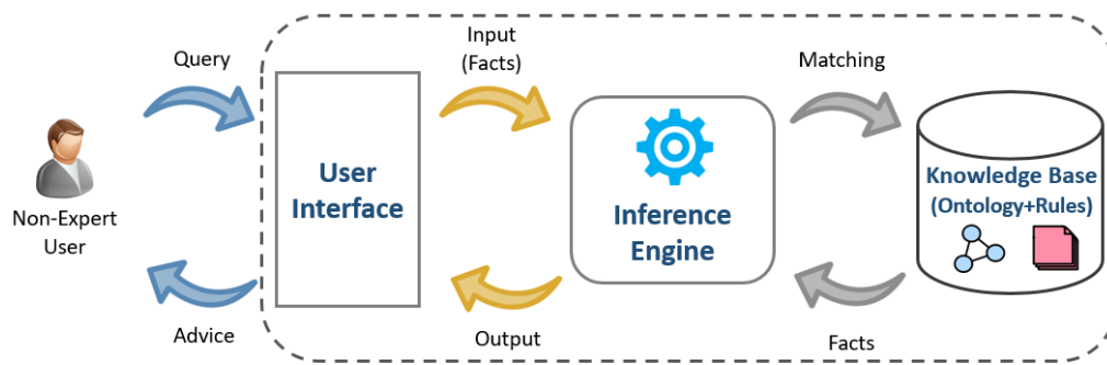
FIGURE 6.3: Reasoning Model of CORBS.
