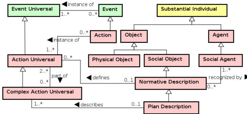
FIGURE 2.13: Agents, objects, and normative descriptions (Nardi et al., 2016).
