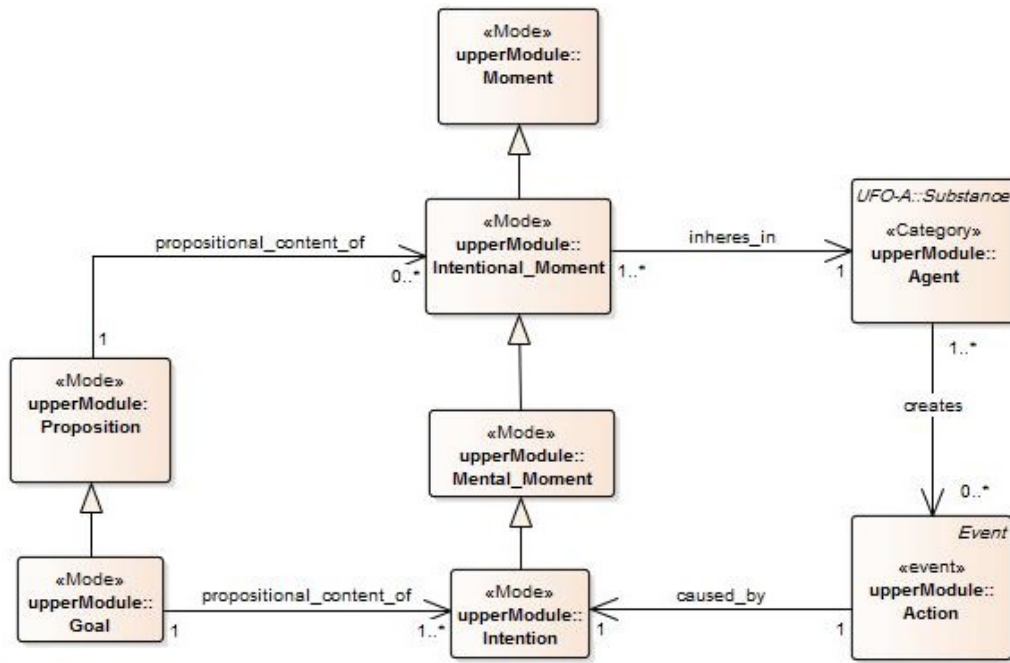
FIGURE 4.16: The concept Intention in OntoUML.
