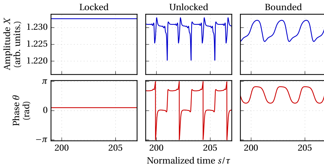
Figure III.22: Example of very different long-term phase and beatnote intensity behaviors obtained by choosing different feedback phases. In the three cases \delta = 0.002 , \kappa_0 = 0.01 , m = 0.8 . Locked: \varphi_{1,2,x} = 0, 0, 0 . Unlocked \varphi_{1,2,x} = 0, -1.3, 2 . Bounded phase \varphi_{1,2,x} = -2, -2.16, 1 (all phases in radians).
