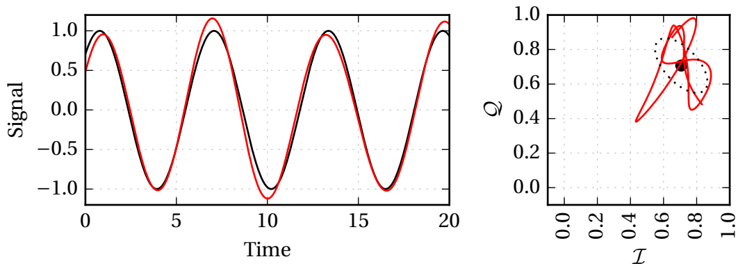
Figure I.6: Sinusoidal signal x(t) with phase and amplitude noise.
