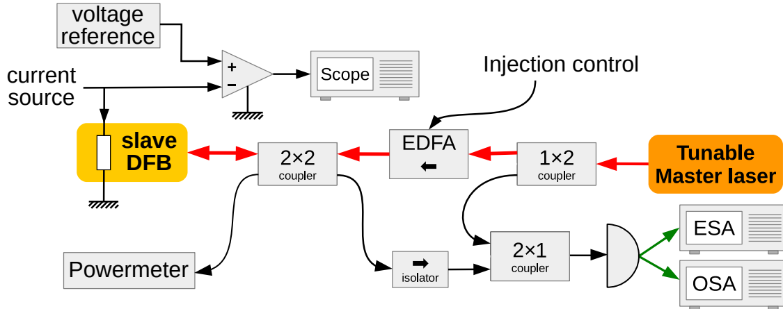
Figure III.13: Experimental setup used for measuring the linewidth enhancement factor.
