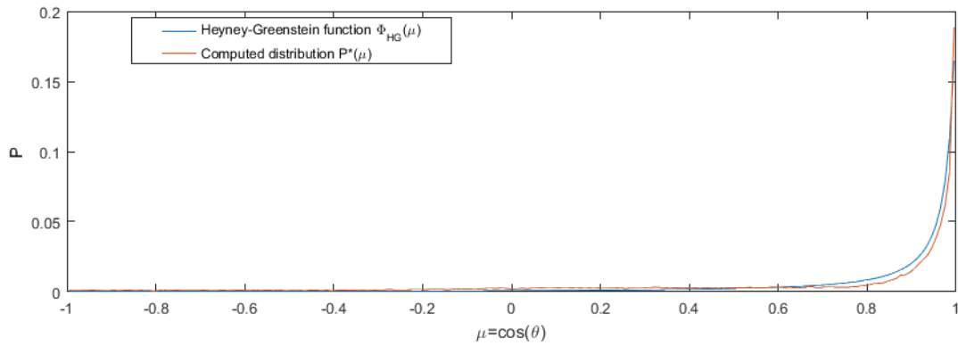
Fig. 6.8 – Comparison of numerically calculated distribution P^* and respective Henyey-Greenstein function \Phi_{HG} for a high-porosity open cell foam ( \epsilon=0.89 )
