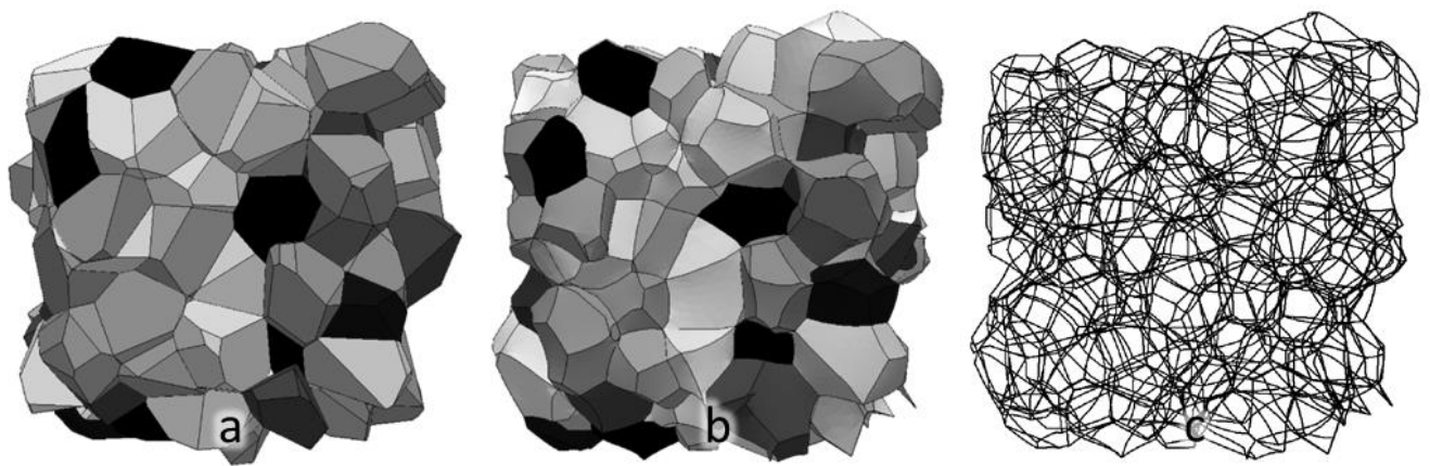
Fig. 4.2 – (a) Initial cell structure (Voronoi diagram) (b) Processed cell structure (after Surface Evolver) (c) Cell structure skeleton.
