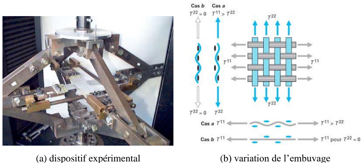
Figure 1.16 La traction biaxiale des tissés [BUE 98, BUE 01]
