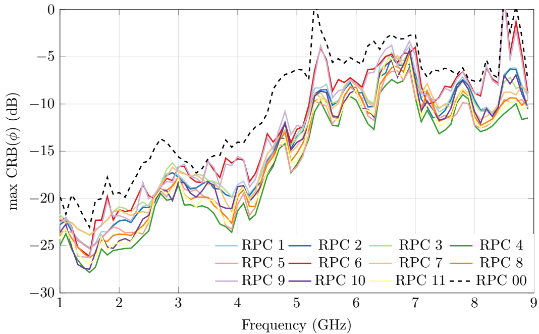
Figure H.8: Highest simulated \text{CRLB}(\phi) of the Four Season VA using different RPCs [1 to 11] added to the RPC 00, and under the scenario conditions defined in Table 3.15 ( \gamma = 67.5^\circ \dagger \eta = 0^\circ )
