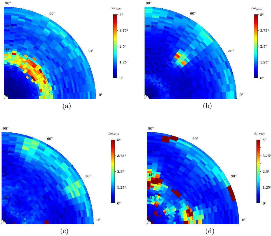
Figure 3.19: Simulated \Delta a_{RMS}(\phi, \theta) obtained with the improved version of Two Season VA from using RPC 0 only, and under the scenario conditions defined in Table 2.3 at the following frequencies: (a) 1.4 GHz, (b) 2.2 GHz, (c) 3.0 GHz, and (d) 3.8 GHz. Elevation angles \theta are given on the radial axis and azimuth angles \phi are given on the angular axis.
