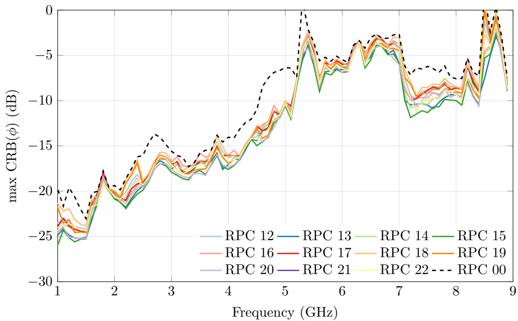
Figure H.9: Highest simulated \text{CRLB}(\phi) of the Four Season VA using different RPCs [12 to 22] added to the RPC 00, and under the scenario conditions defined in Table 3.15 ( \gamma = 67.5^\circ \dagger \eta = 0^\circ )
